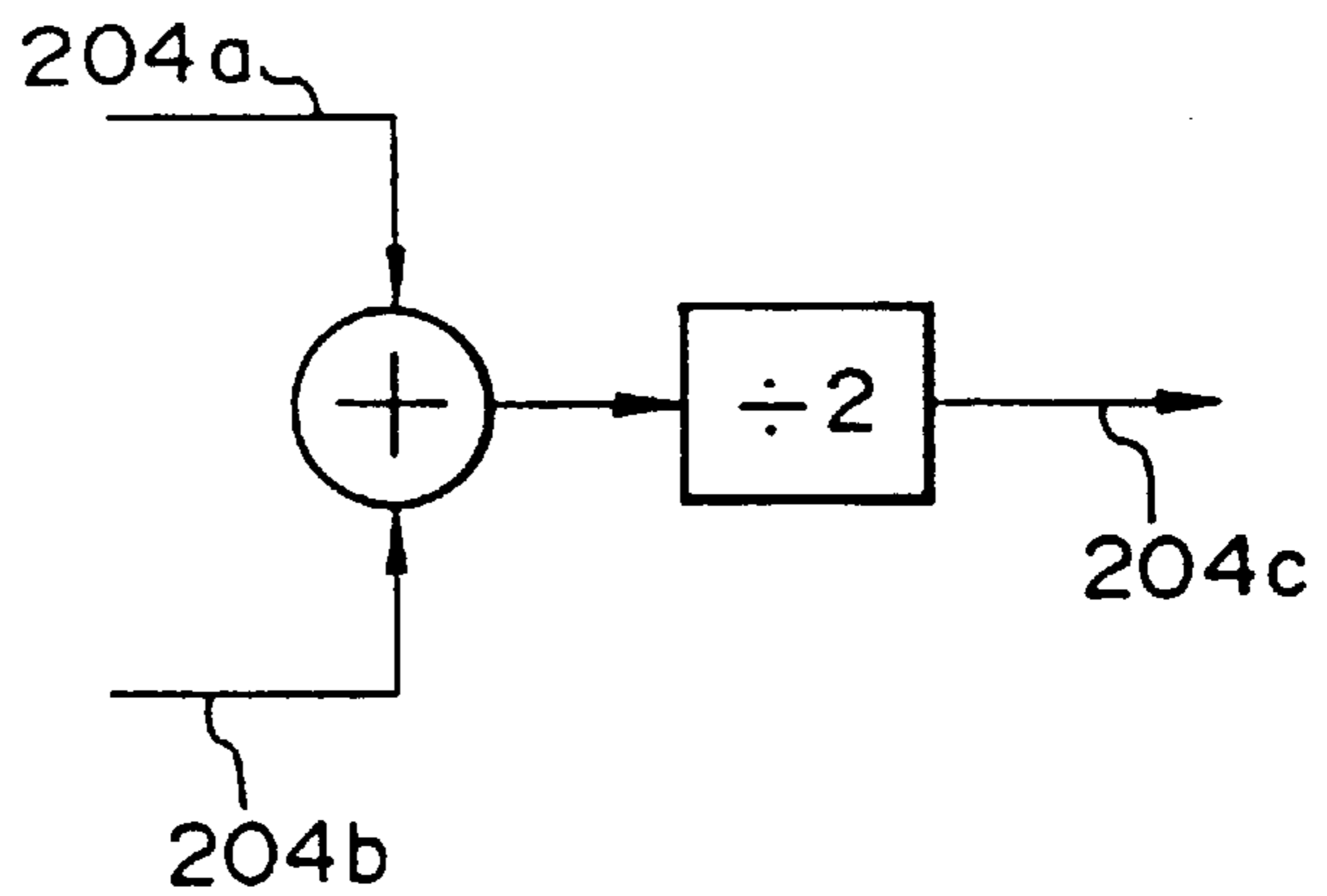
INTERPOLATION SECTION
