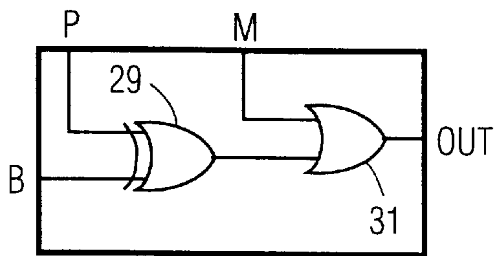
CELL TYPE 2 PROGRAMMABLE INVERTER WITH MASK
