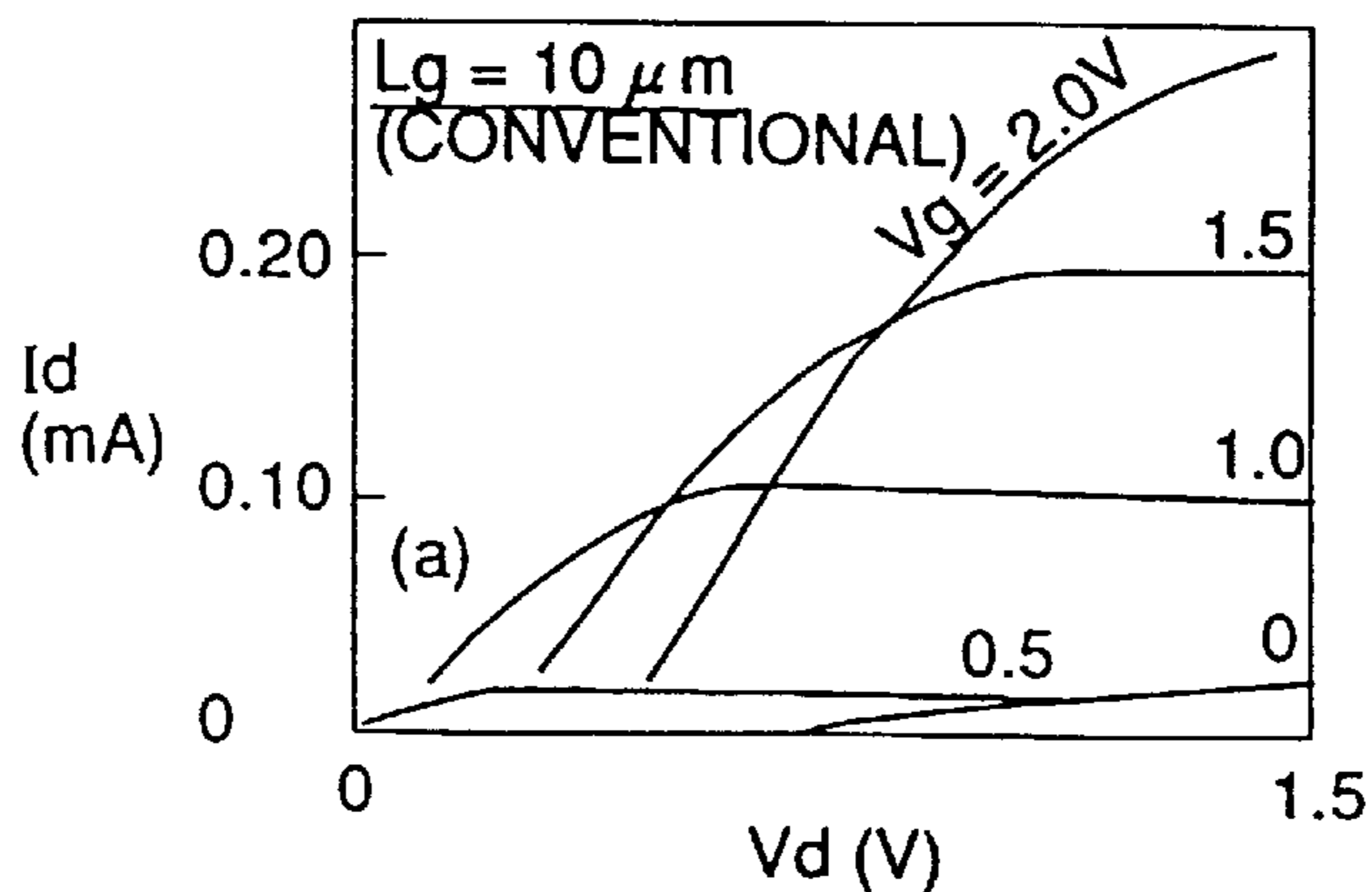
DEPENDANVE OF I_d/V_d UPON GATE VOLTAGE V_g
