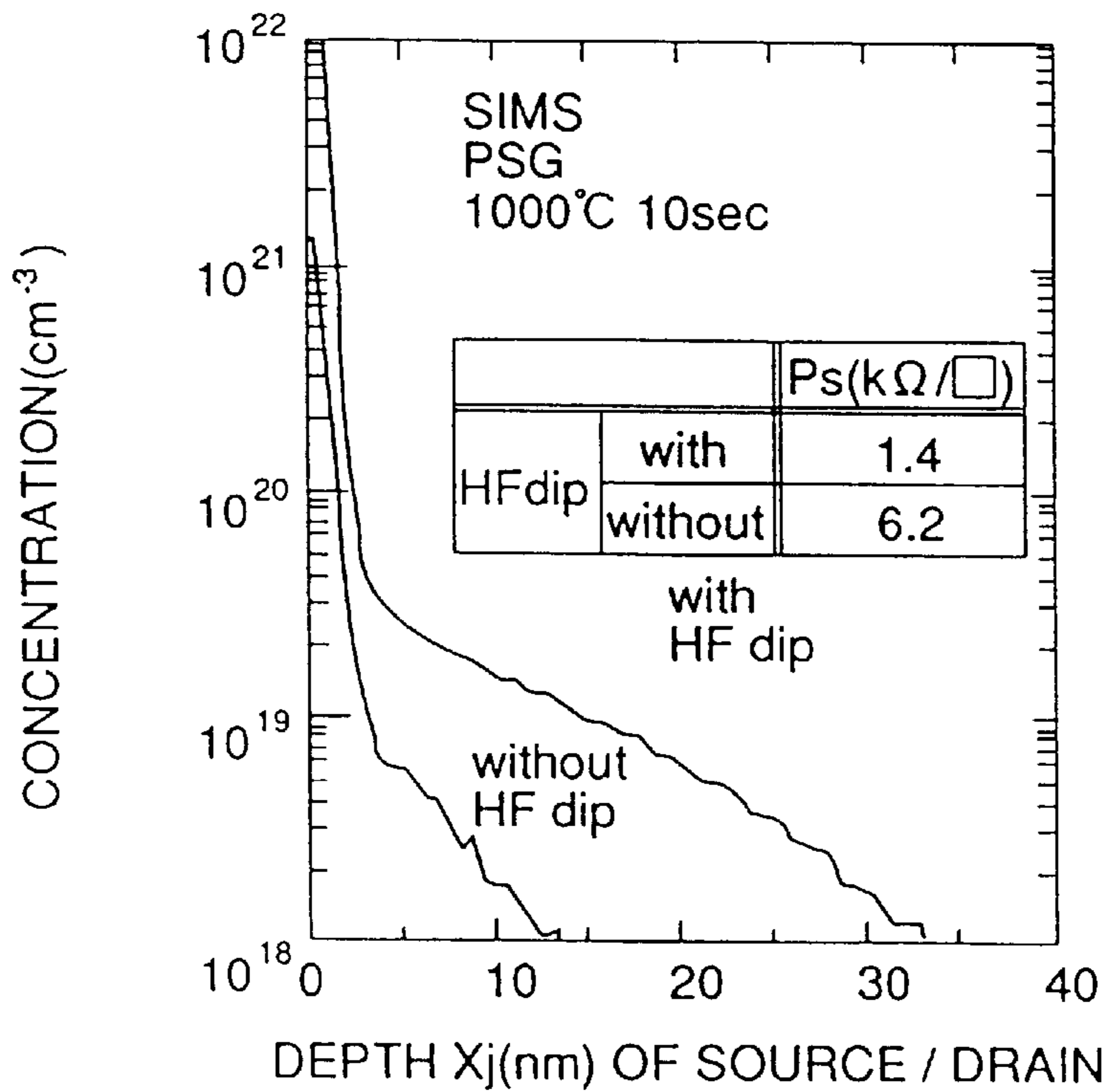
CONCENTRATION PROFILE TO DIFFUSION DEPTH AT SOURCE / DRAIN REGION
