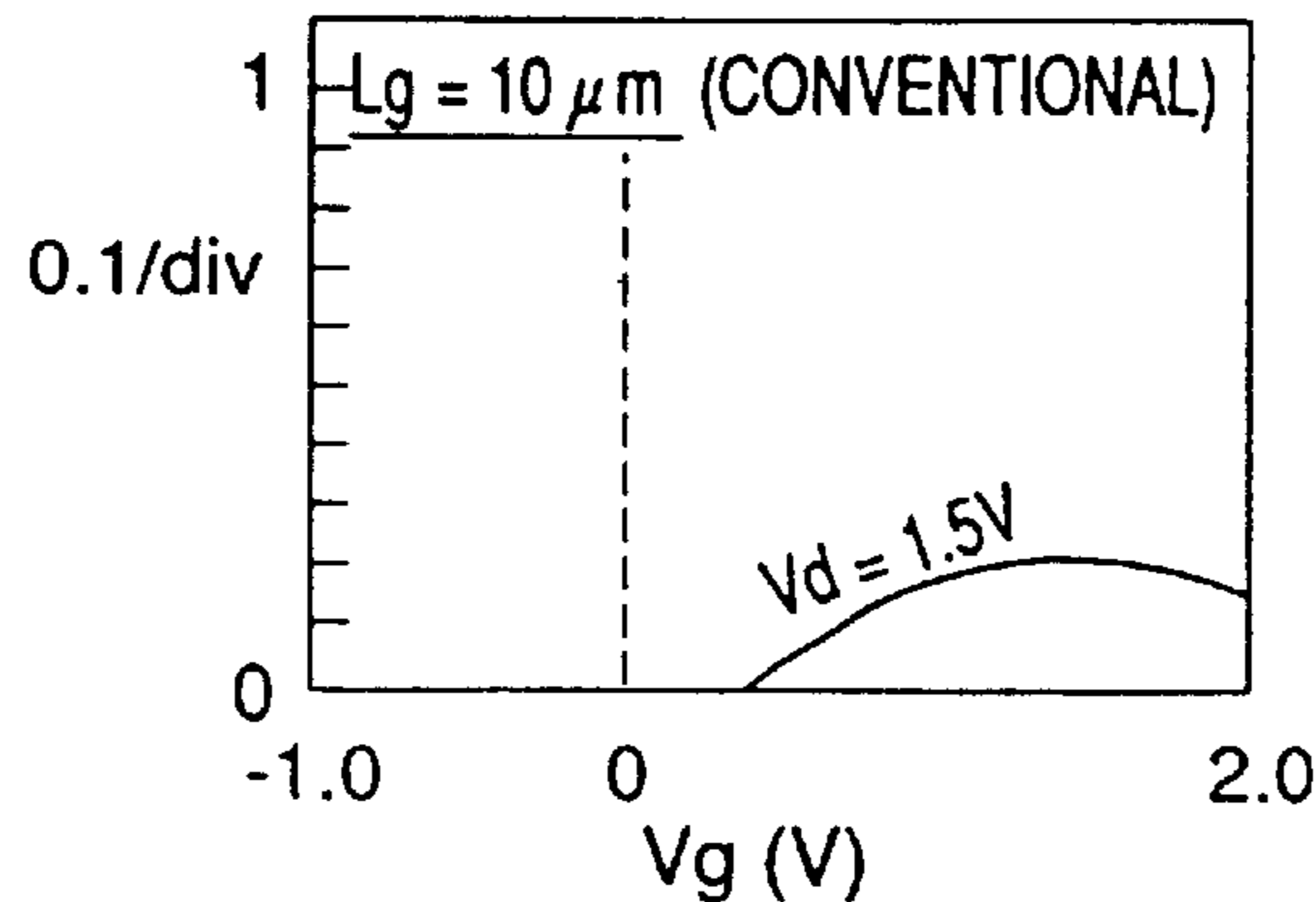
DEPENDANCE OF TRANSCONDUCTANCE gm UPON GATE VOLTAGE
