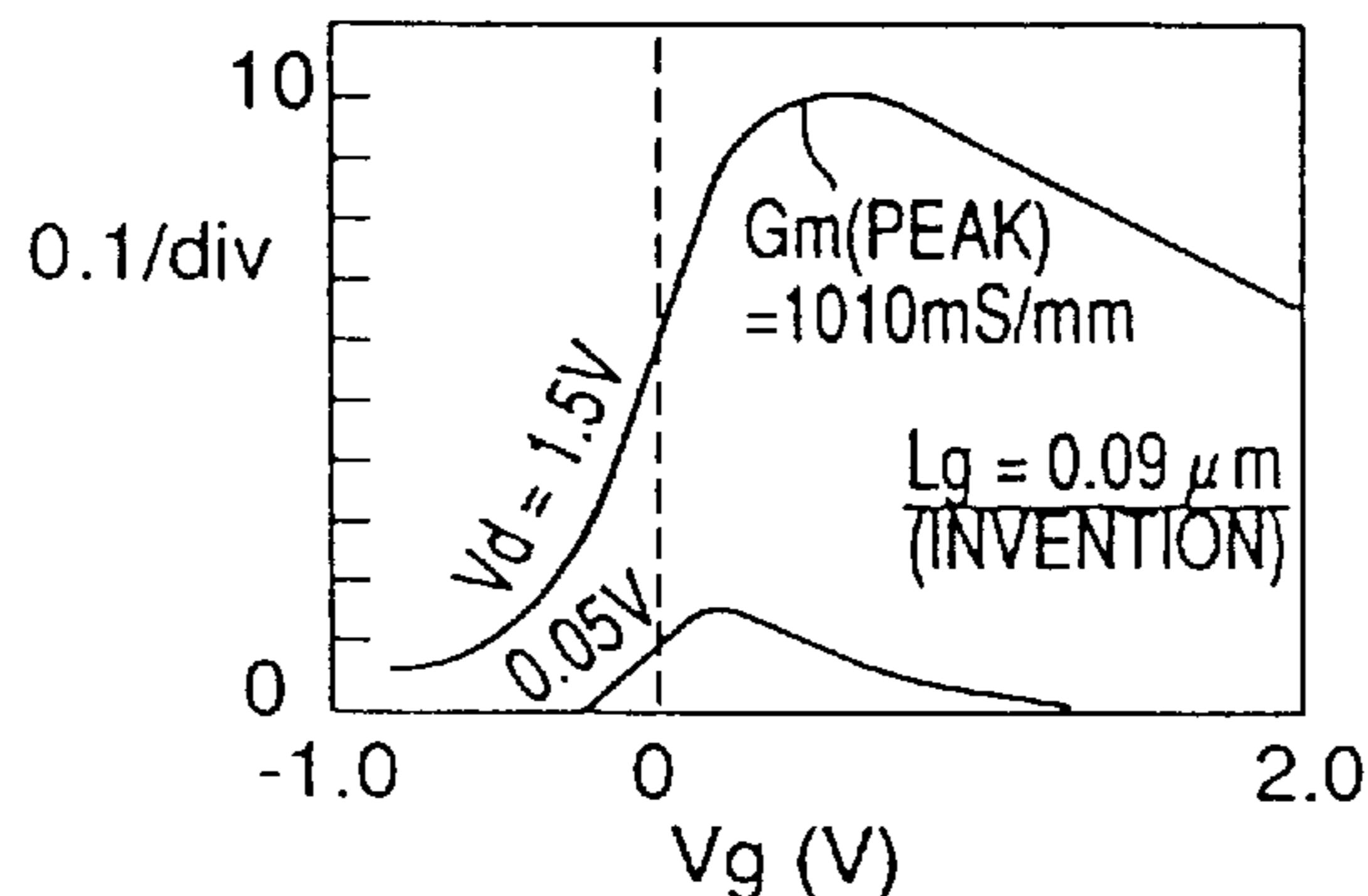
DEPENDANCE OF TRANSCONDUCTANCE gm UPON GATE VOLTAGE
