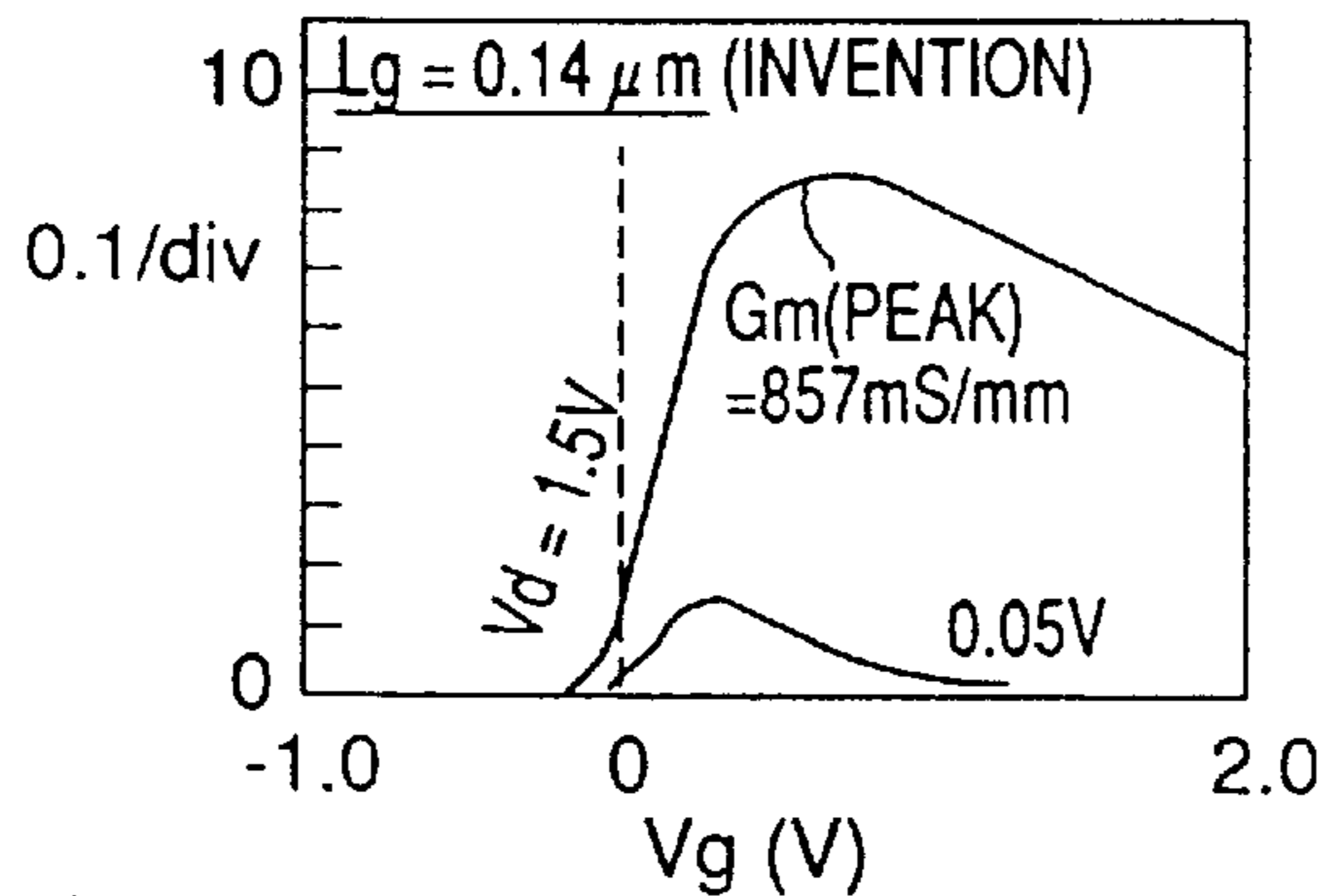
DEPENDANCE OF TRANSCONDUCTANCE gm UPON GATE VOLTAGE
