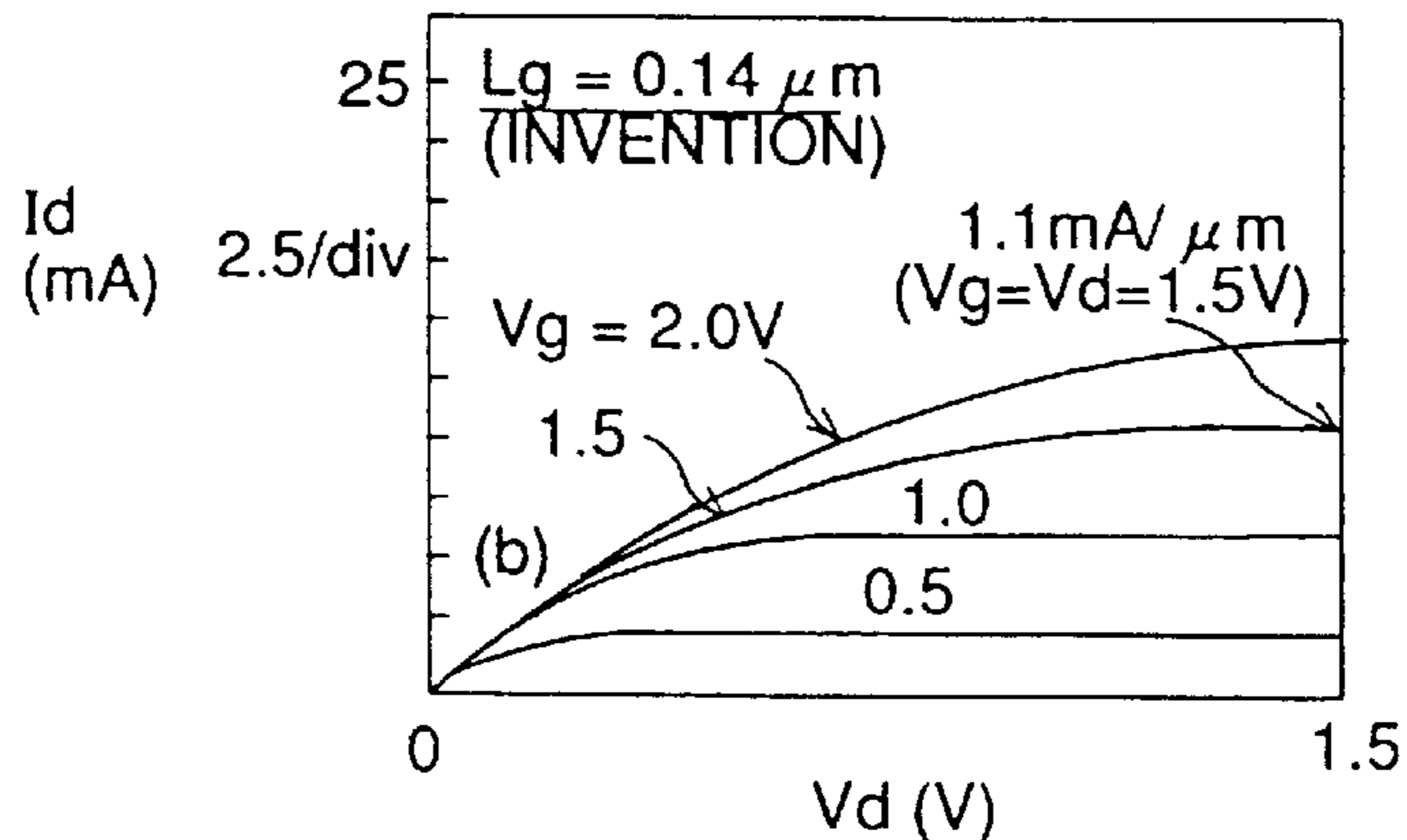
DEPENDANVE OF I_d/V_d UPON GATE VOLTAGE V_g
