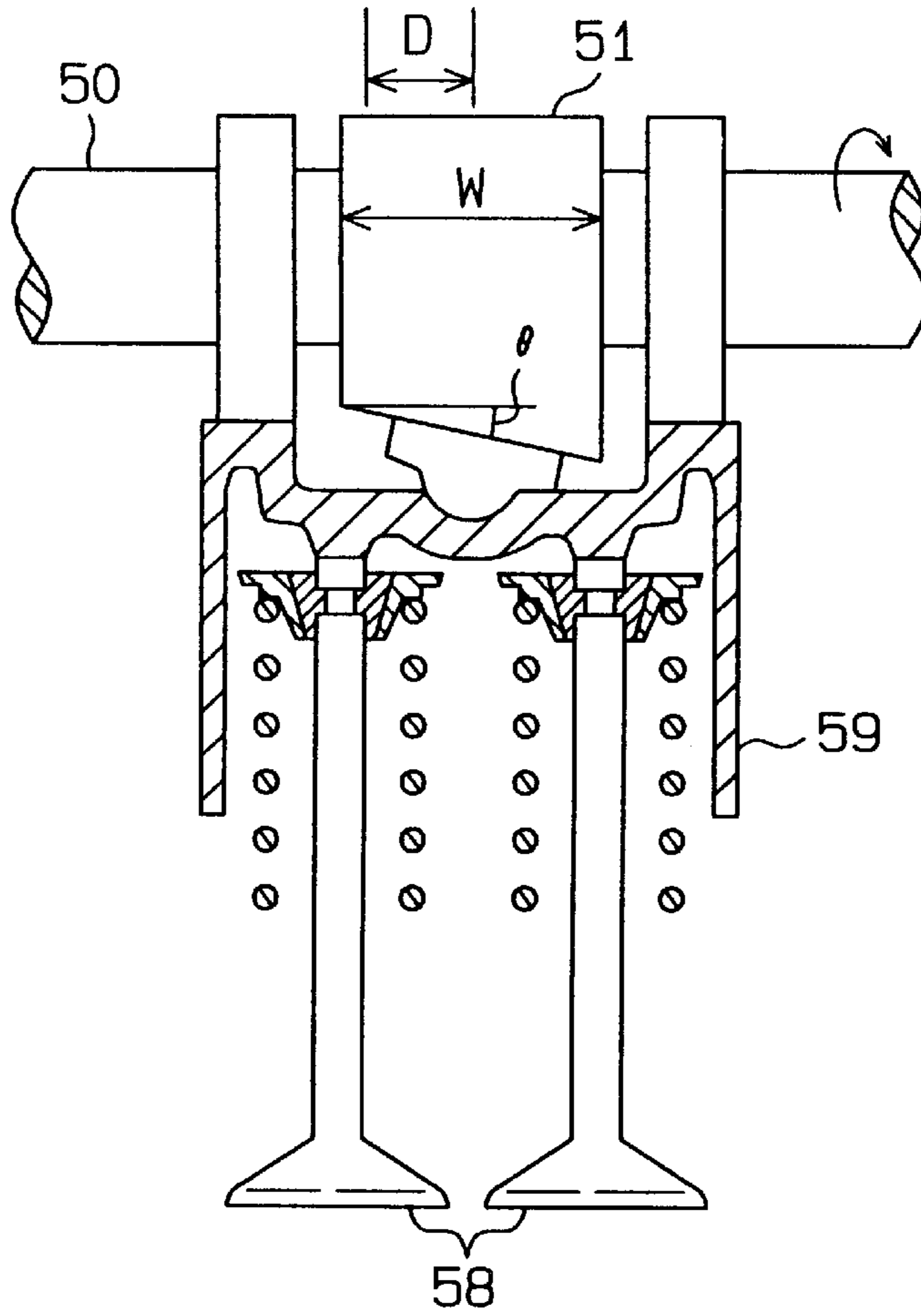
Fig. 14 (Prior Art)
