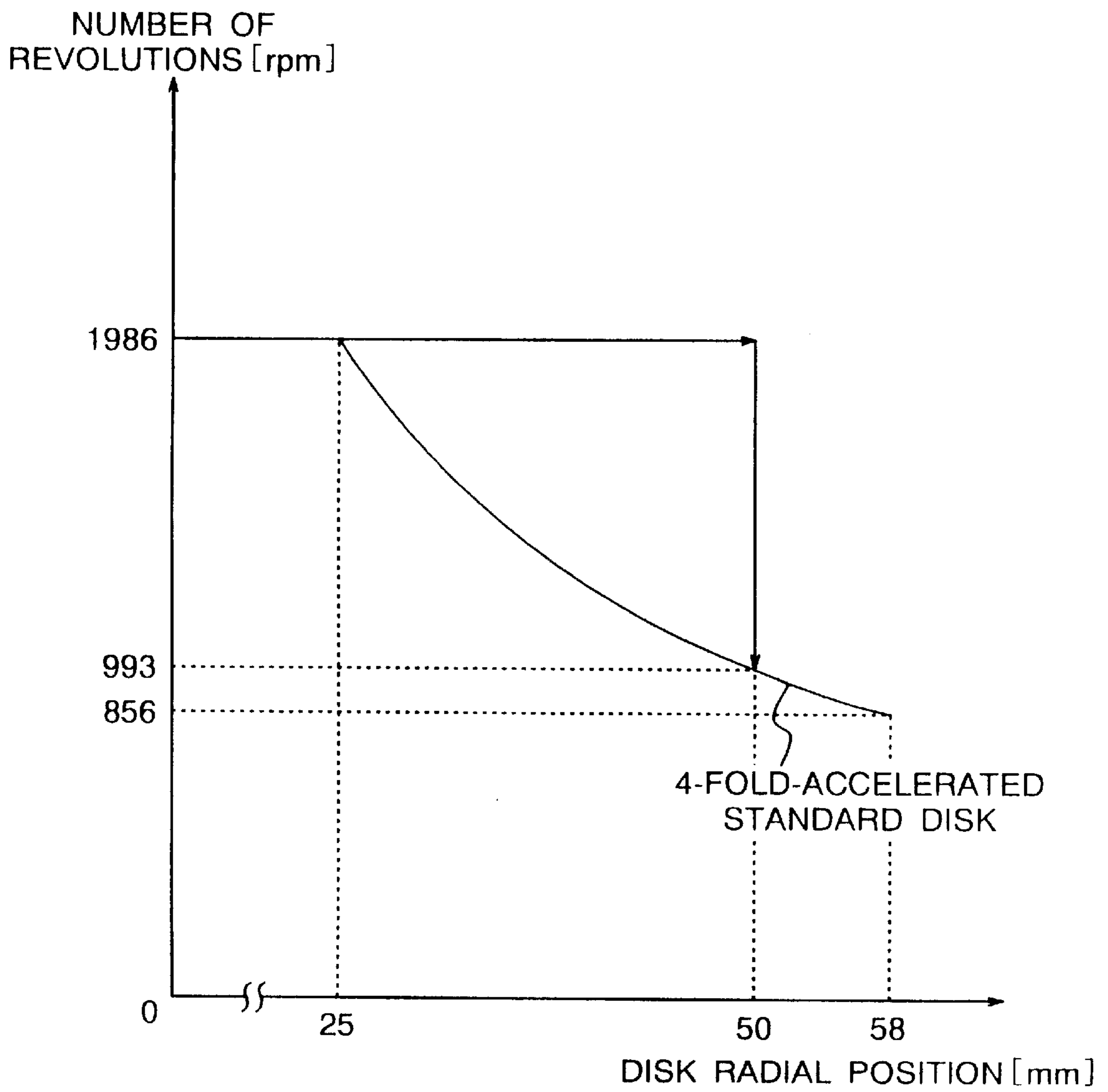
FIG. 19 PRIOR ART
