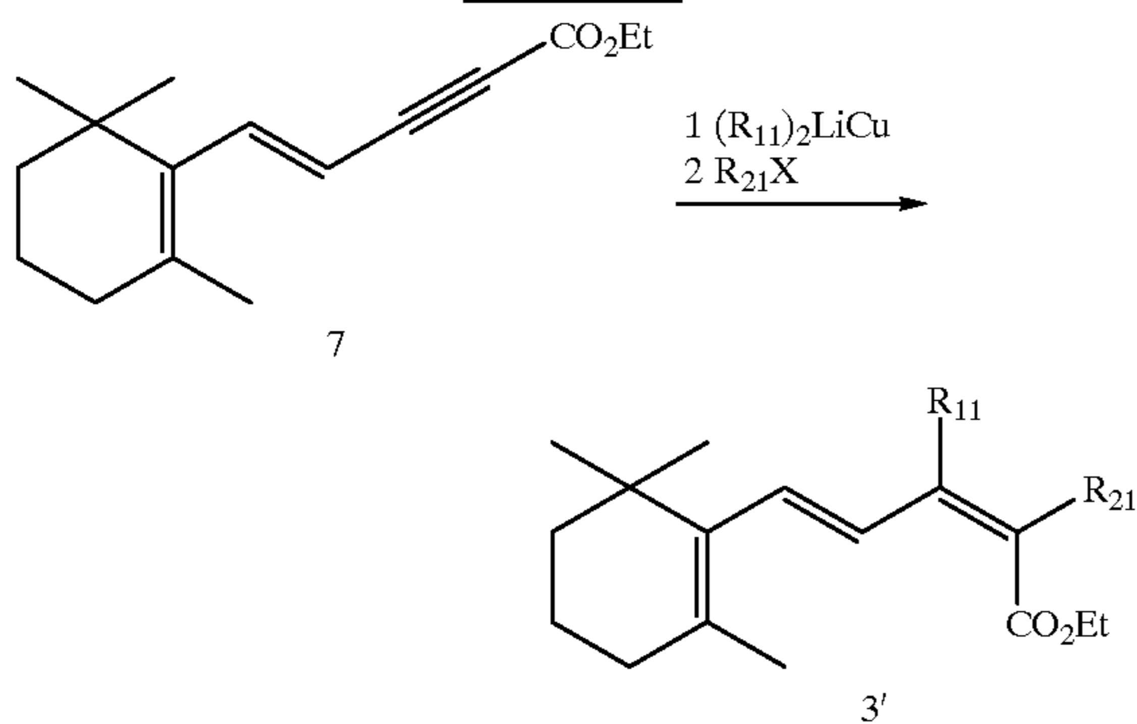
SCHEME 1b
