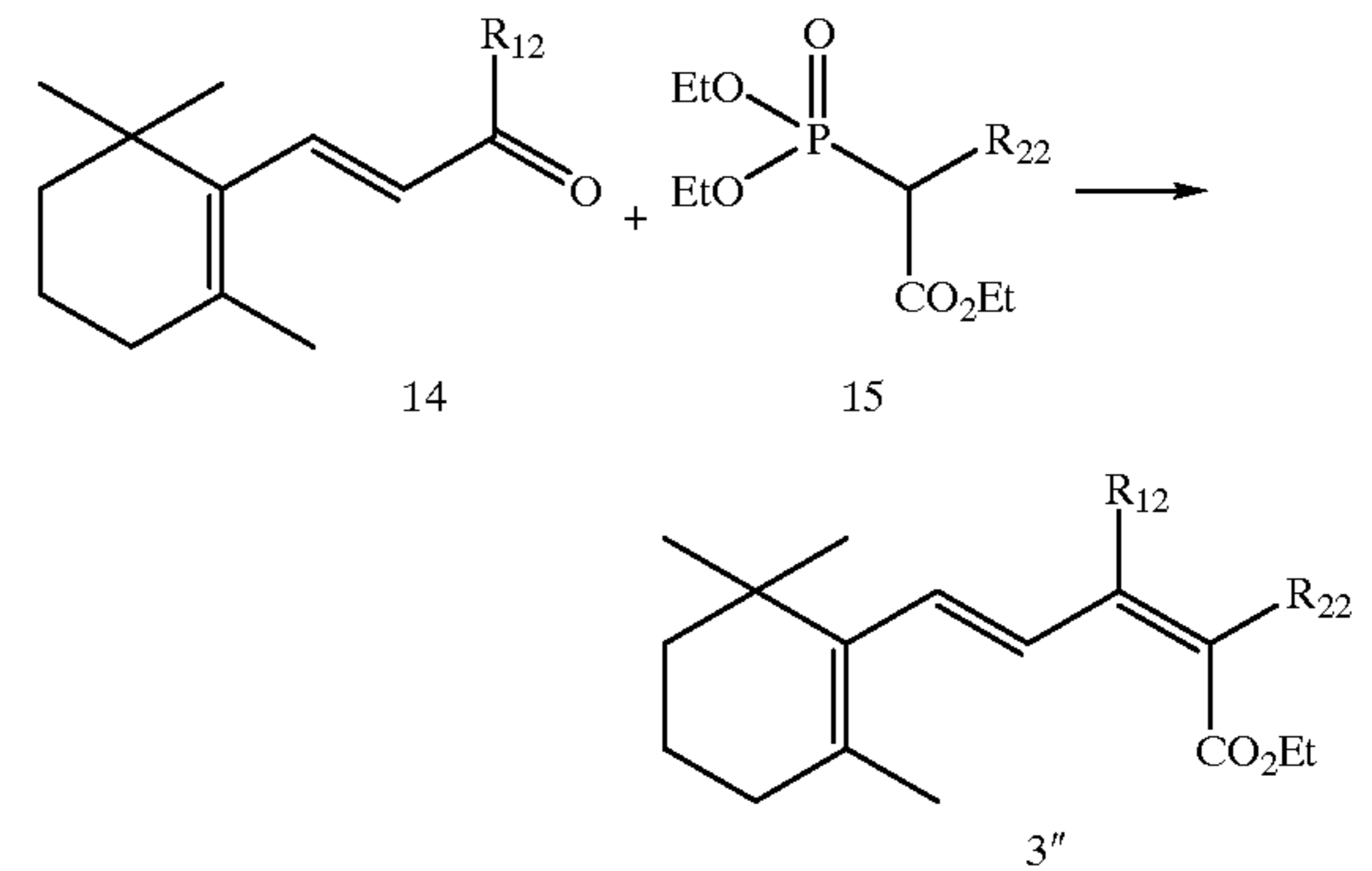
SCHEME 1c
