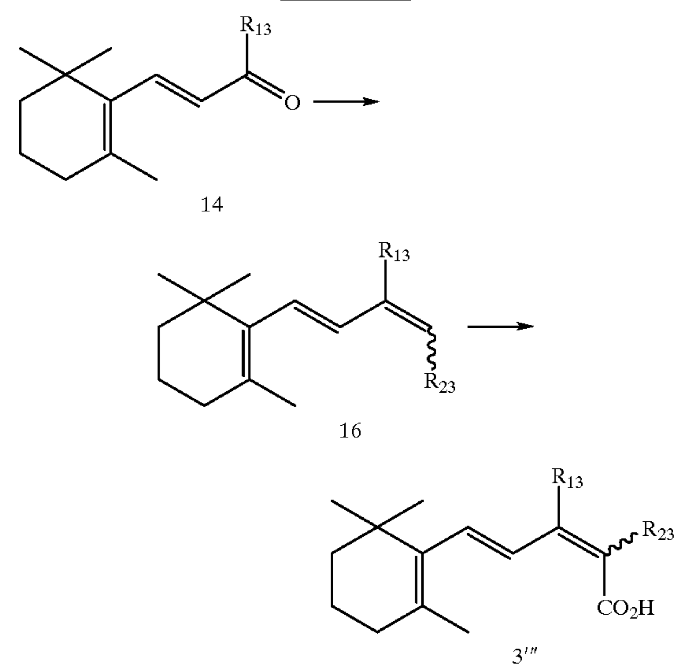
SCHEME 1d
