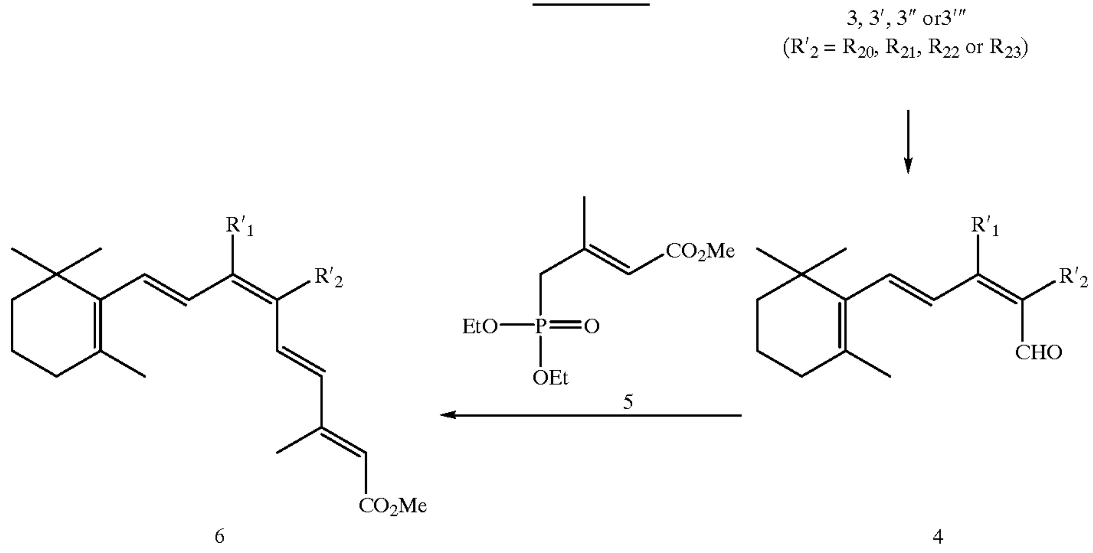
SCHEME 2
