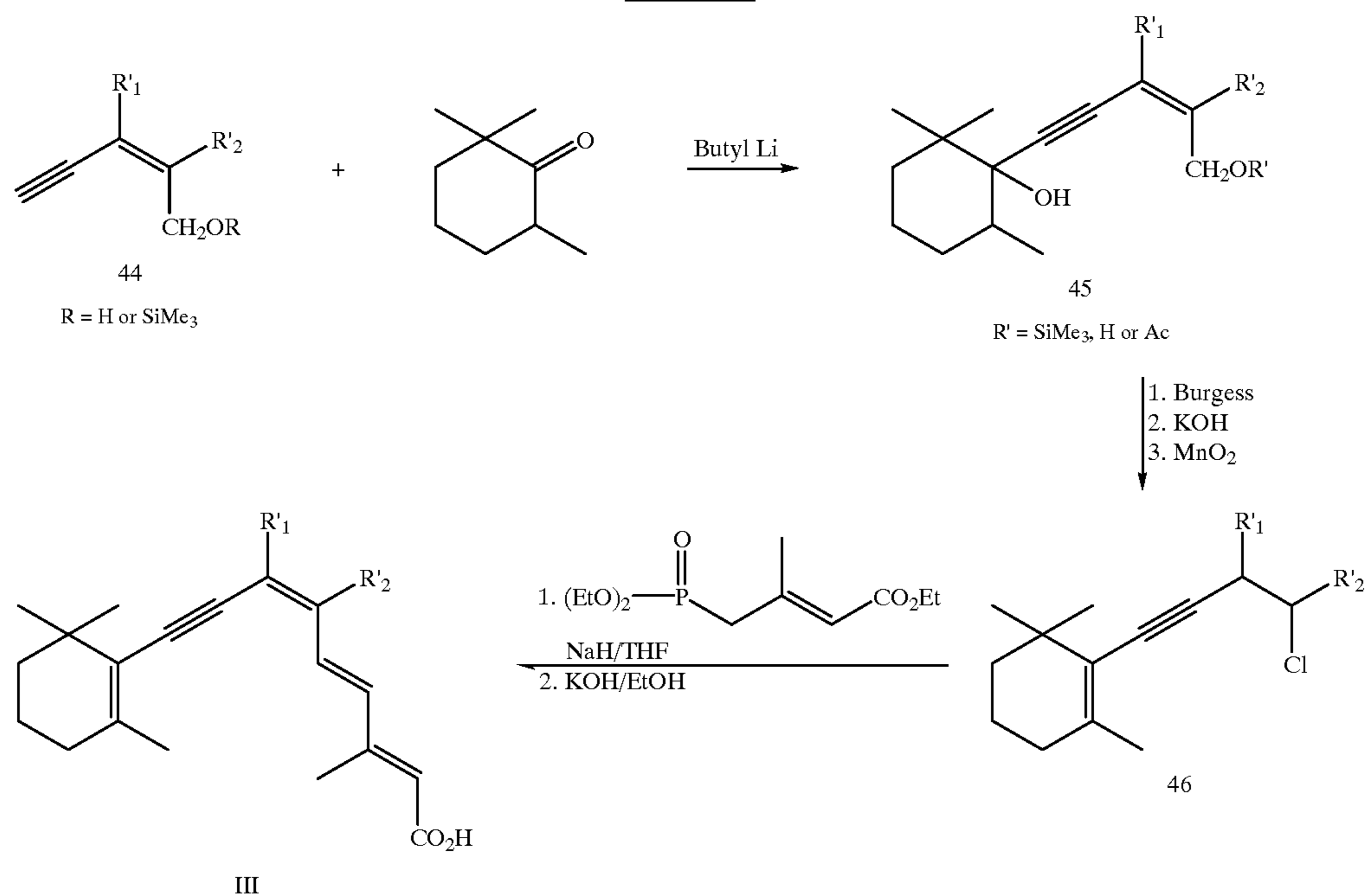
SCHEME 9
