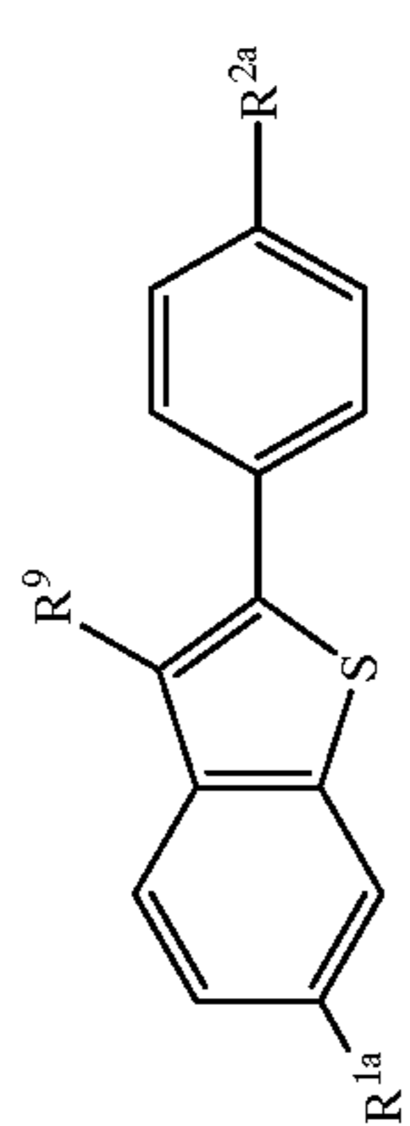
Scheme V
