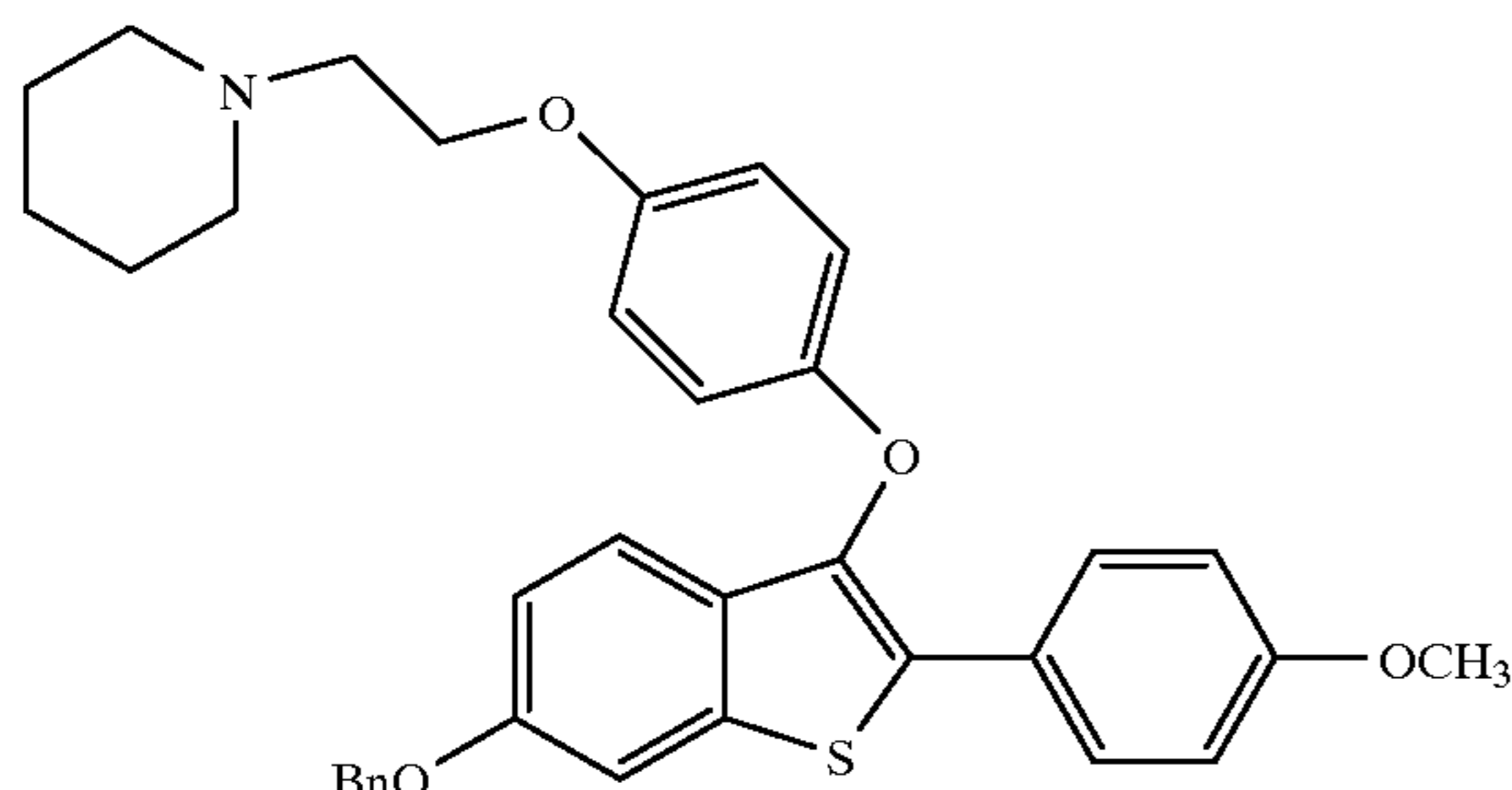
[6-Benzyloxy-3-[4-[2-(1-piperidiny)ethoxy]phenoxy]-2-(4-methoxyphenyl)]benzo[b]thiophene
