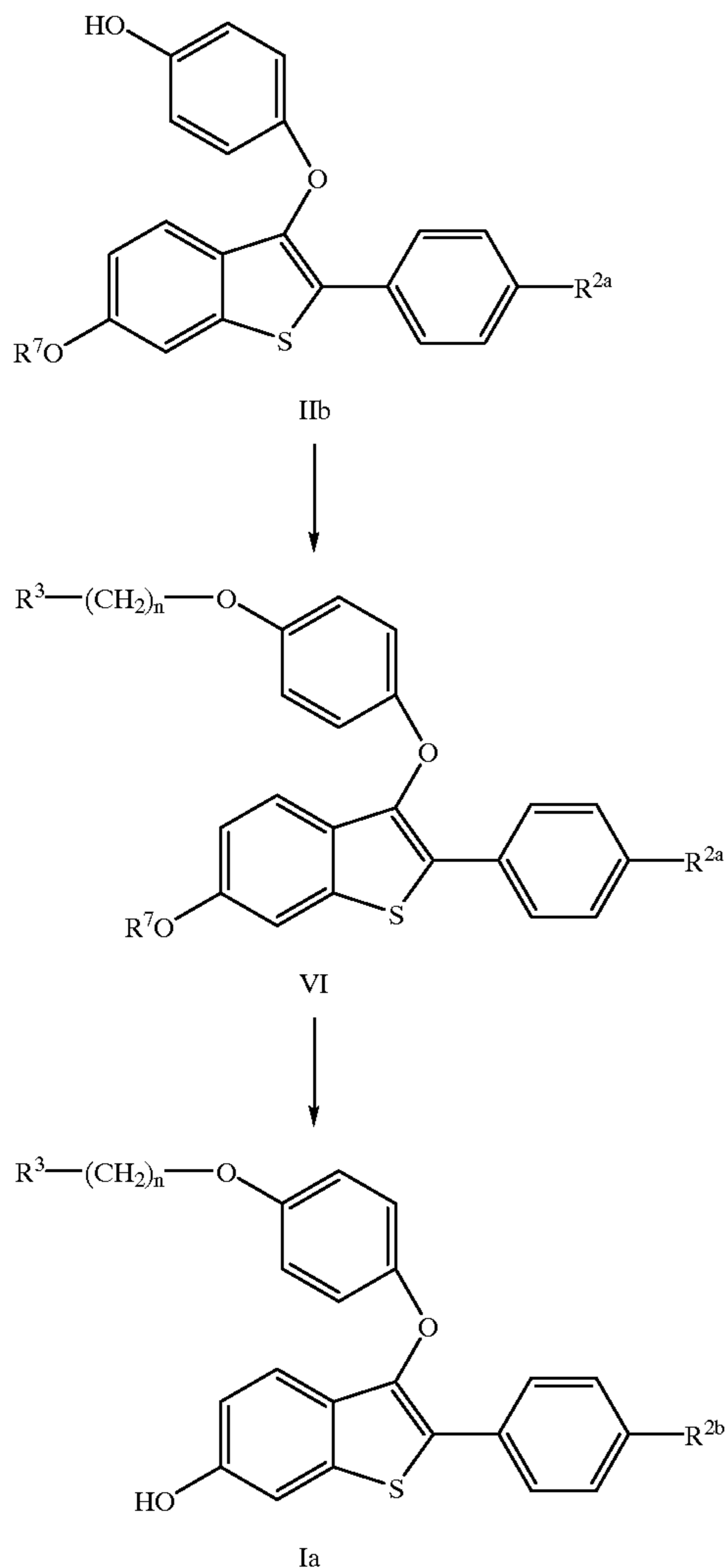
Scheme II
