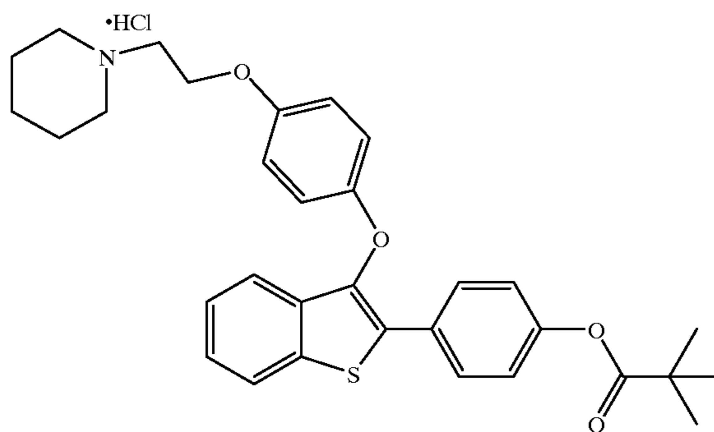
3-[4-[2-(1-piperidinyl)ethoxy]phenoxy]-2-(4-pivaloyloxyphenyl)benzo[b]thiophene Hydrochloride
