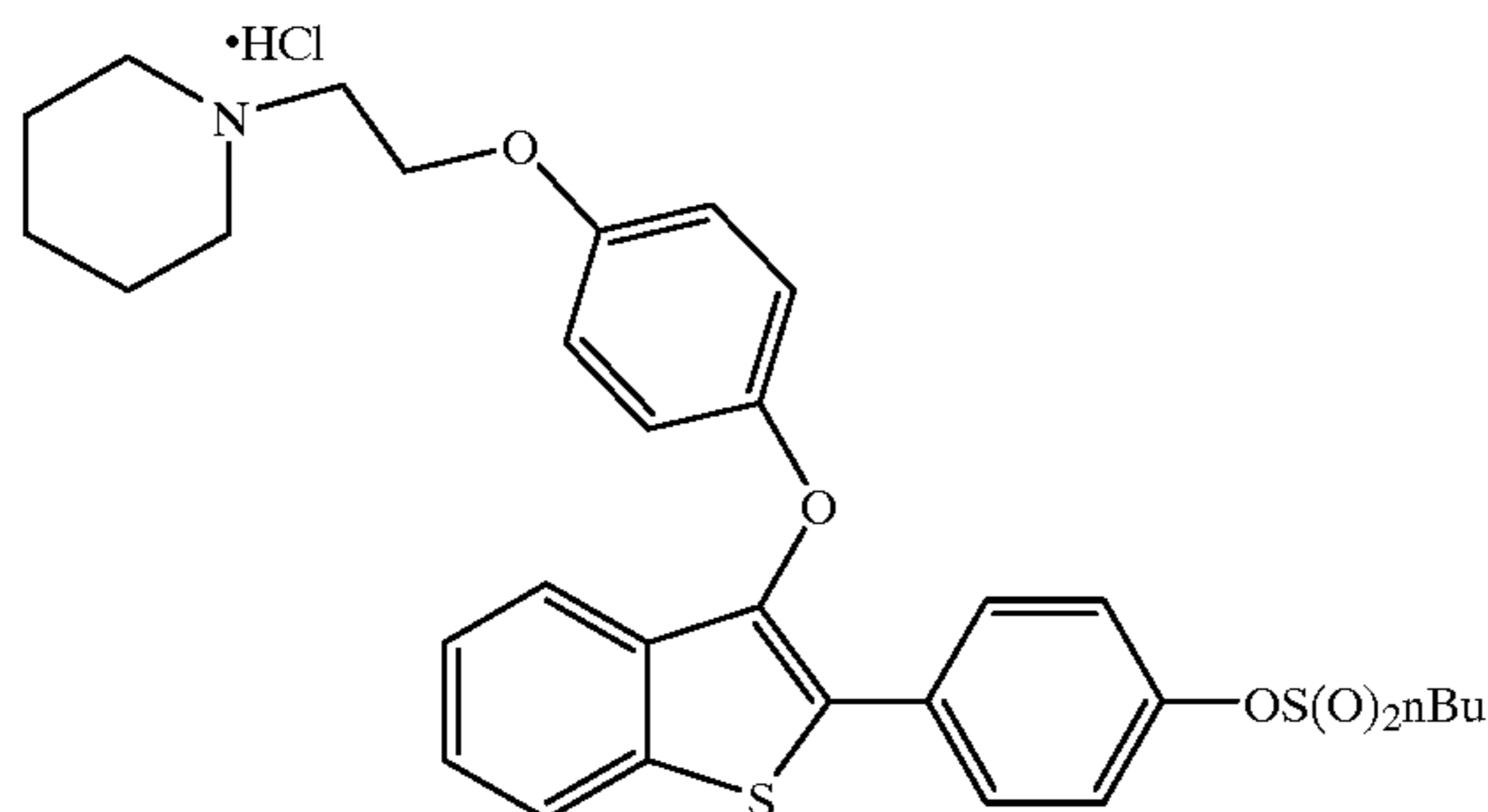
3-[4-[2-(1-piperidinyl)ethoxy]phenoxy]-2-(4-butylsulfonyl-oxyphenyl)benzo[b]thiophene Hydrochloride
