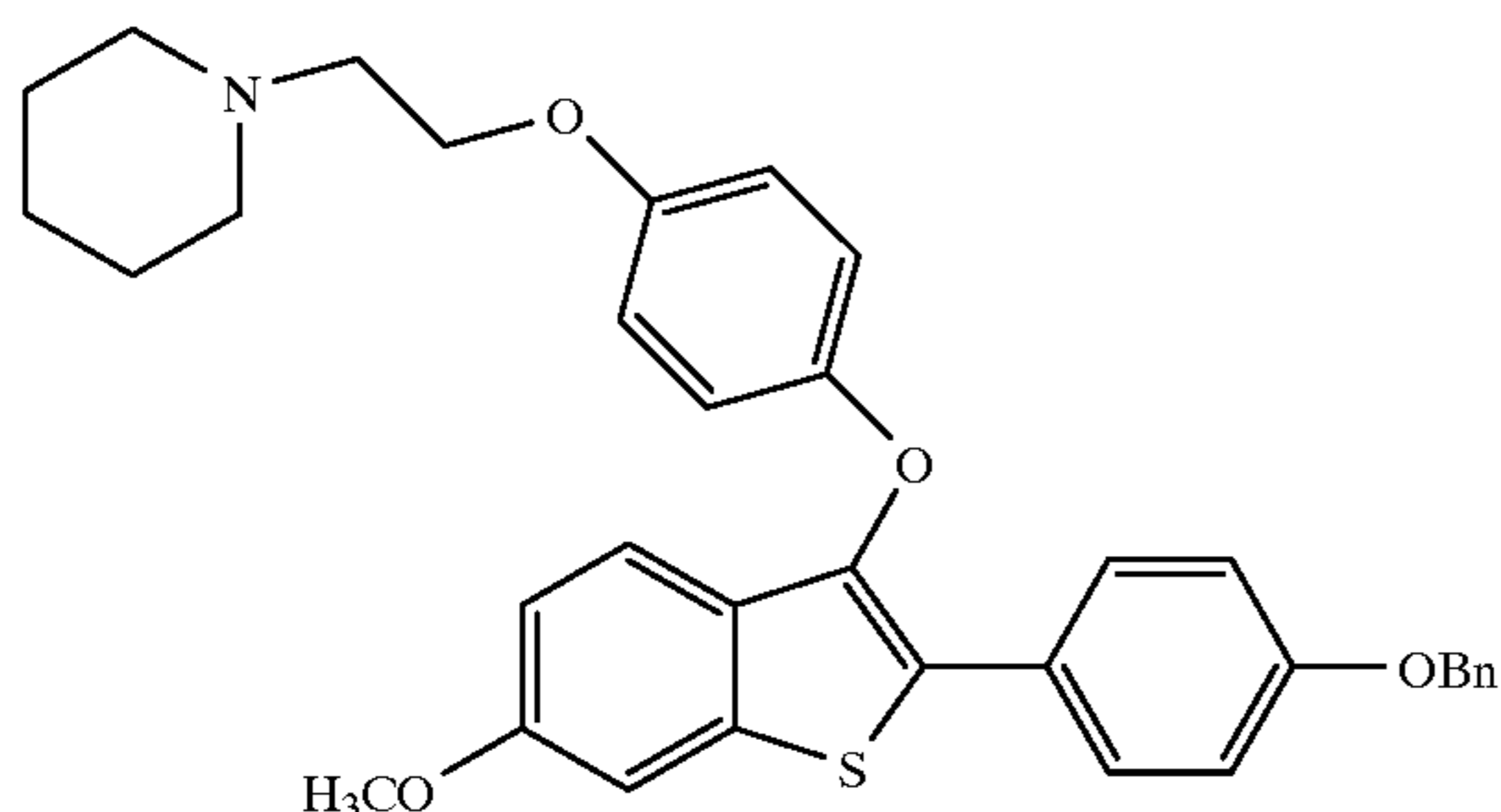
[6-Methoxy-3-[4-[2-(1-piperidiny)ethoxy]phenoxy]-2-(4-benzyloxyphenyl)]benzo[b]thiophene
