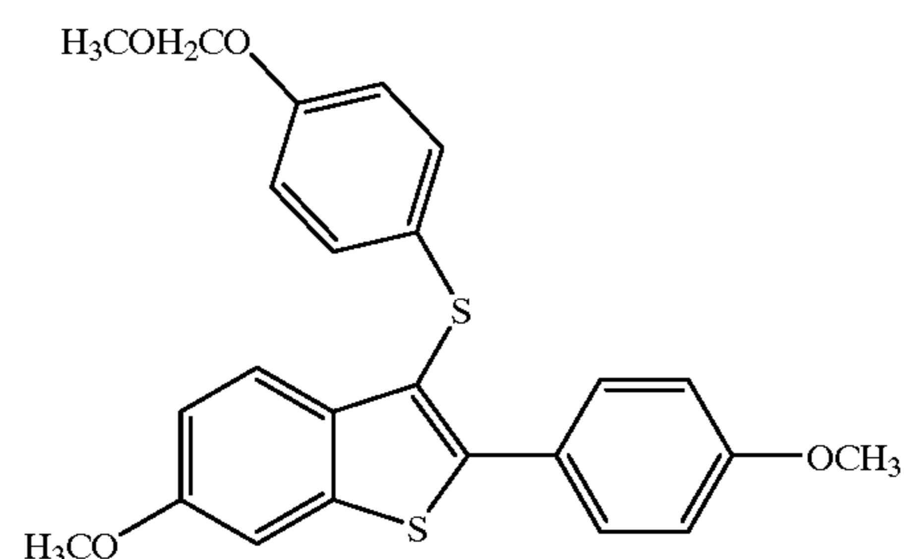
[6-Methoxy-2-(4-methoxyphenyl)-3-(4-methoxymethyleneoxy)thiophenoxy]benzo[b]thiophene
