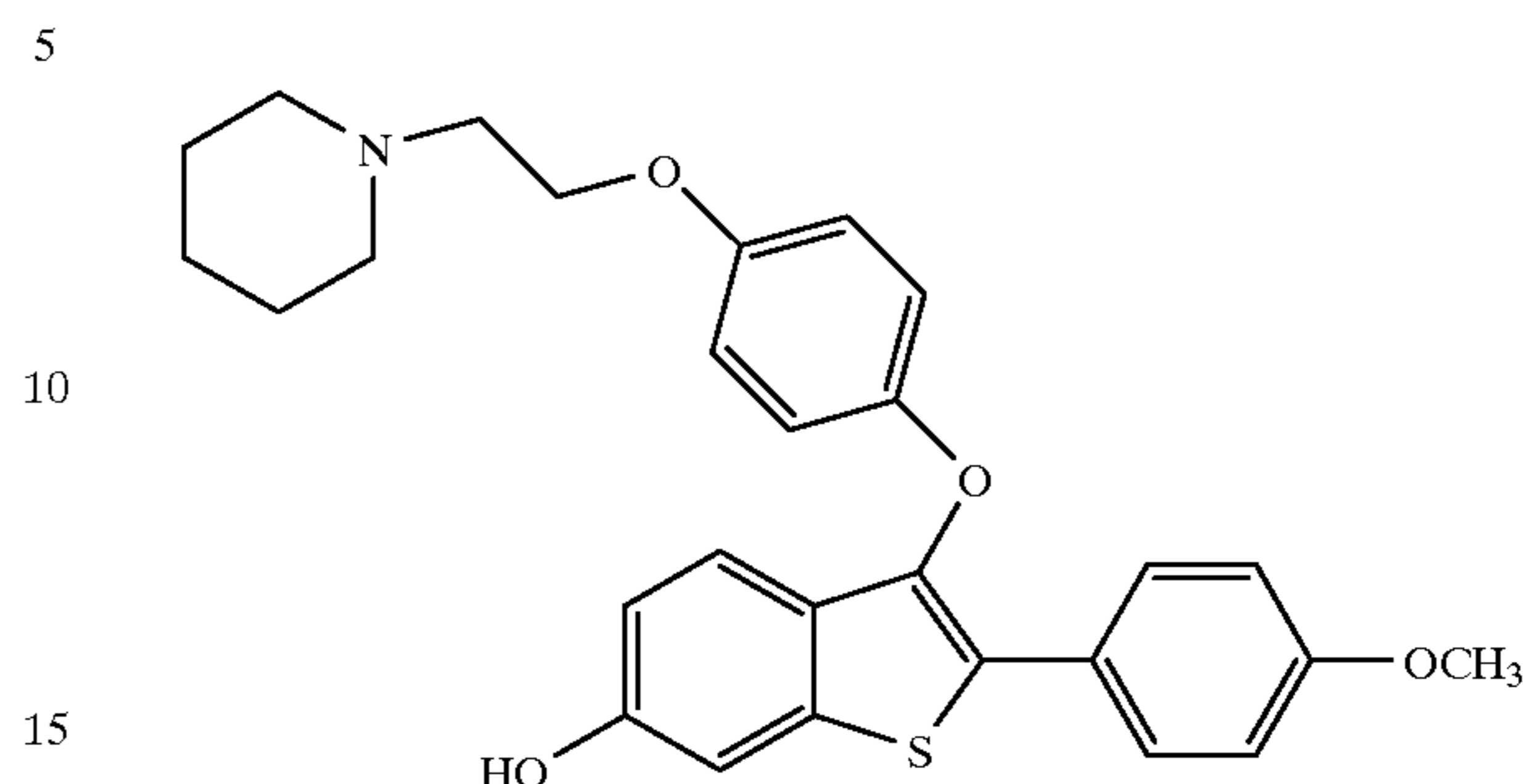
[6-Hydroxy-3-[4-[2-(1-piperidiny)ethoxy]phenoxy]-2-(4-methoxyphenyl)]benzo[b]thiophene
