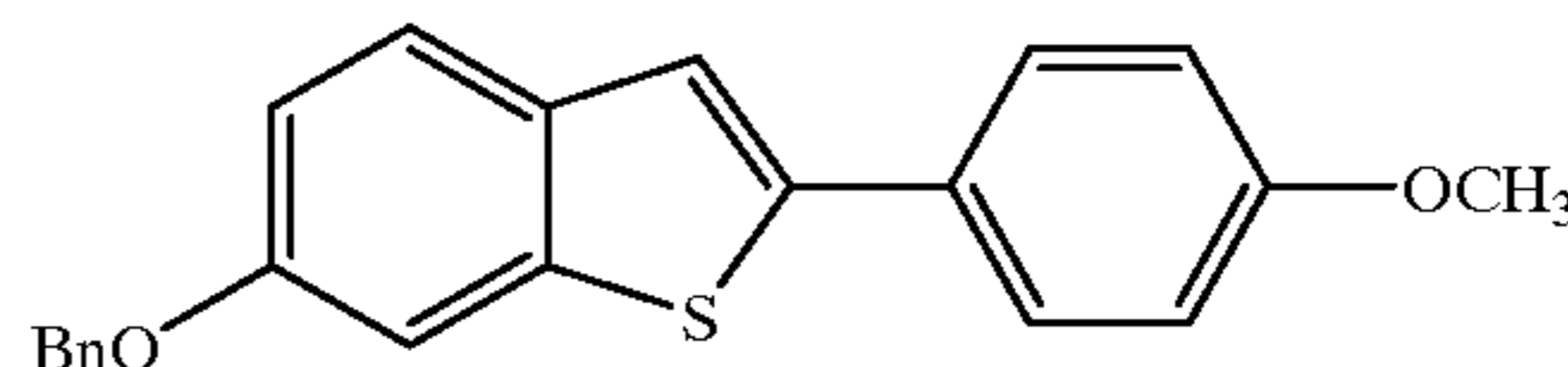
[6-Benzyloxy-2-(4-methoxyphenyl)]benzo[b]thiophene
