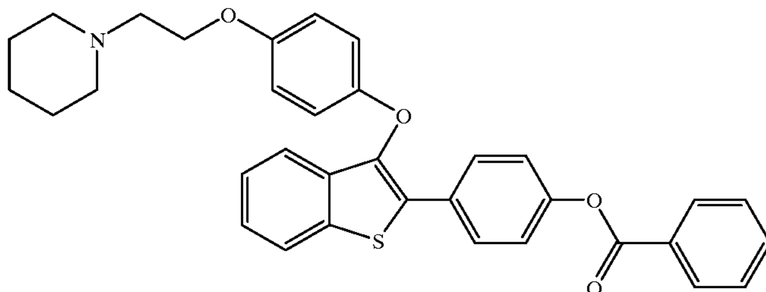
3-[4-[2-(1-piperidinyloxy)phenoxy]-2-(4-benzoyloxyphenyl)]benzo[b]thiophene hydrochloride •HCl
