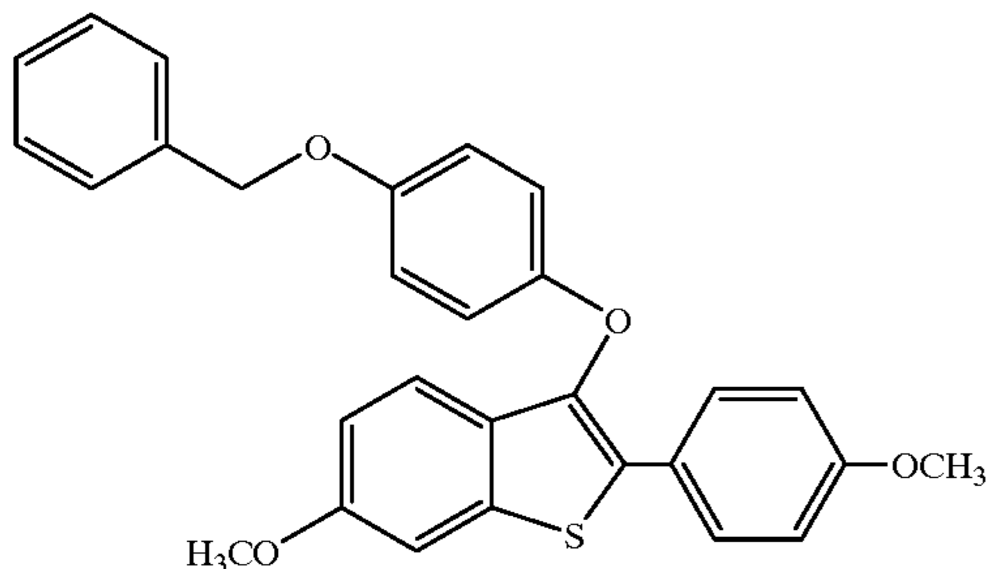
[6-methoxy-2-(4-methoxyphenyl)-3-(4-benzyloxy)phenoxy]-benzo[b]thiophene
