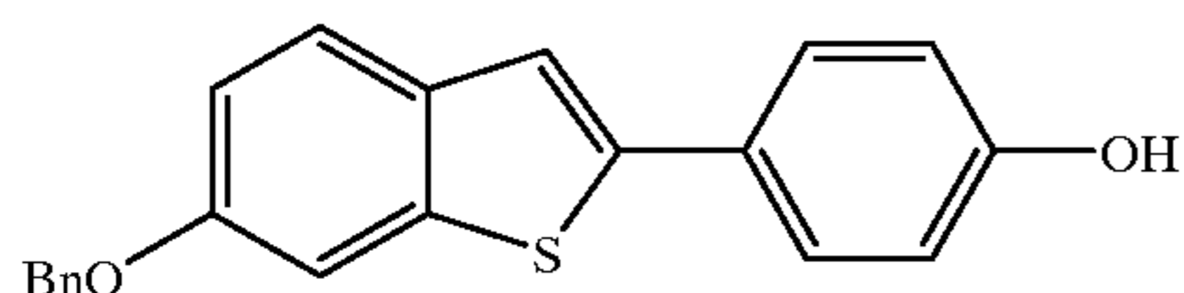
[6-Benzyloxy-2-(4-hydroxyphenyl)]benzo[b]thiophene
