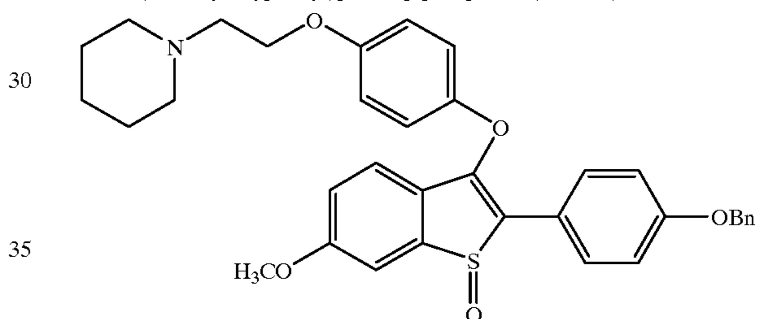
[6-Methoxy-3-[4-[2-(1-piperidinyl)ethoxy]phenoxy]-2-(4-benzyloxyphenyl)]benzo[b]thiophene-(S-oxide)
