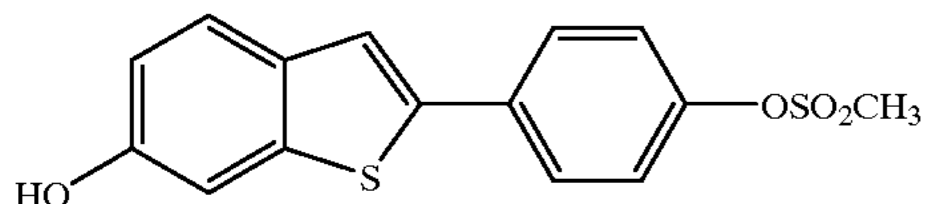
[6-Hydroxy-2-(4-methanesulfonyloxyphenyl)]benzo[b]thiophene
