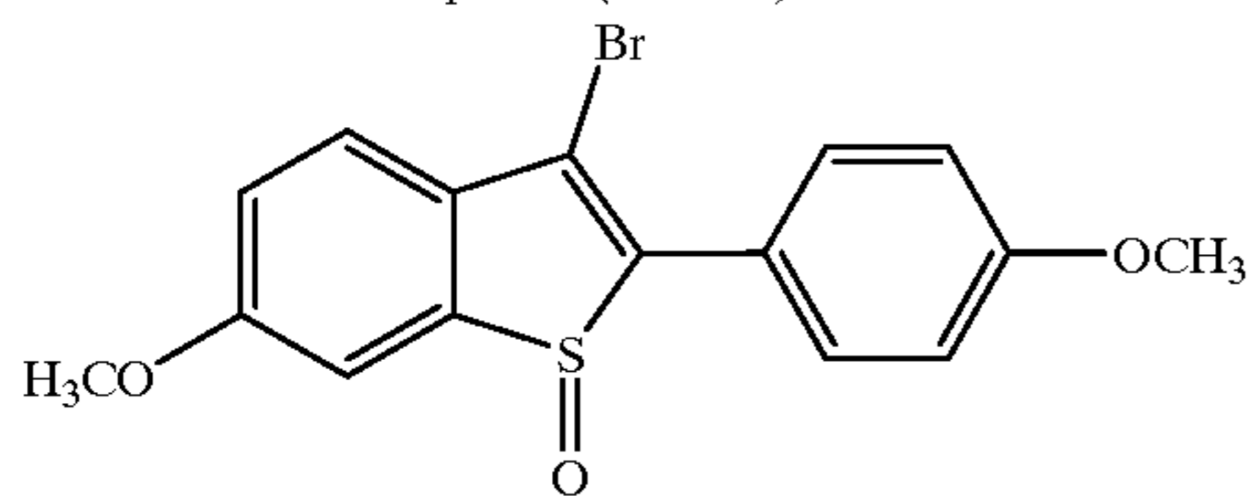
[6-methoxy-2-(4-methoxyphenyl)-3-bromo]benzo[b]thiophene-(S-oxide)
