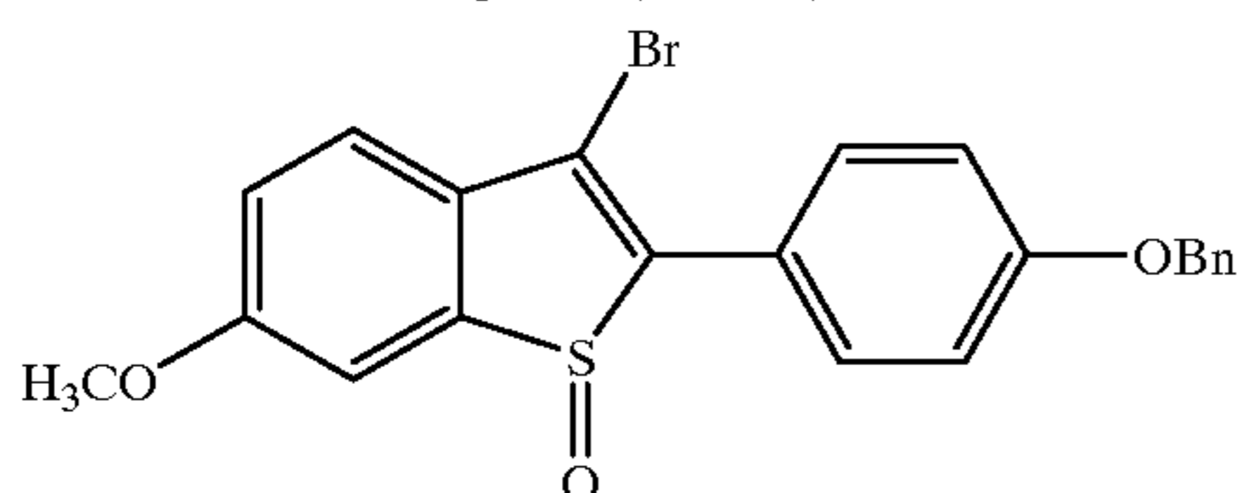
[6-Methoxy-2-(4-benzyloxyphenyl)-3-bromo]benzo[b]thiophene-(S-oxide)
