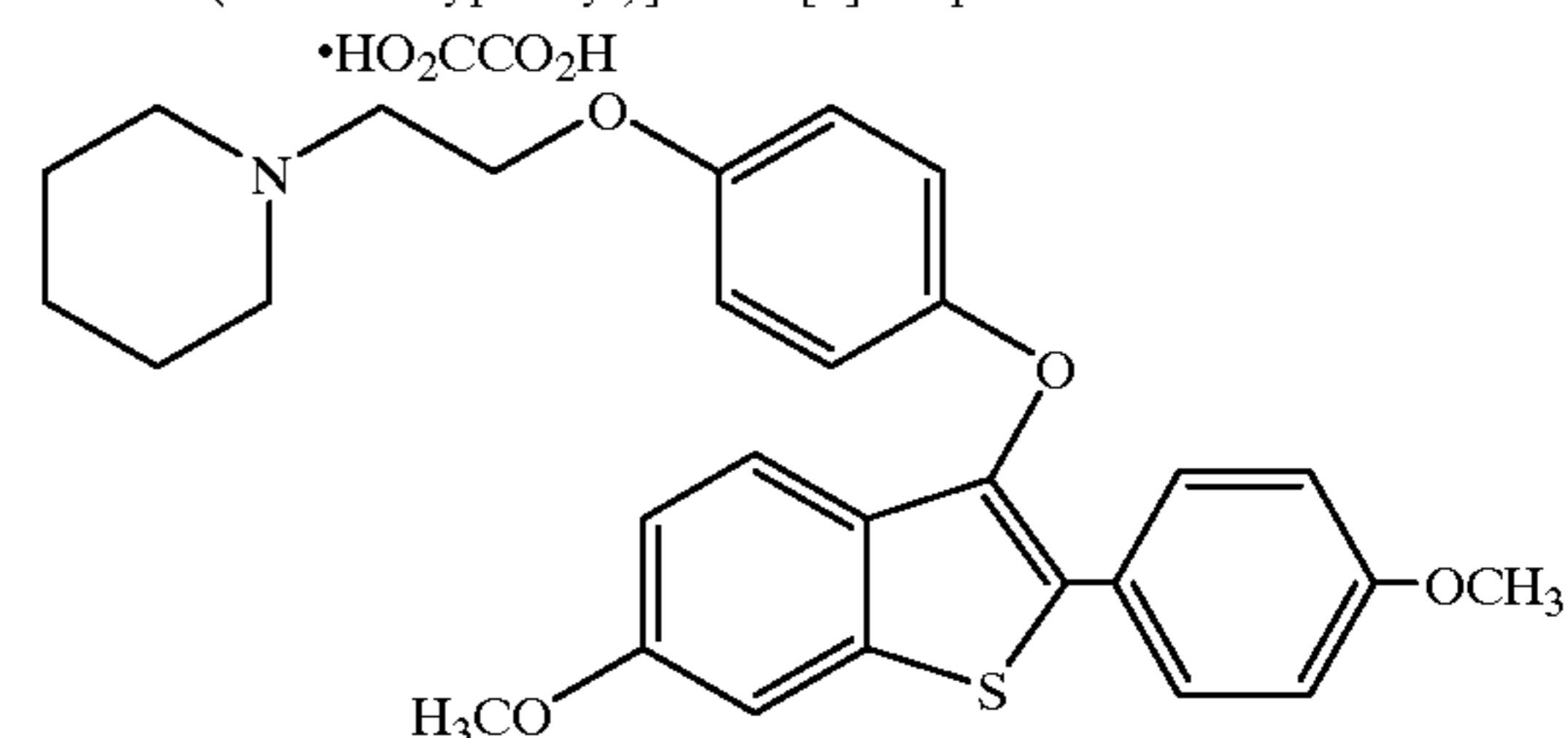
[6-methoxy-3-[4-[2-(1-piperidinyloxy)]phenoxy]-2-(4-methoxyphenyl)]benzo[b]thiophene.
