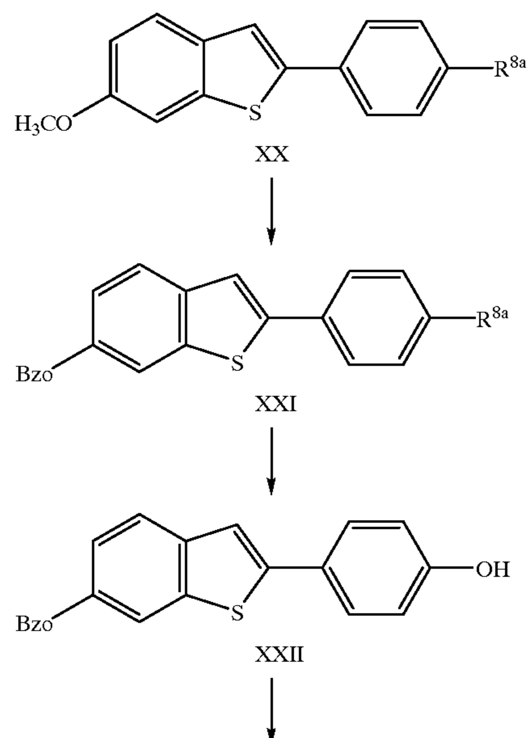
Scheme VII
