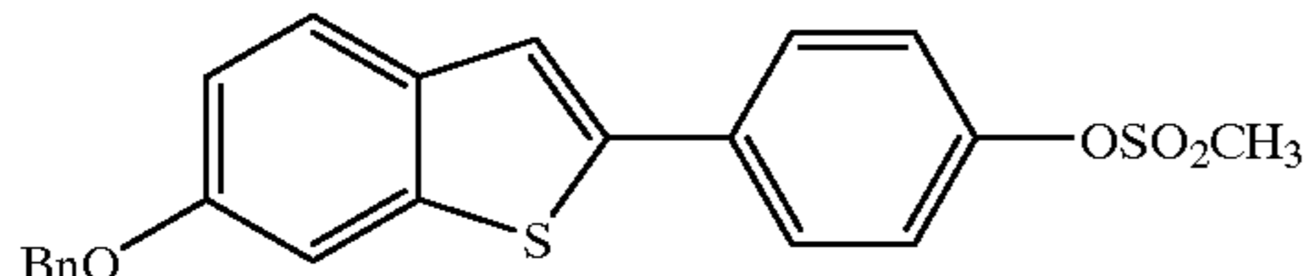
[6-Benzyloxy-2-(4-methanesulfonyloxyphenyl)]benzo[b]thiophene
