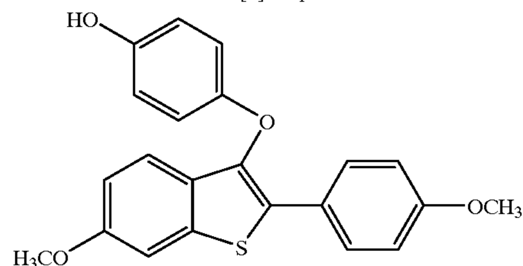
[6-methoxy-2-(4-methoxyphenyl)-3-(4-hydroxy)phenoxy]benzo[b]thiophene
