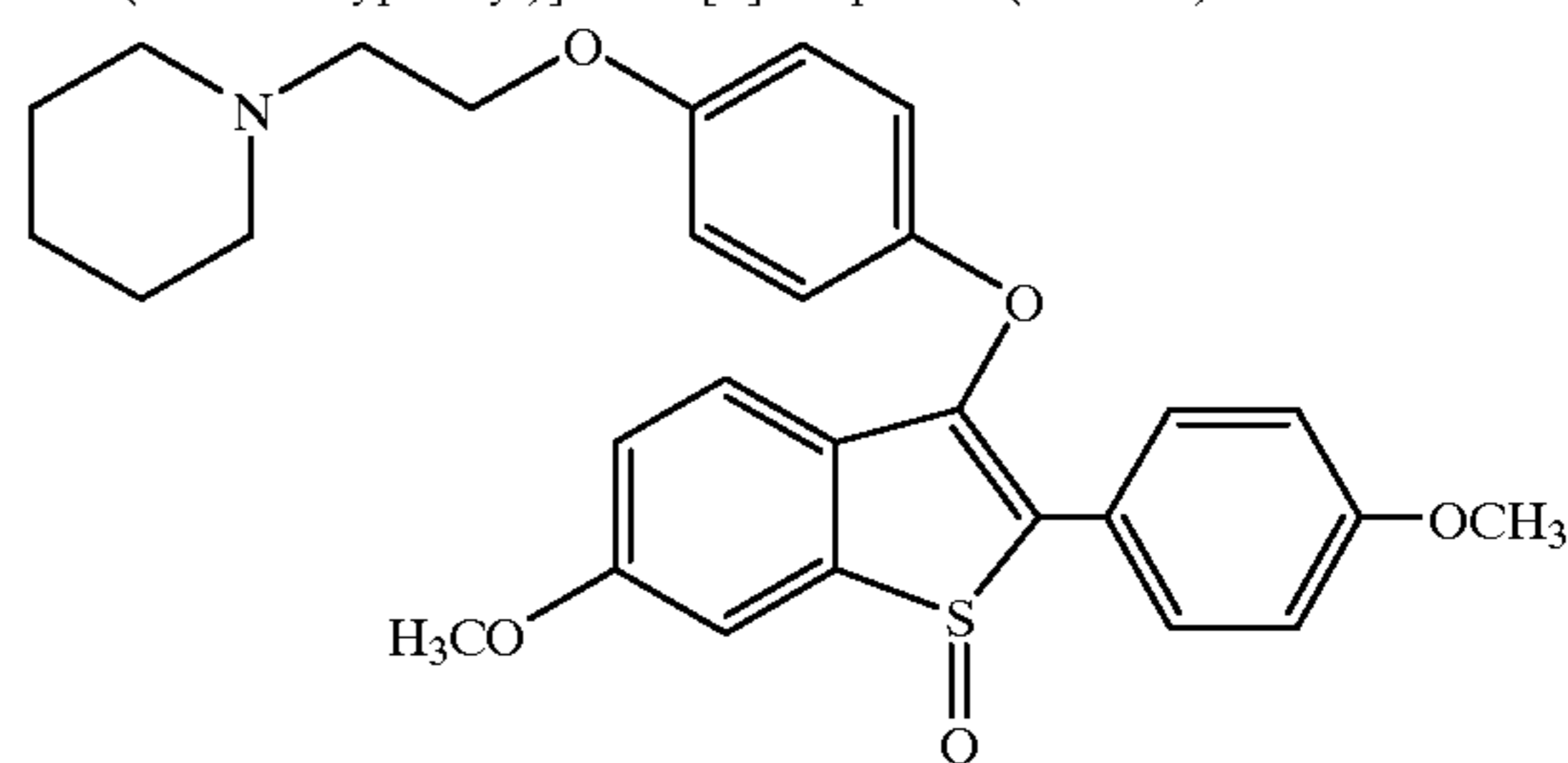
[6-Methoxy-3-[4-[2-(1-piperidinyl)ethoxy]phenoxy]-2-(4-methoxyphenyl)]benzo[b]thiophene-(S-oxide)
