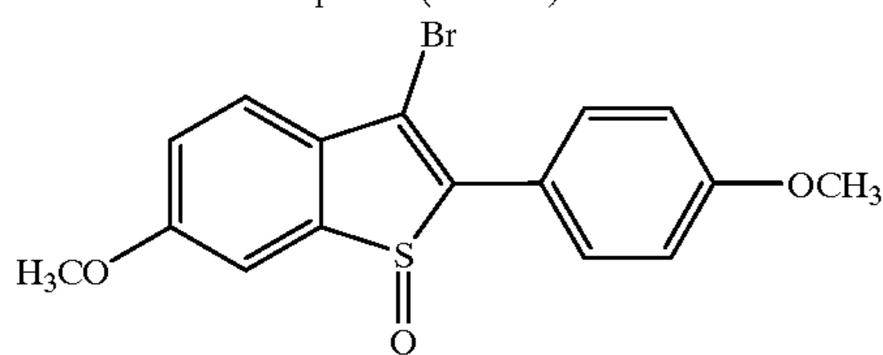
[6-methoxy-2-(4-methoxyphenyl)-3-bromo]benzo[b]thiophene-(S-oxide)
