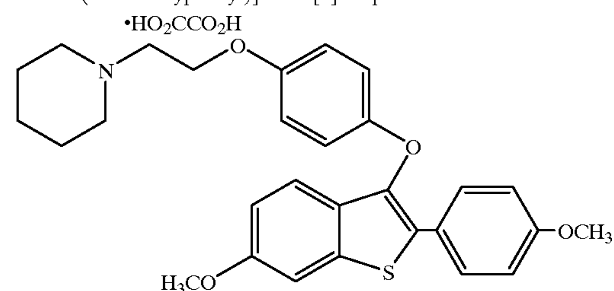
[6-methoxy-3-[4-[2-(1-piperidiny)ethoxy]-phenoxy]-2-(4-methoxyphenyl)]benzo[b]thiophene.
