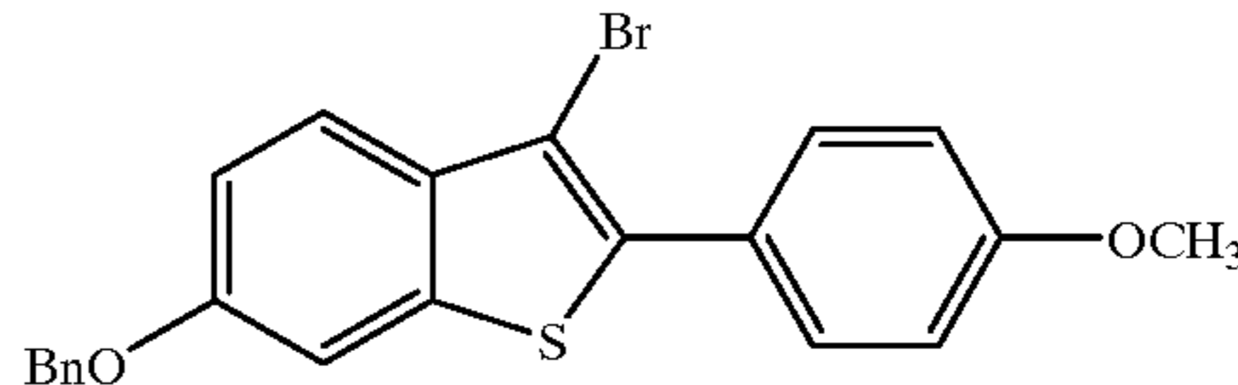
[6-Benzyloxy-2-(4-methoxyphenyl)-3-bromo]benzo[b]thiophene
