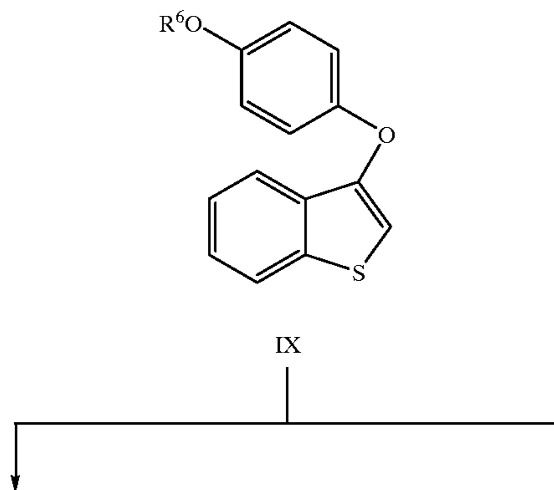
Scheme IV
