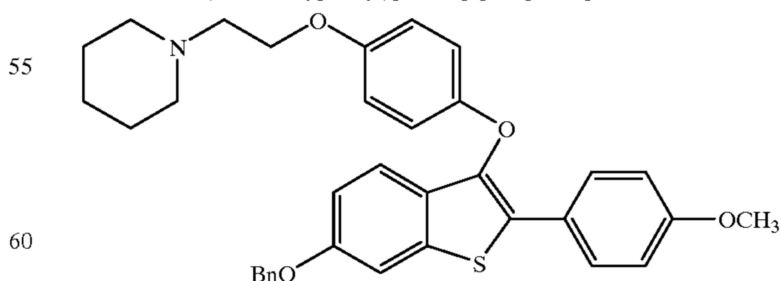
[6-Benzyloxy-3-[4-[2-(1-piperidinyl)ethoxy]phenoxy]-2-(4-methoxyphenyl)]benzo[b]thiophene
