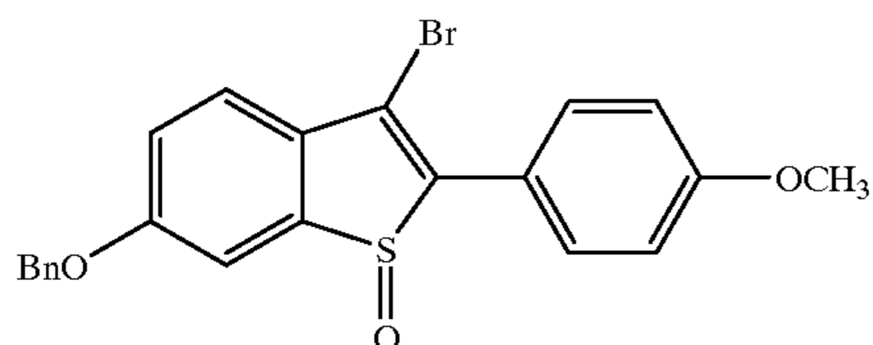
[6-Benzyloxy-2-(4-methoxyphenyl)-3-bromo]benzo[b]thiophene-(S-oxide)
