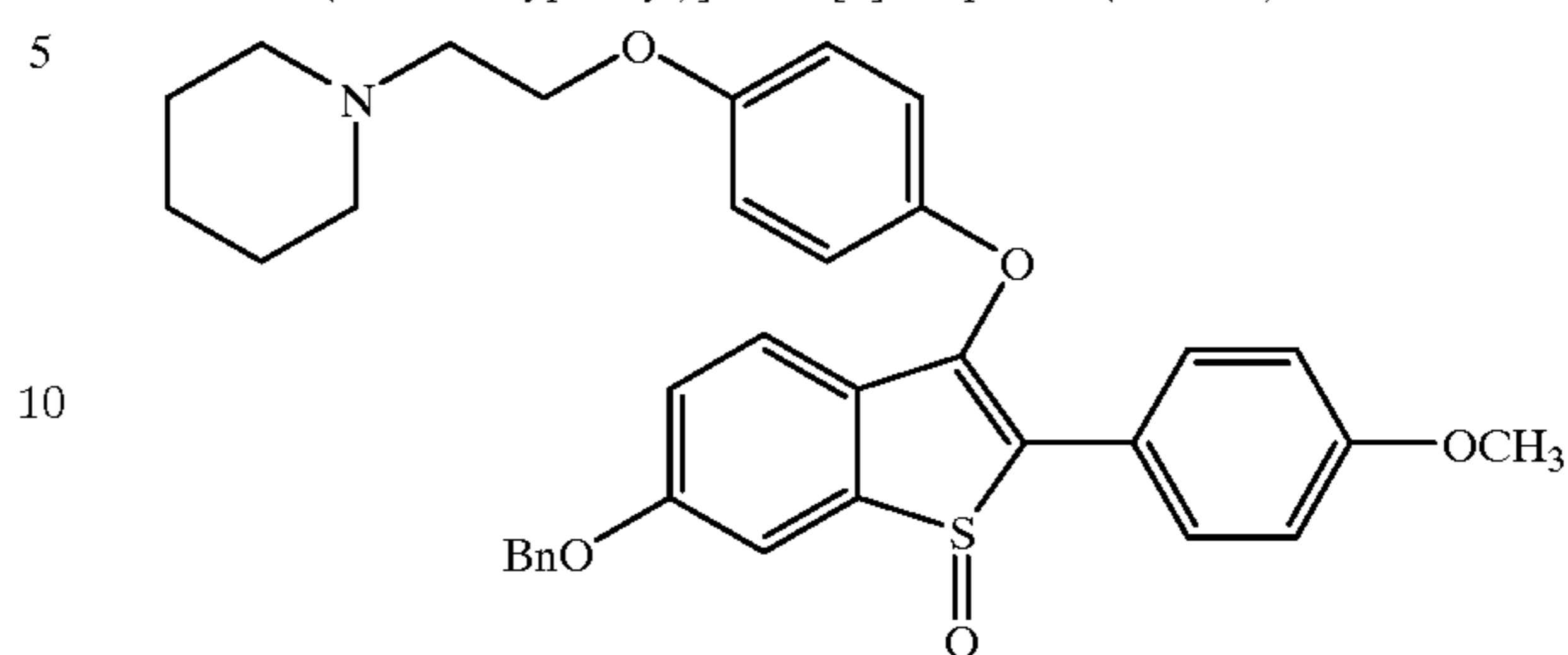
[6-Benzyloxy-3-[4-[2-(1-piperidinyl)ethoxy]phenoxy]-2-(4-methoxyphenyl)]benzo[b]thiophene-(S-oxide)
