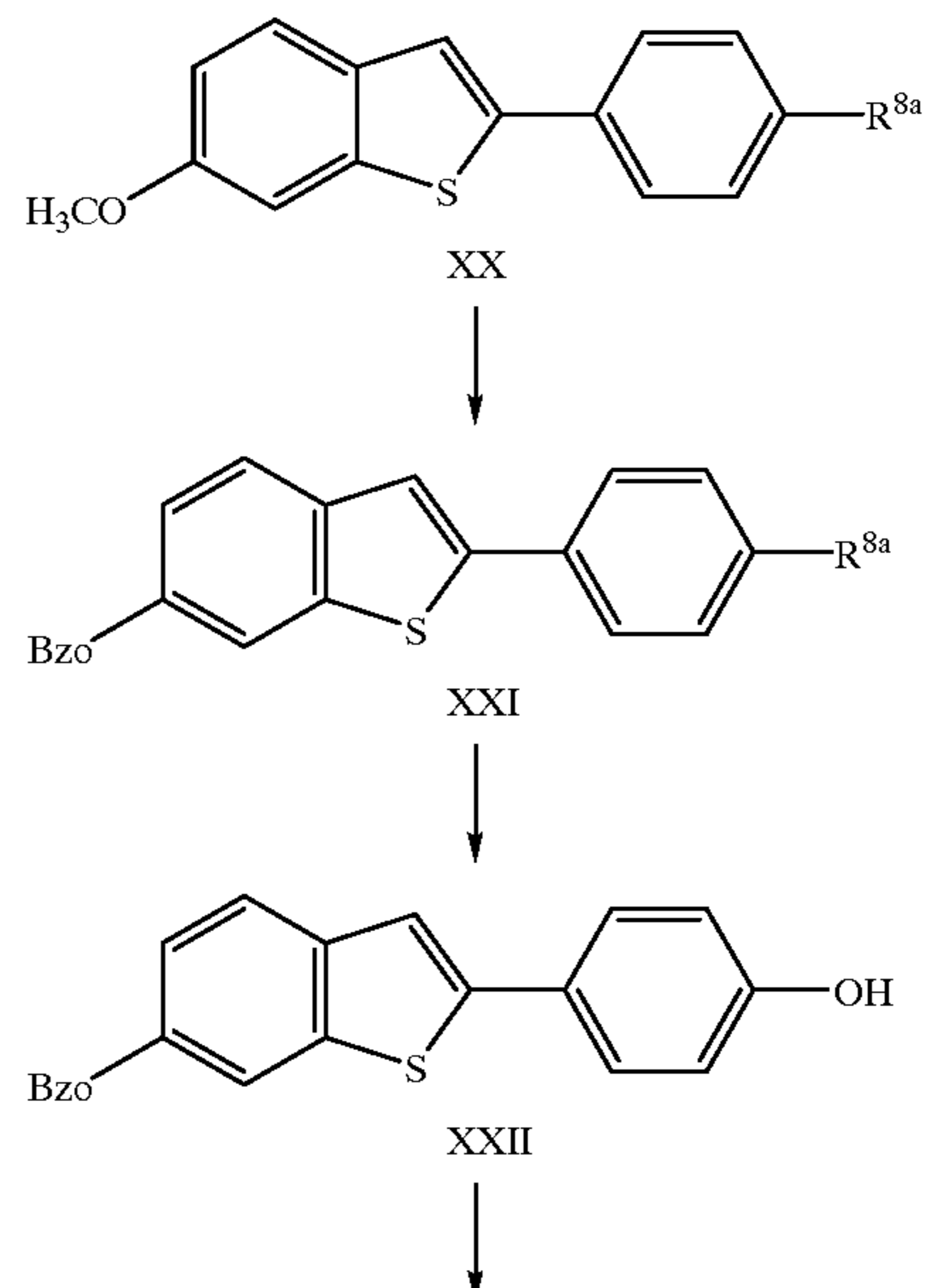
Scheme VII
