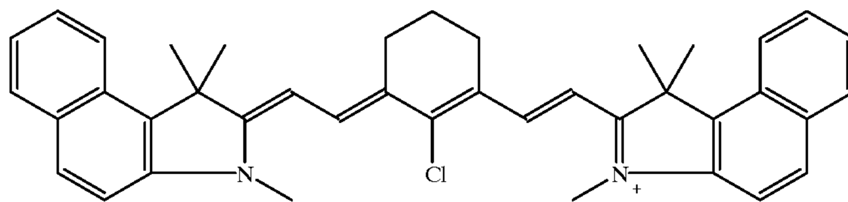
p-Toluenesulfonate
