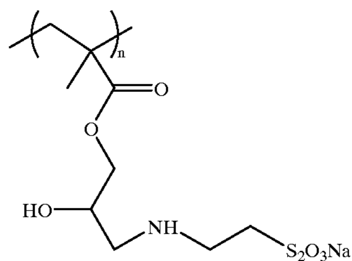
polymer 14
