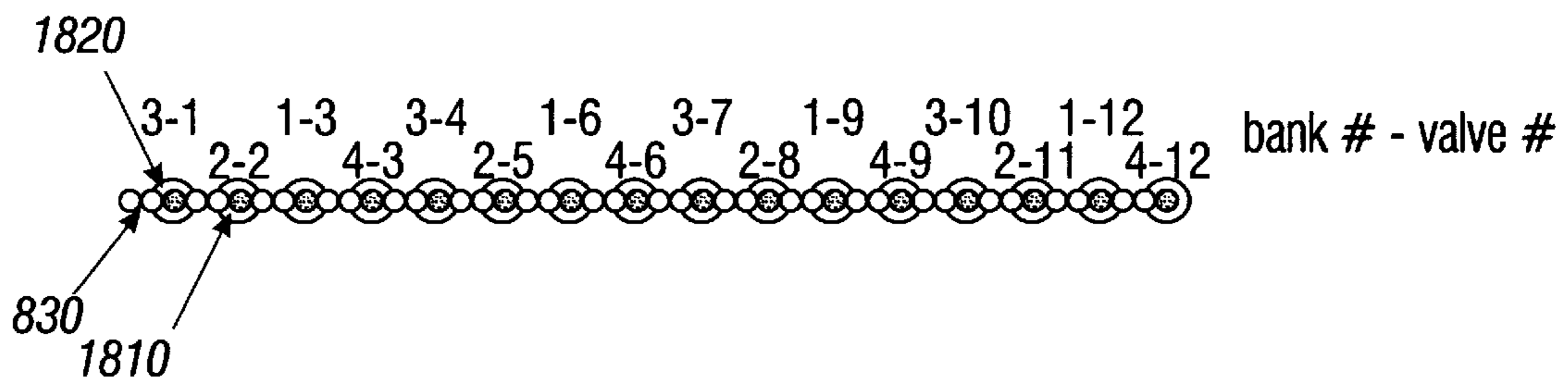
Dispensing into 384 well plate, 3.4mm diam. wells
