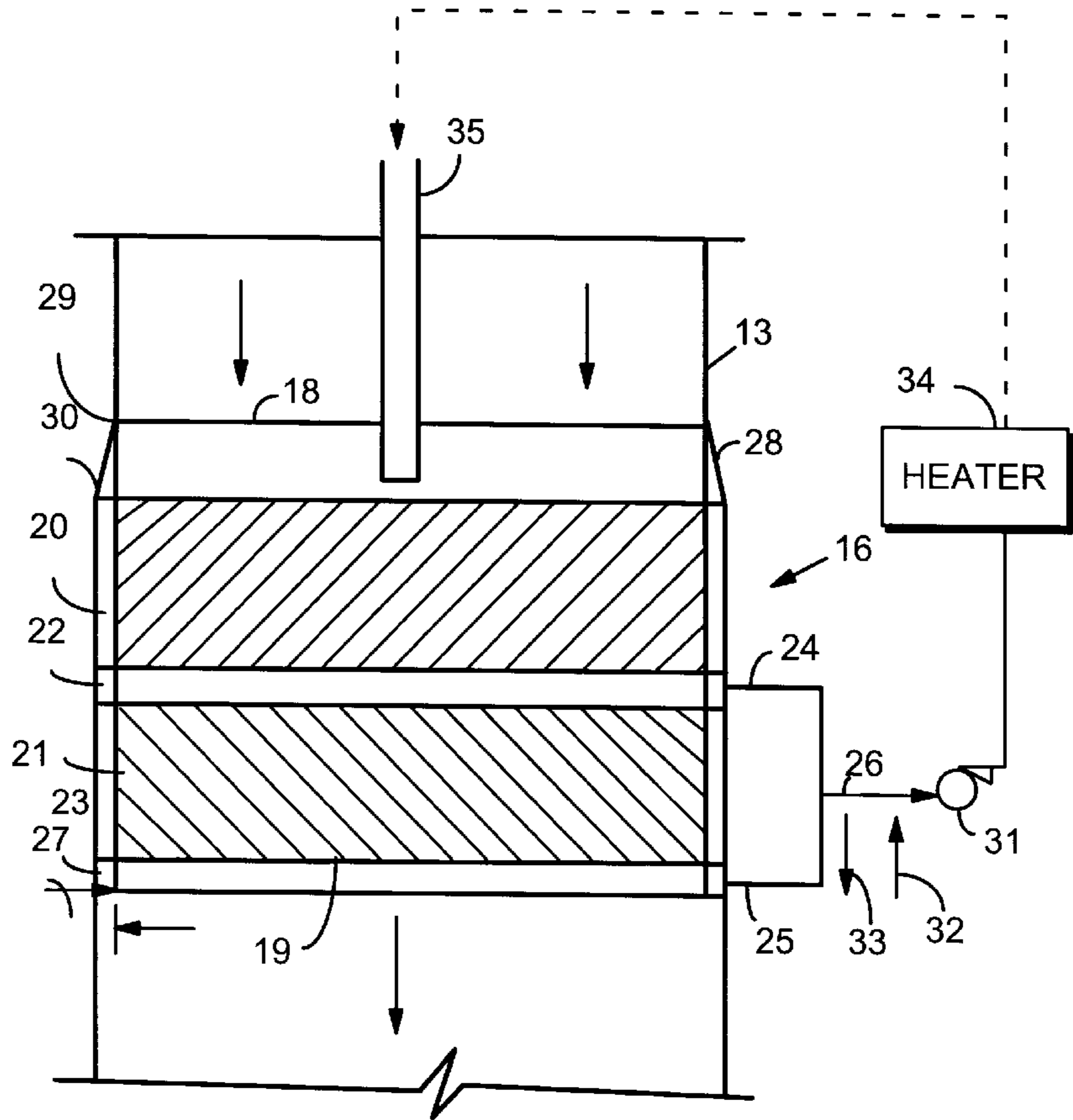
Fig. 2 (PRIOR ART)
