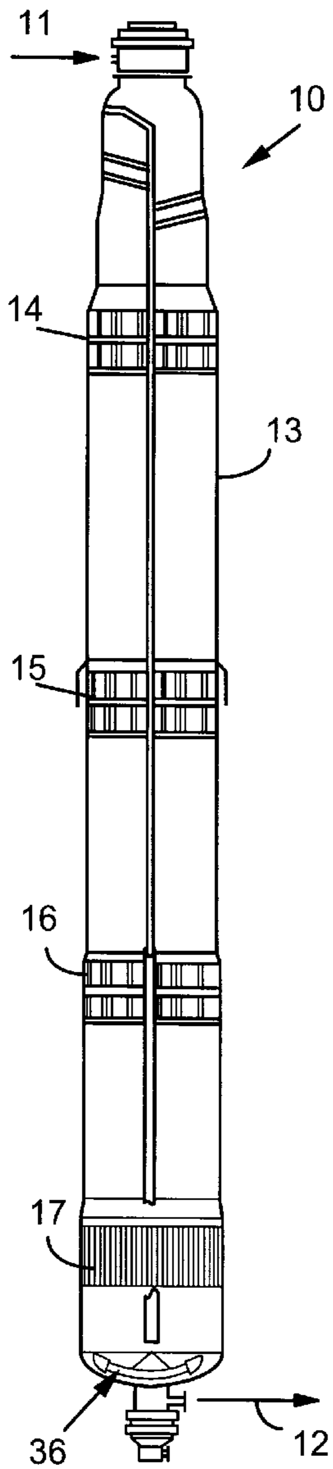
Fig. 1 (PRIOR ART)
