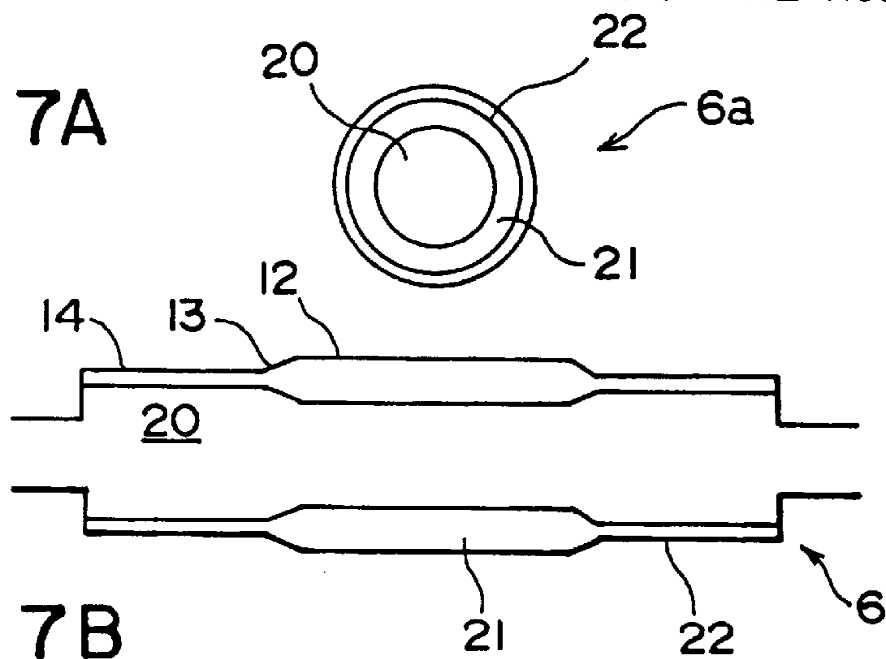
SECTIONAL SURFACE OF THE ROLL
