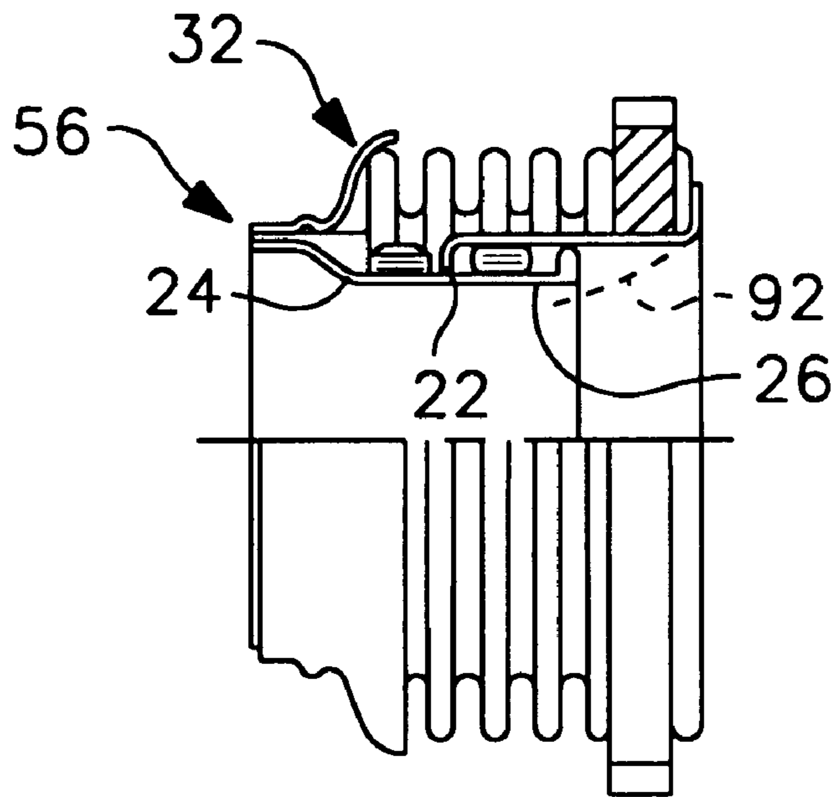
ASSEMBLE & SIZE END CAP
