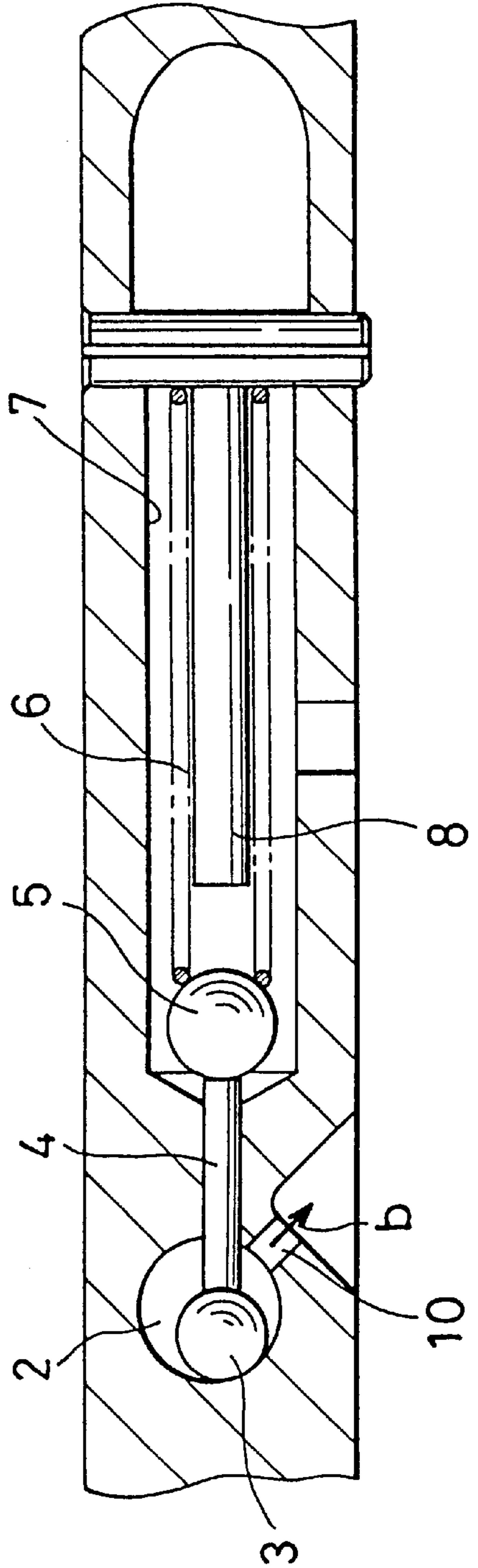
FIG. 2 PRIOR ART
