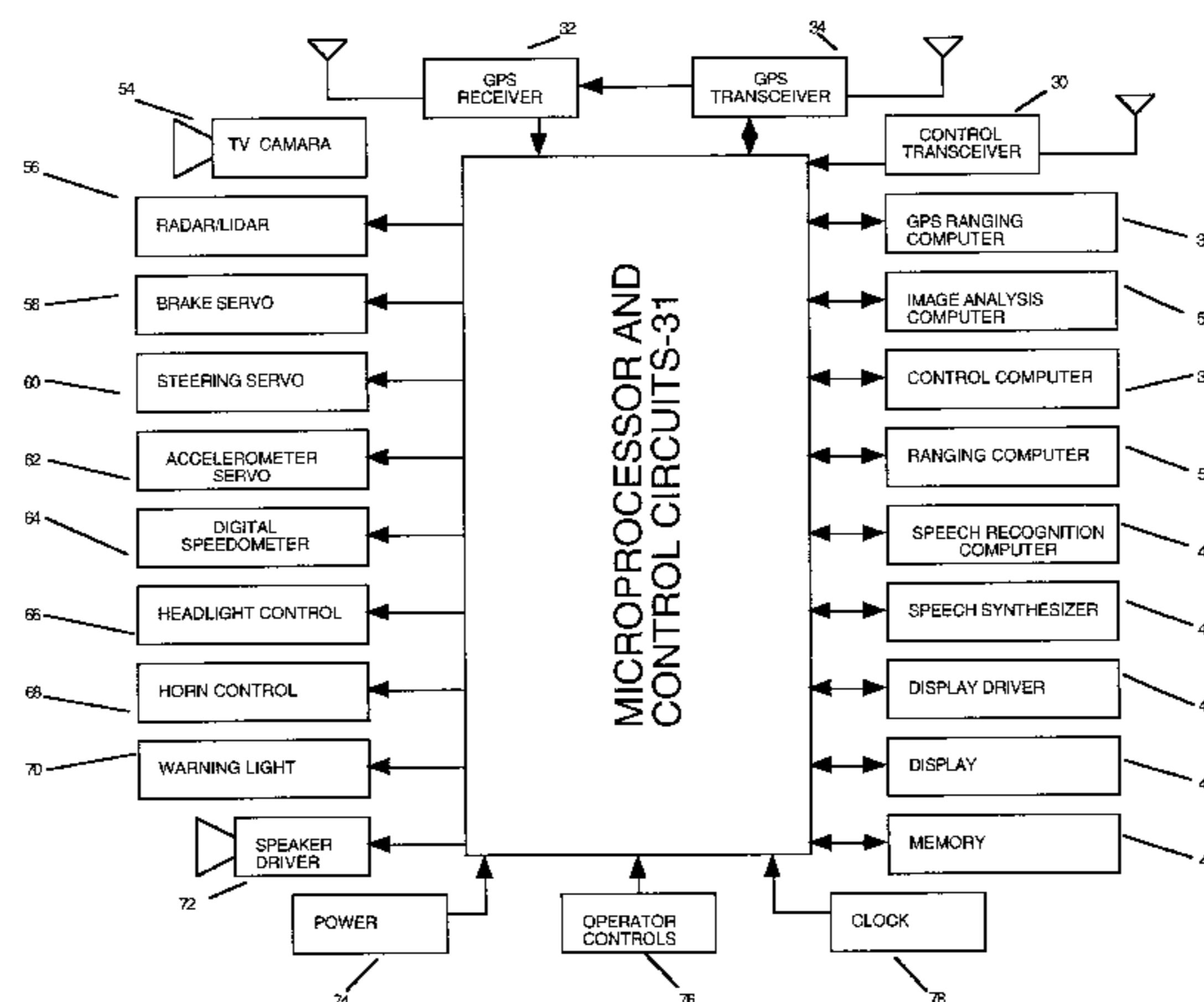
VEHICLE SYSTEM BLOCK DIAGRAM
