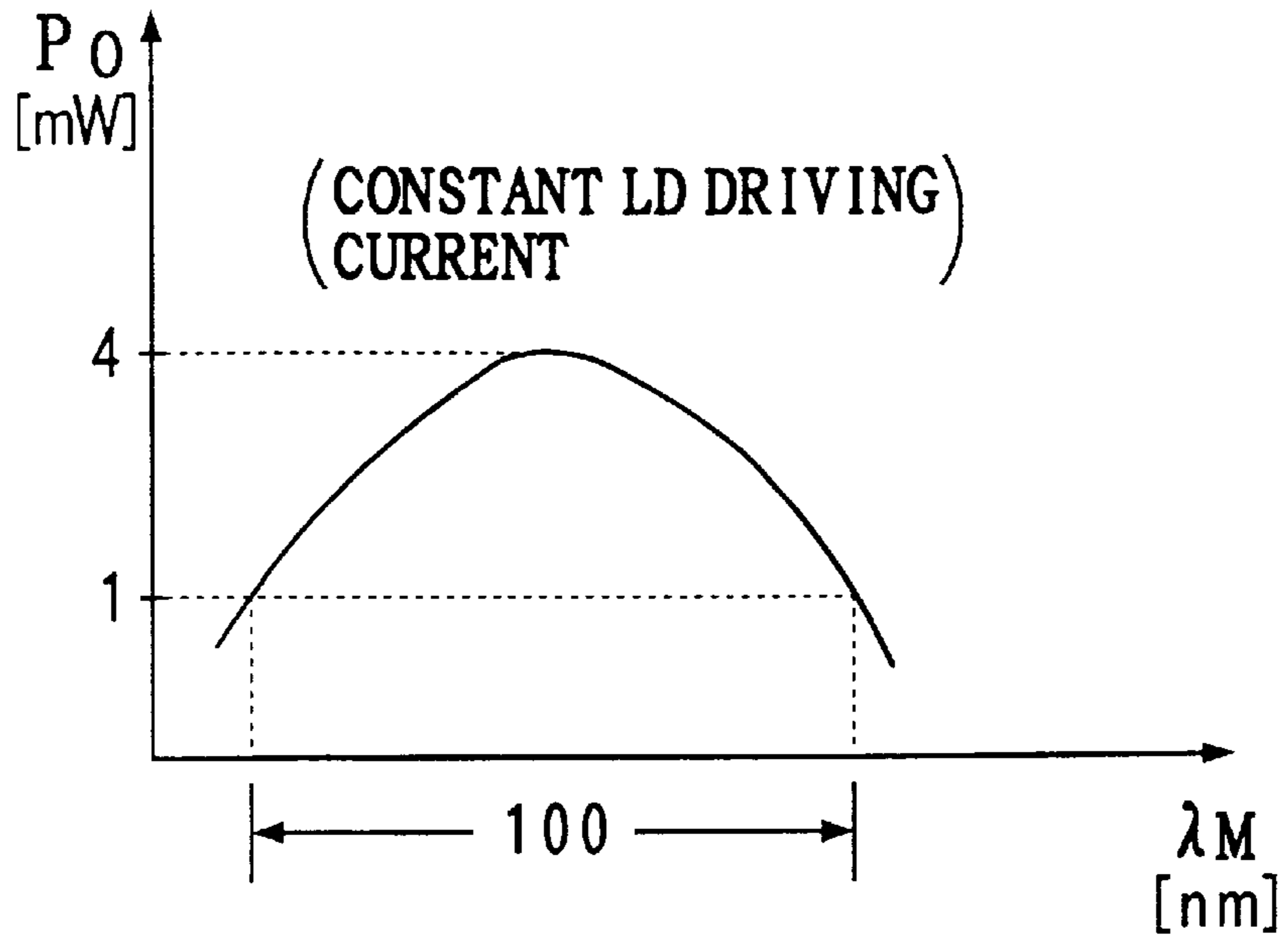
FIG. 13 PRIOR ART
