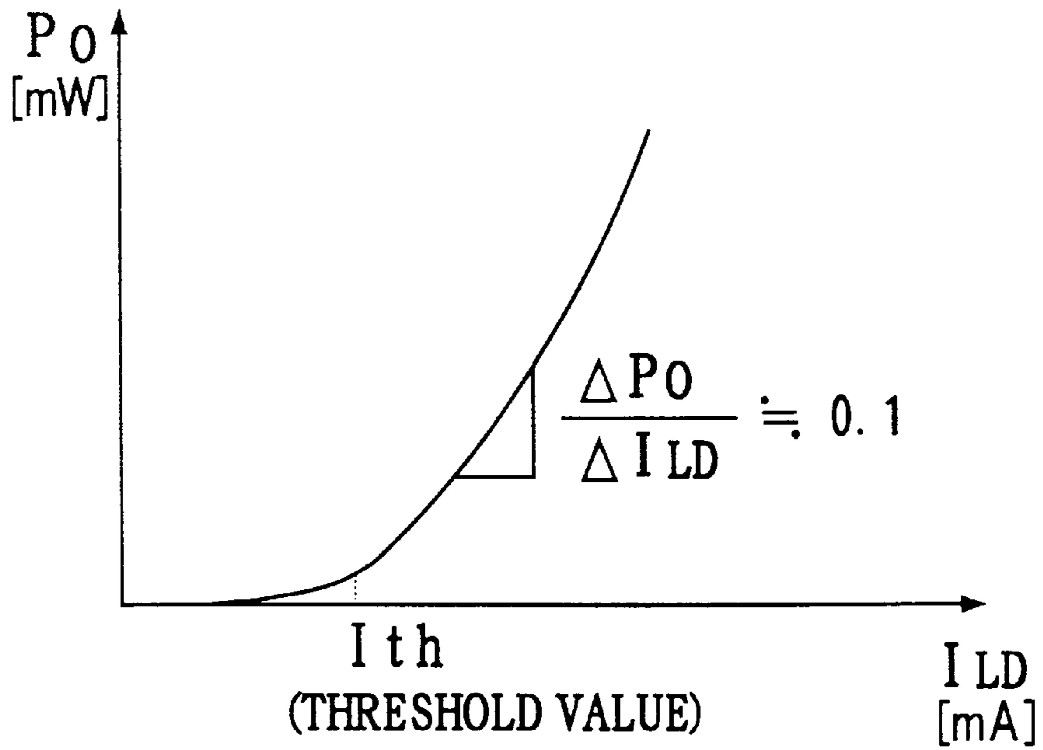
FIG. 15 PRIOR ART
