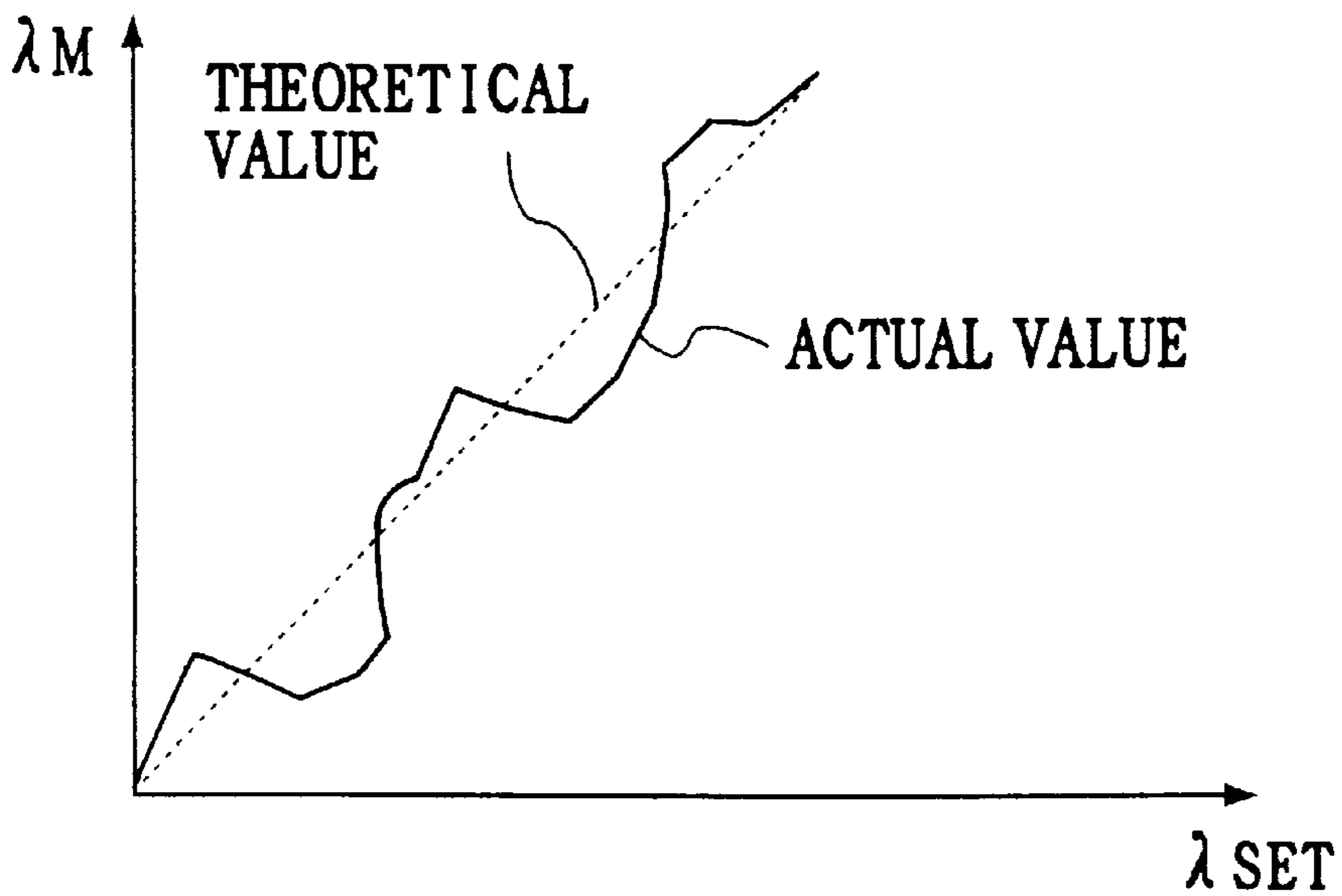
FIG. 16 PRIOR ART
