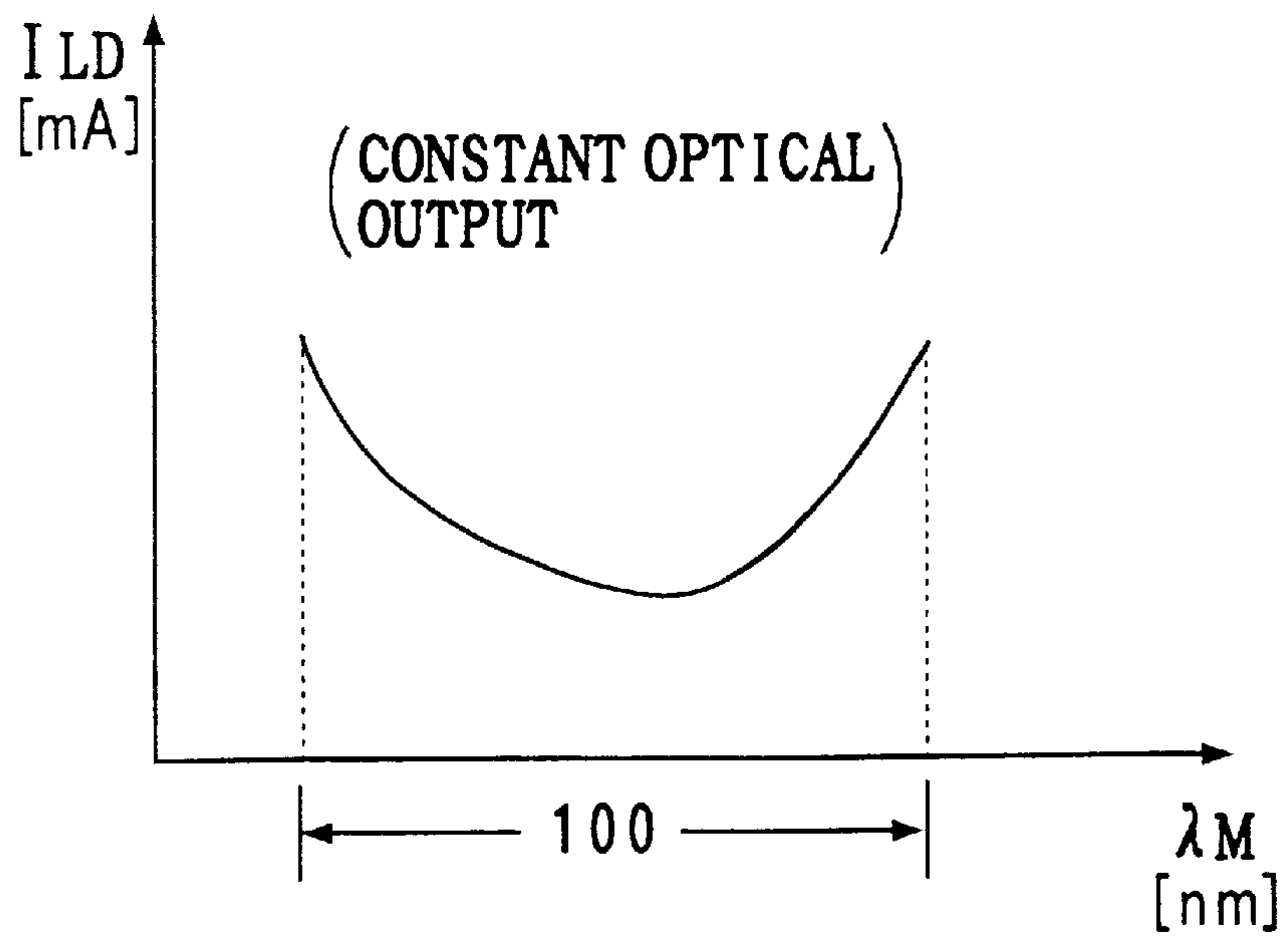
FIG. 14 PRIOR ART
