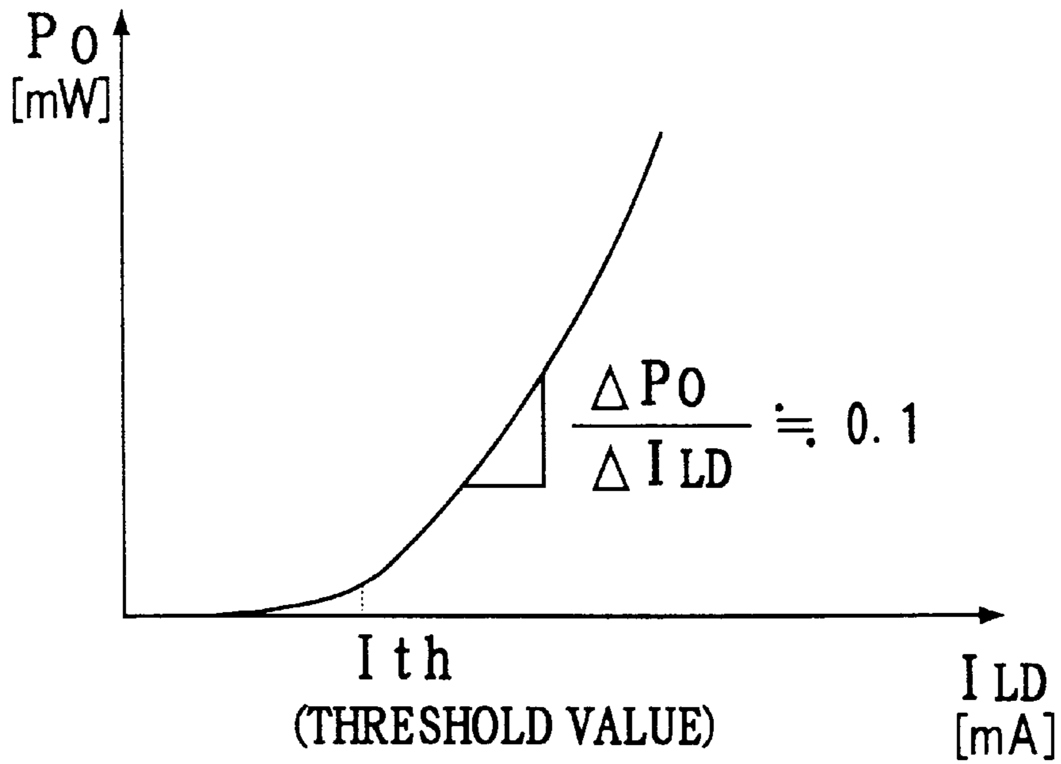
FIG. 15 PRIOR ART
