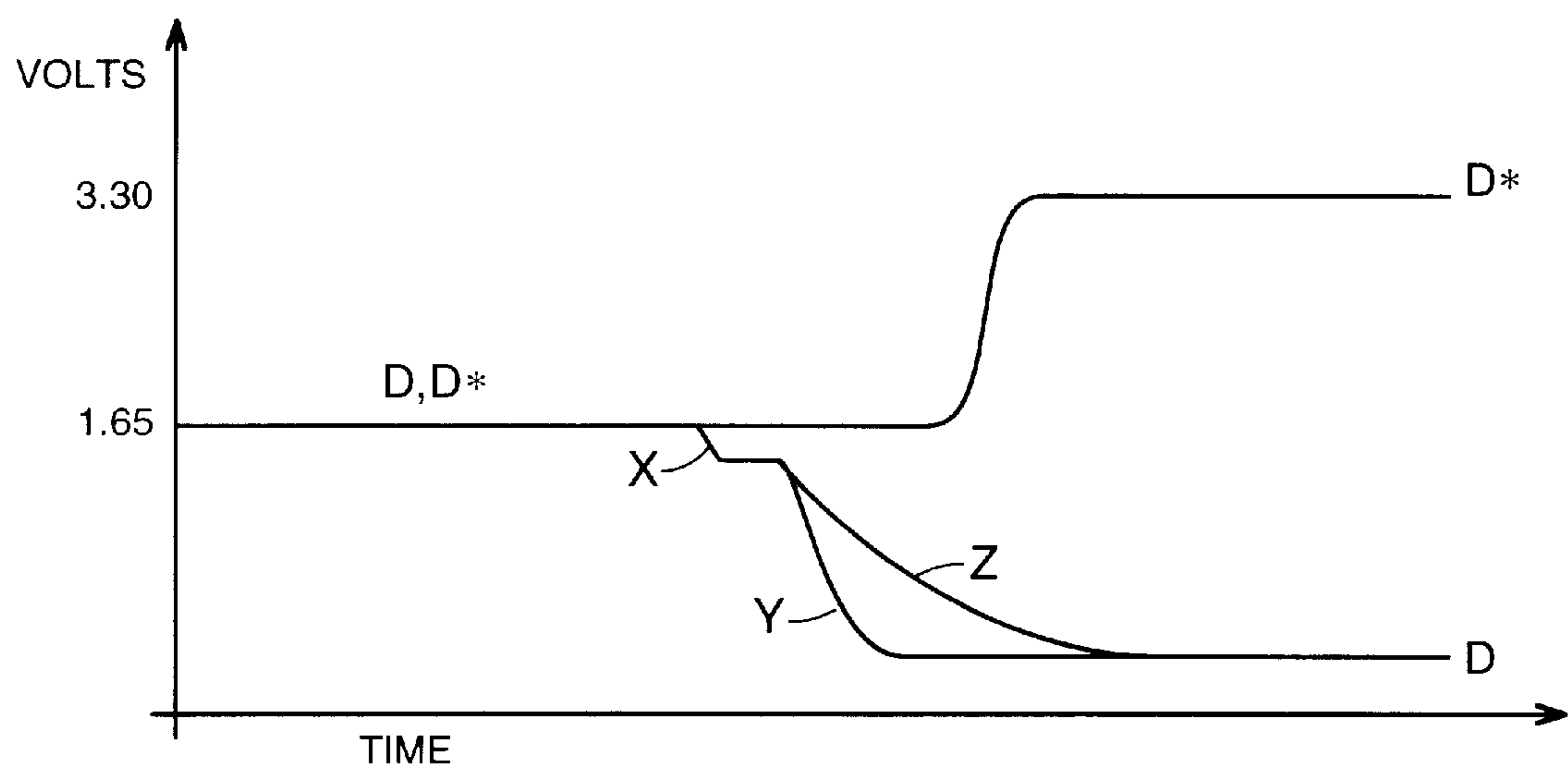
FIG. 2 (PRIOR ART)
