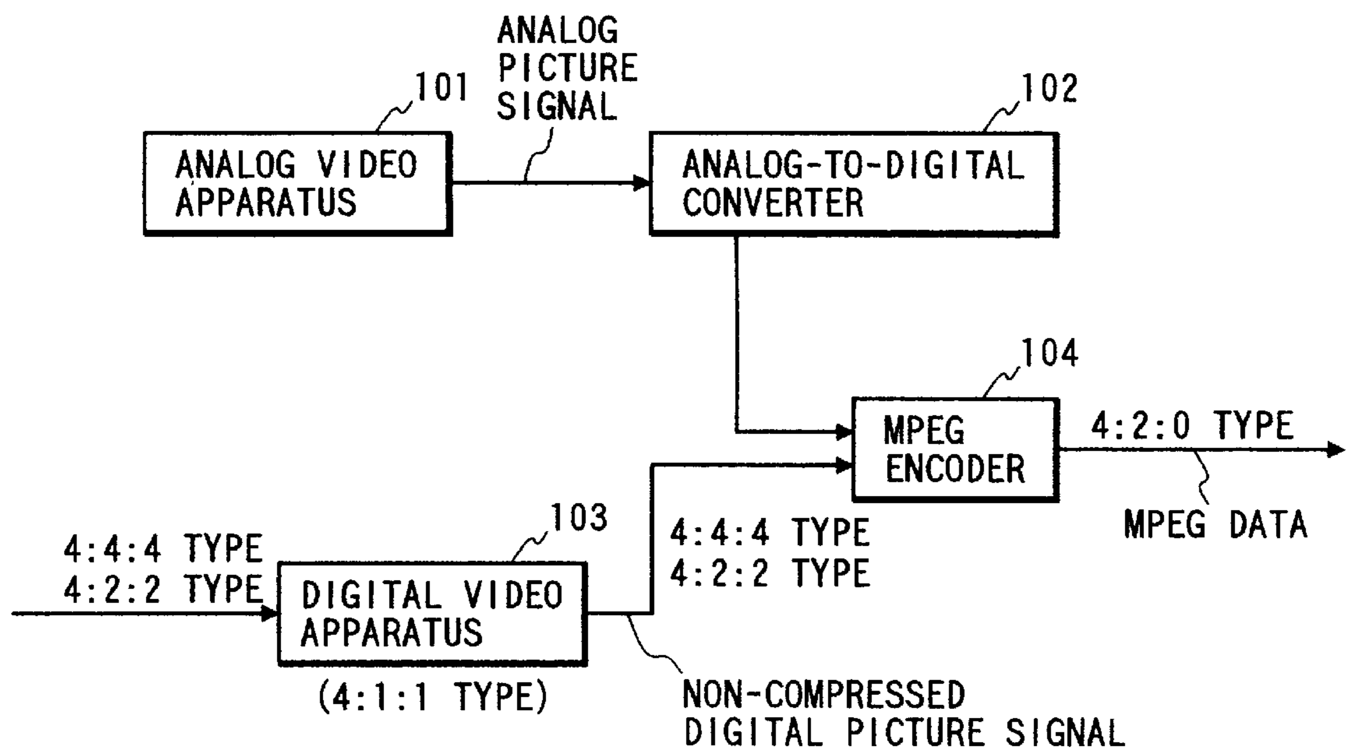
FIG. 5 PRIOR ART
