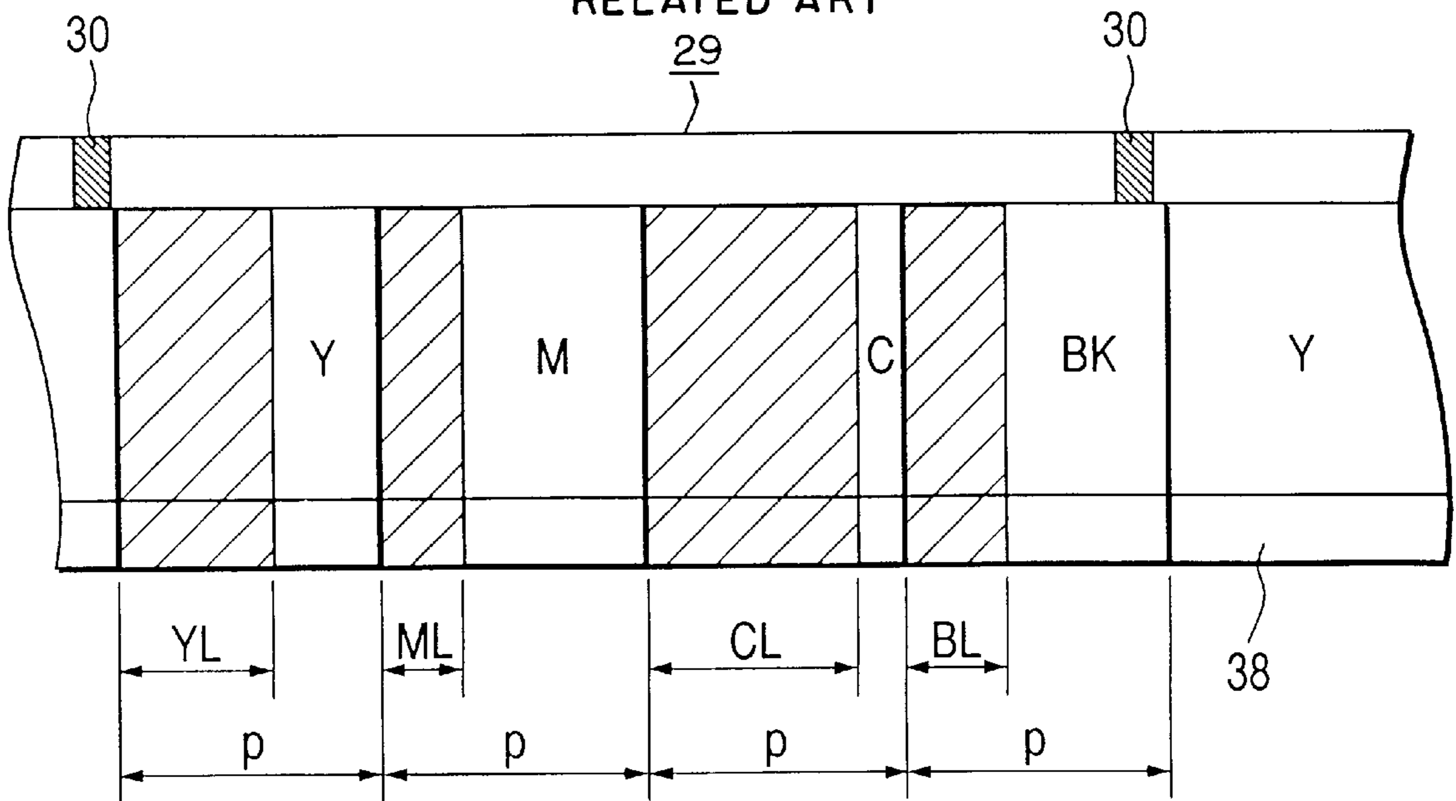
FIG. 13 RELATED ART
