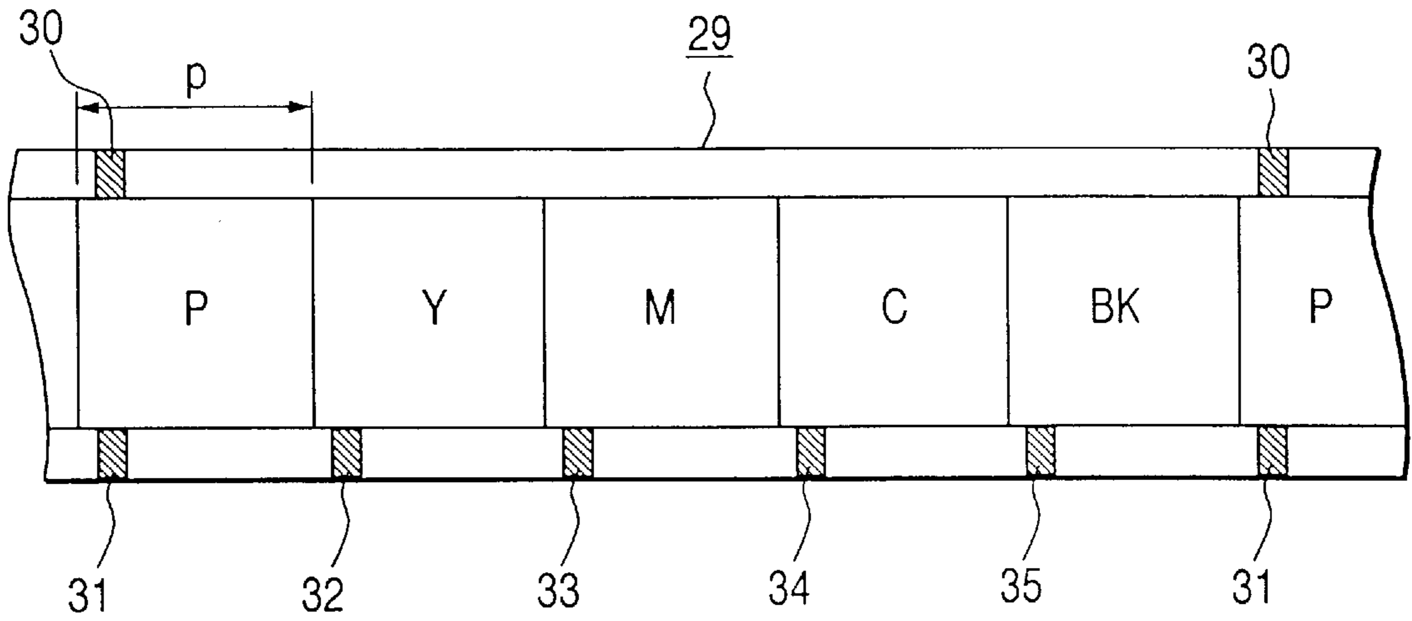
FIG. 10 RELATED ART
