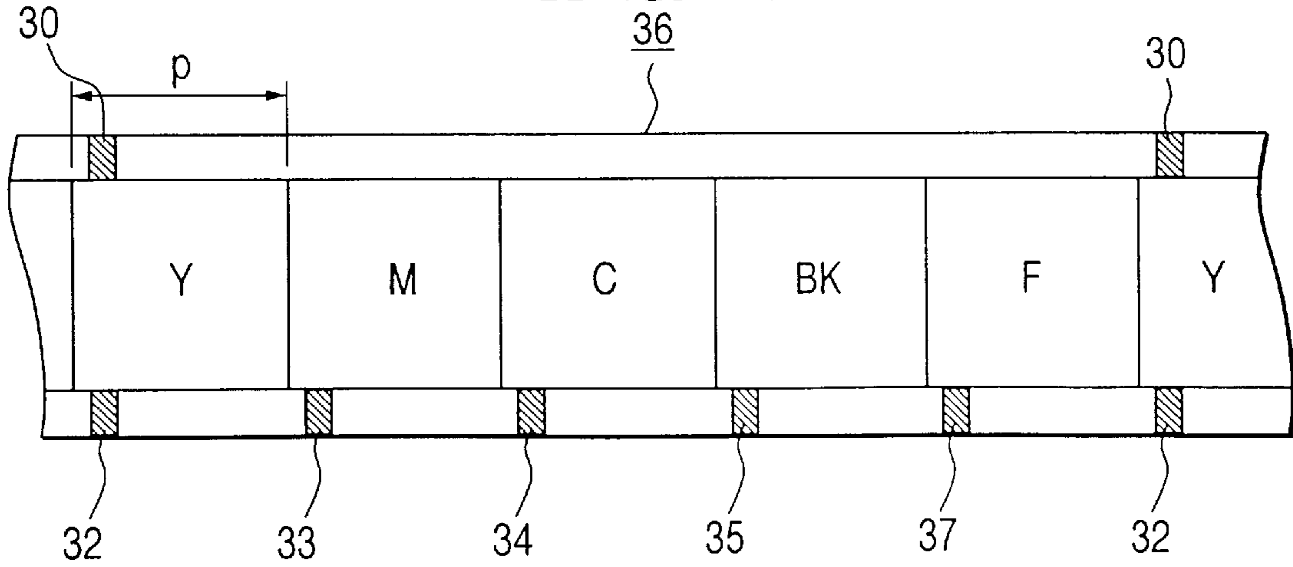
FIG. 11 RELATED ART
