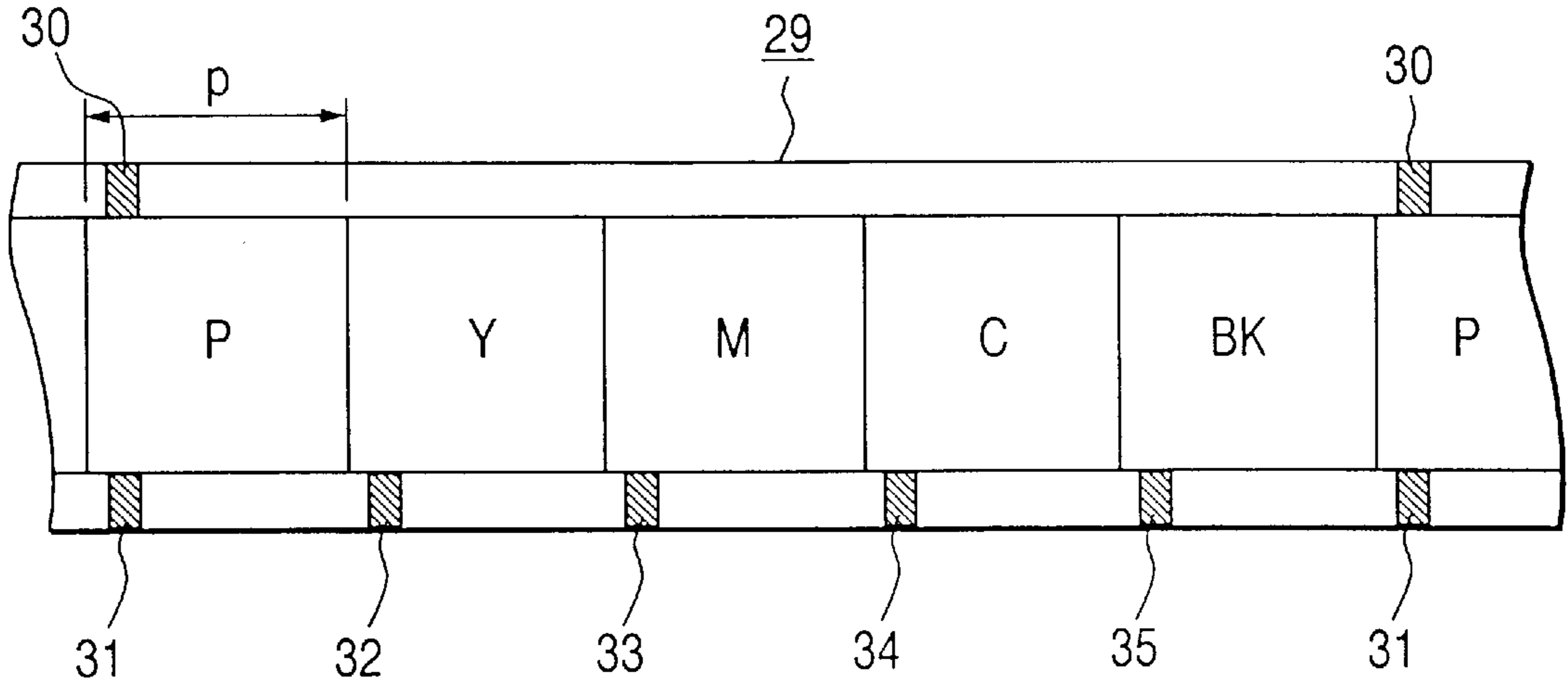
FIG. 10 RELATED ART
