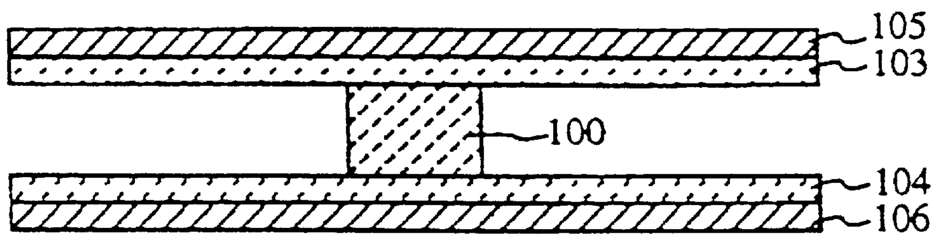
FIG. 26C PRIOR ART
