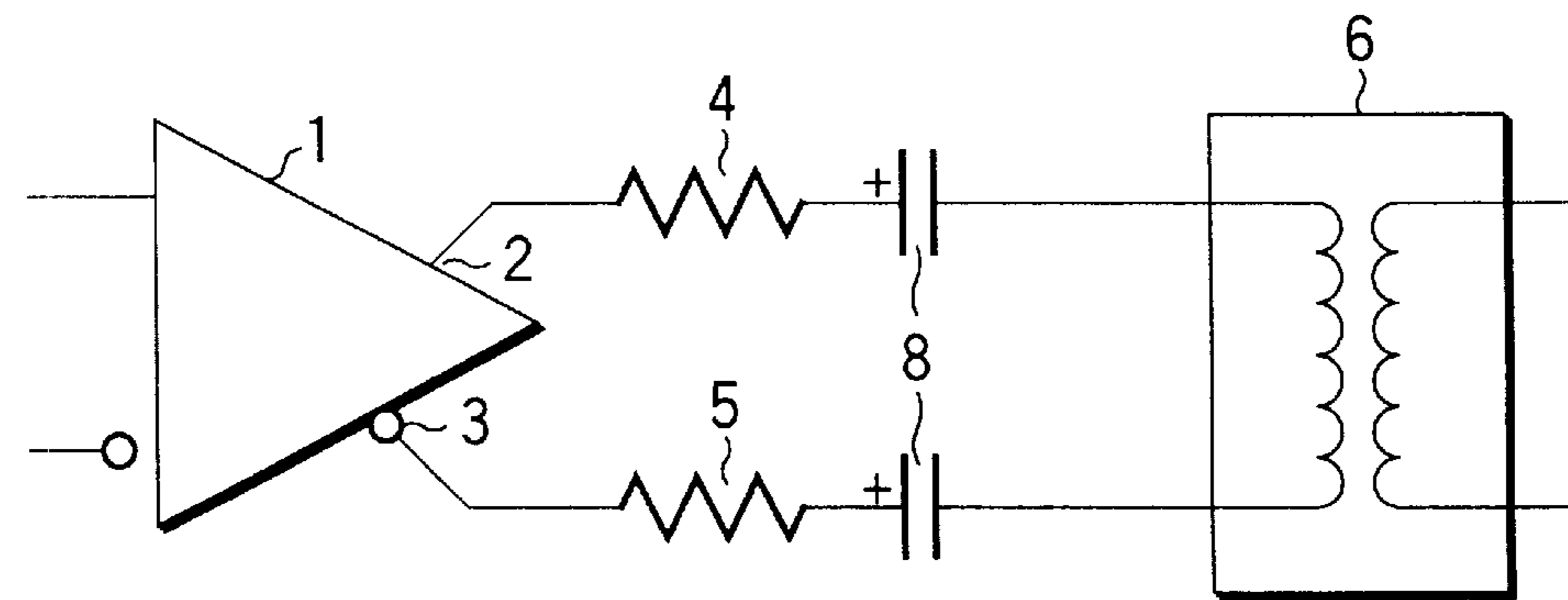
FIG. 6 PRIOR ART
