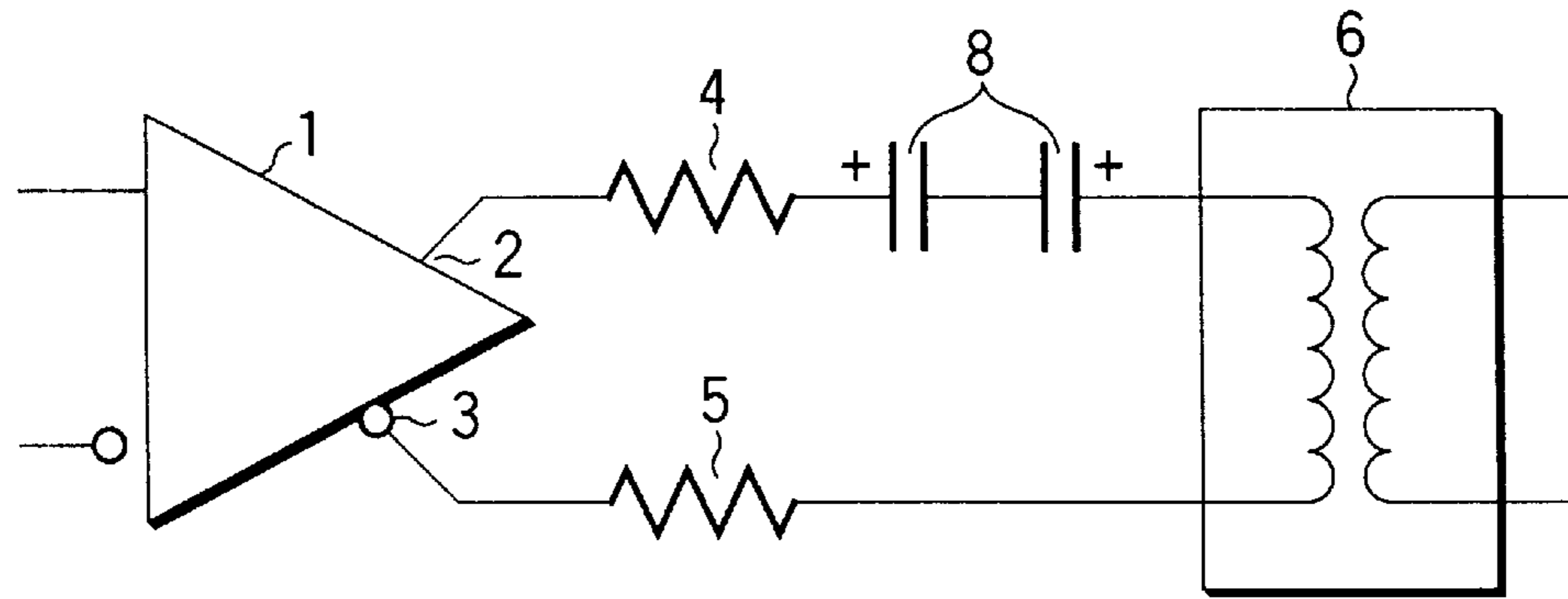
FIG. 5 PRIOR ART
