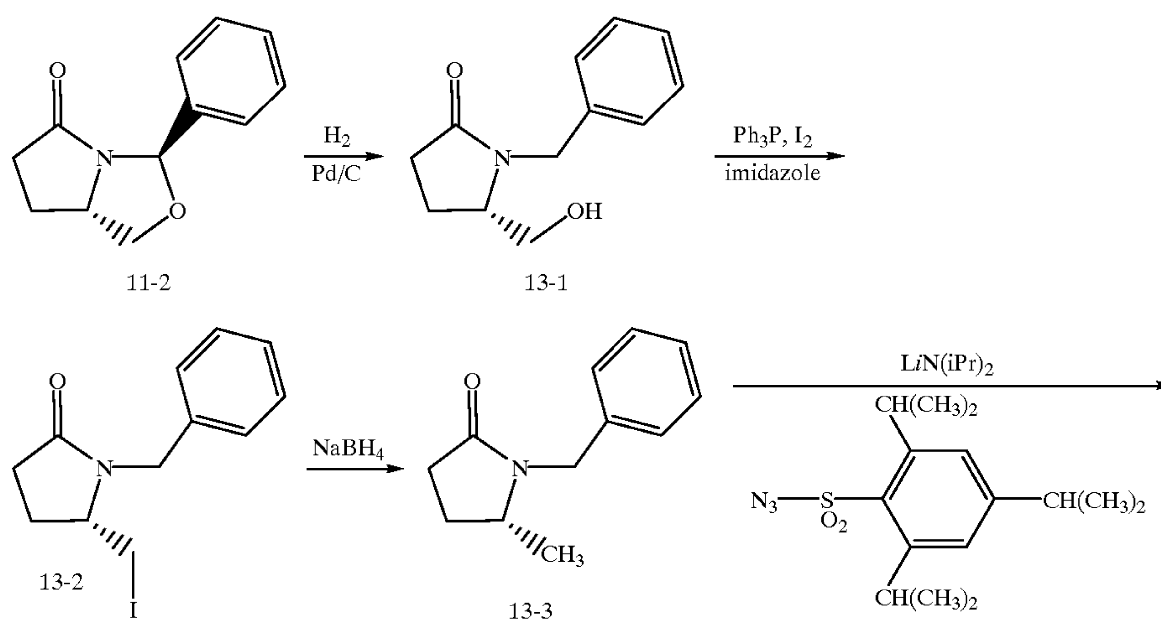
Scheme 13
