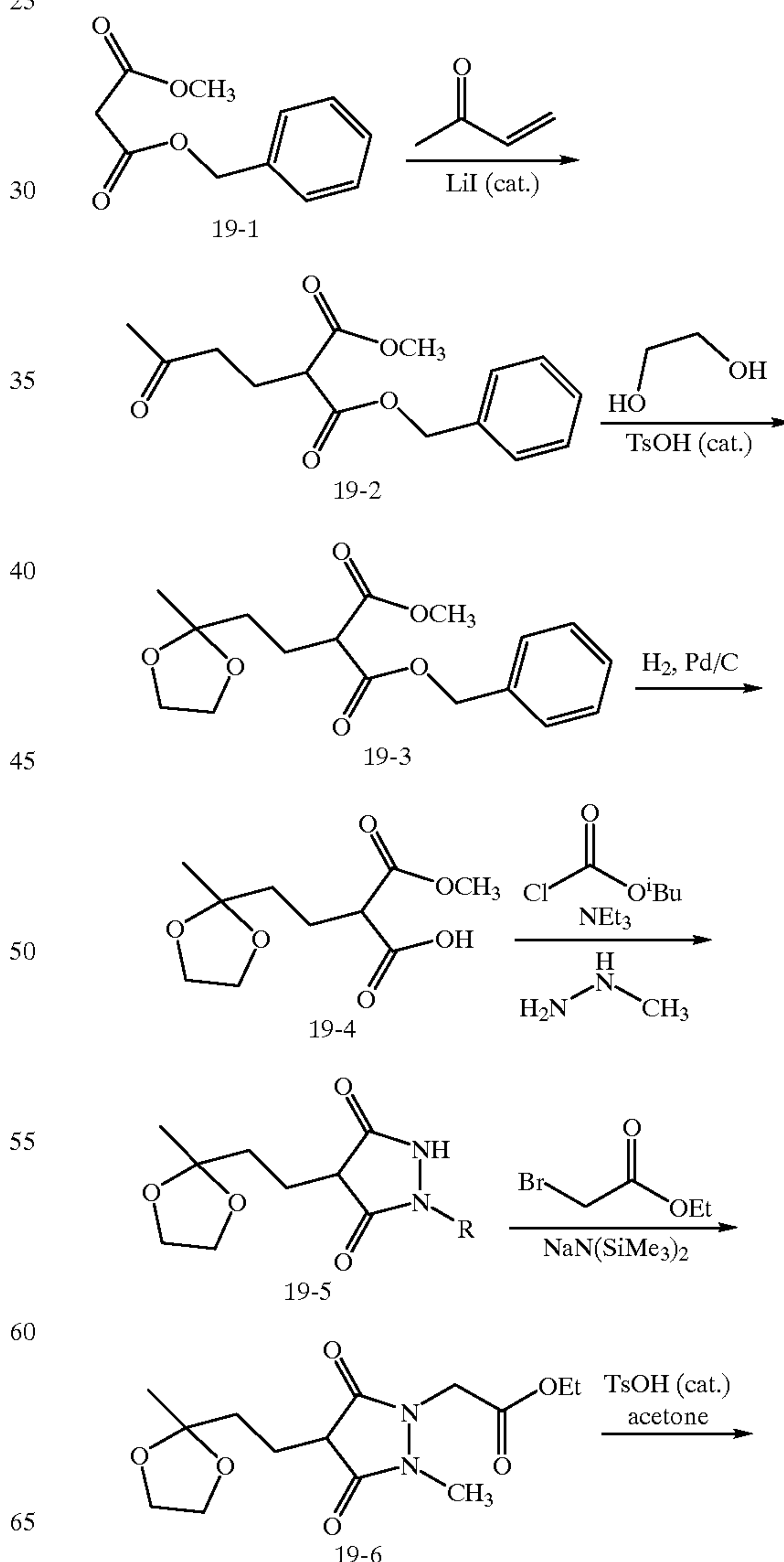
SCHEME 19
