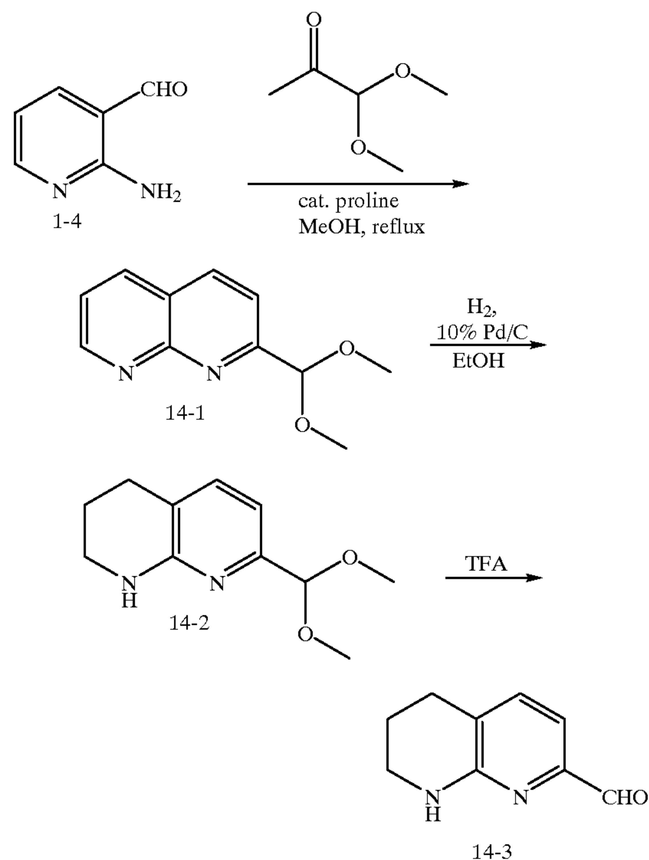
2-Dimethoxymethyl-[1,8]naphthyridine (14-1)
