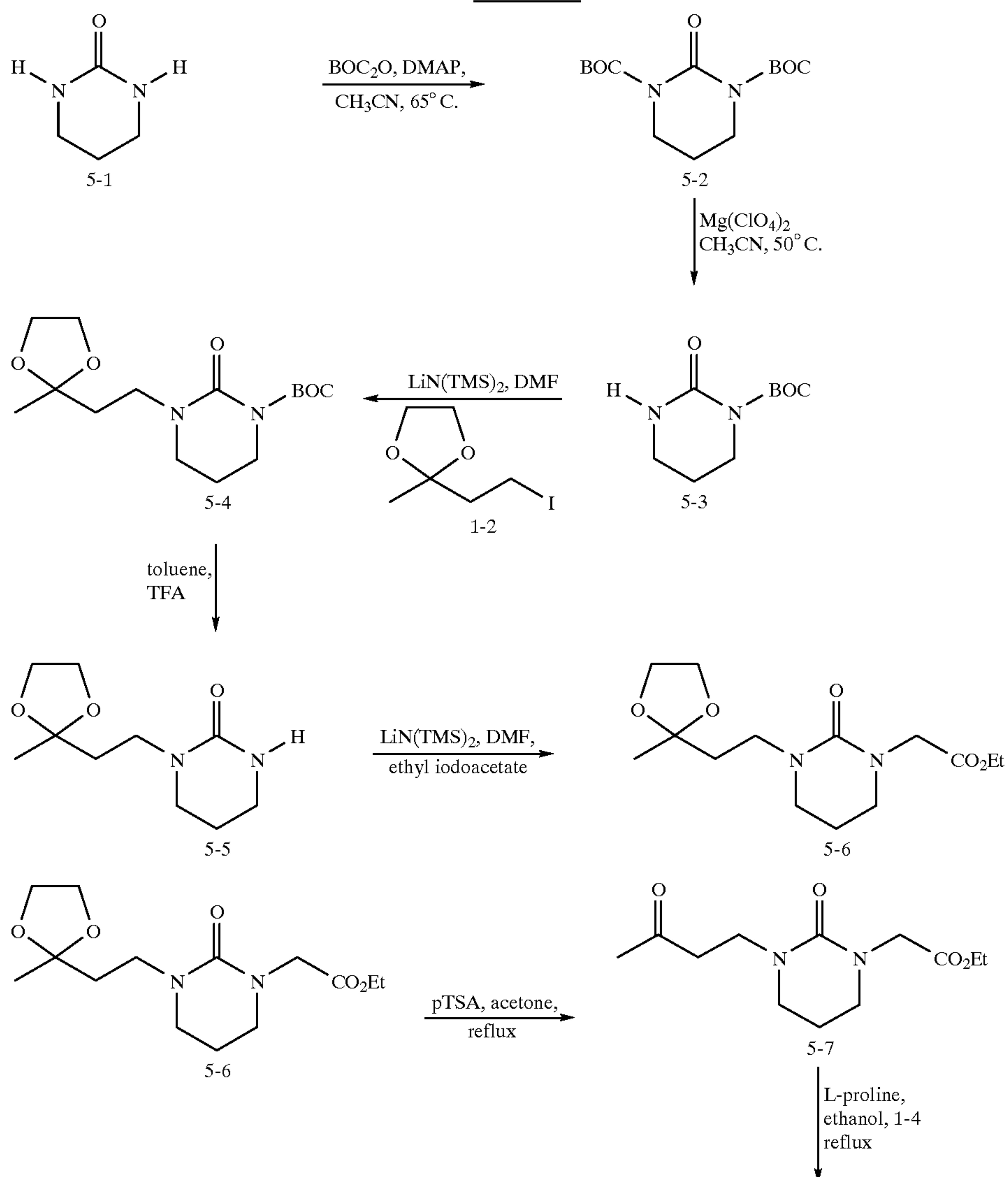
SCHEME 5
