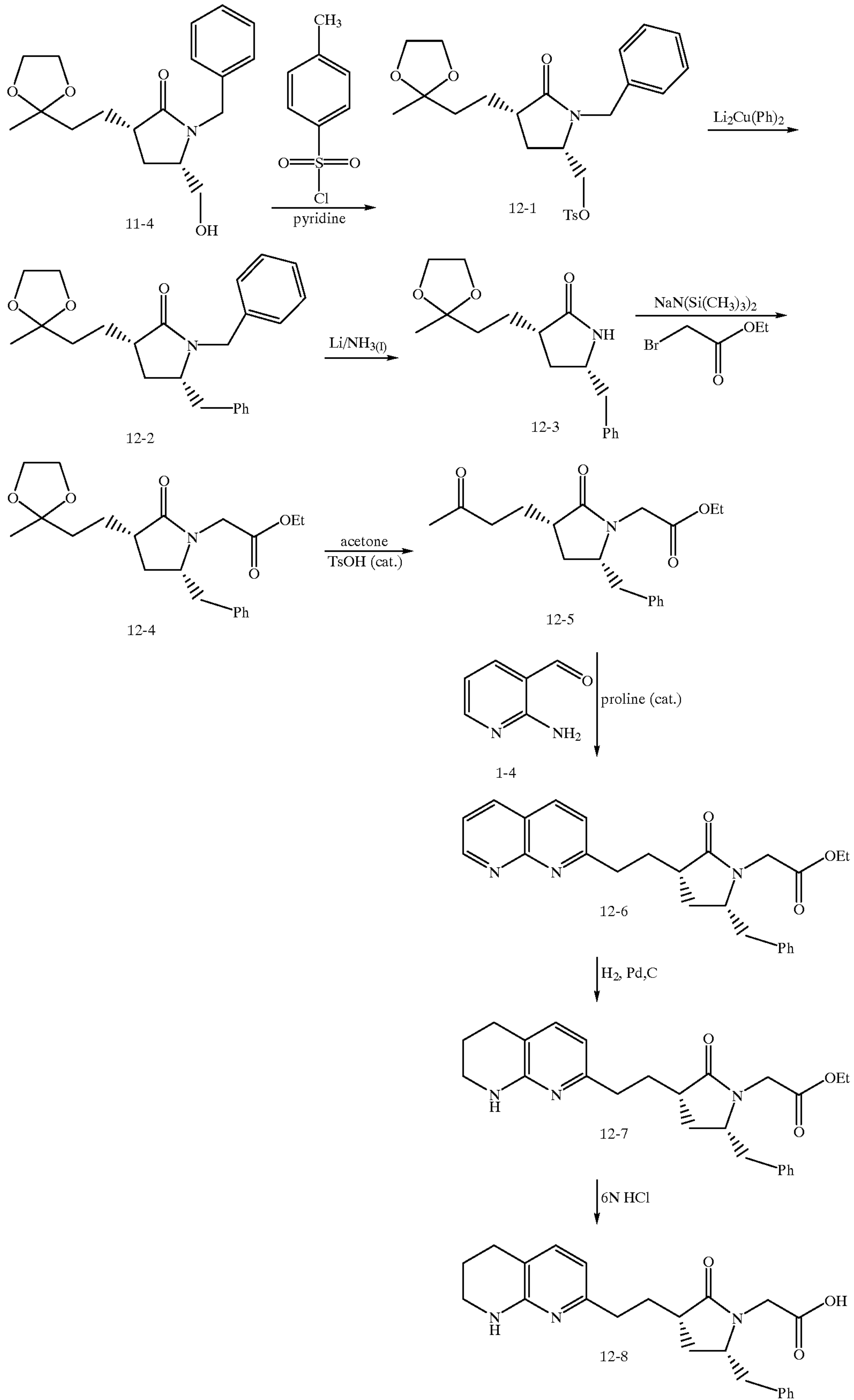
Scheme 12
