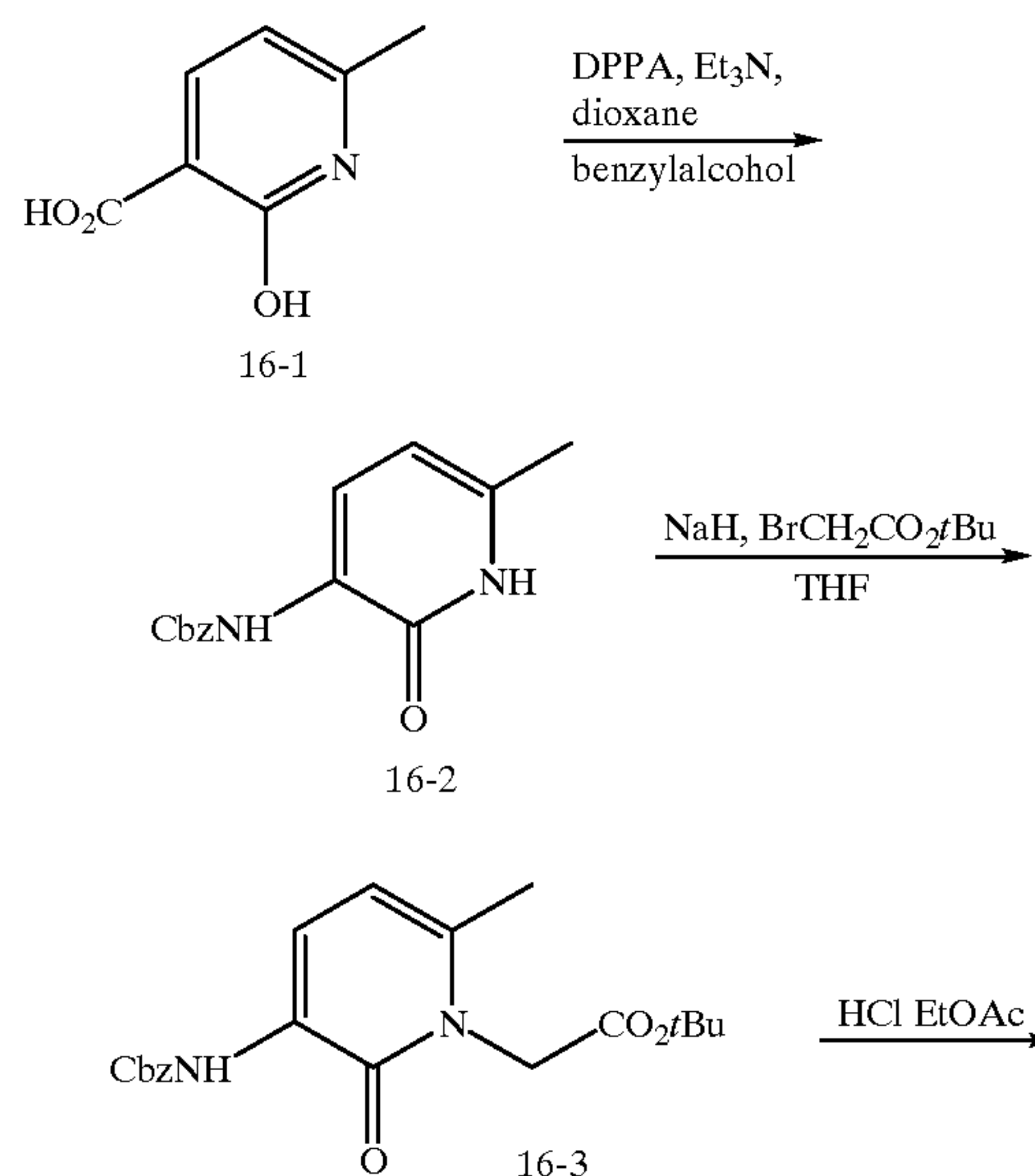
SCHEME 16
