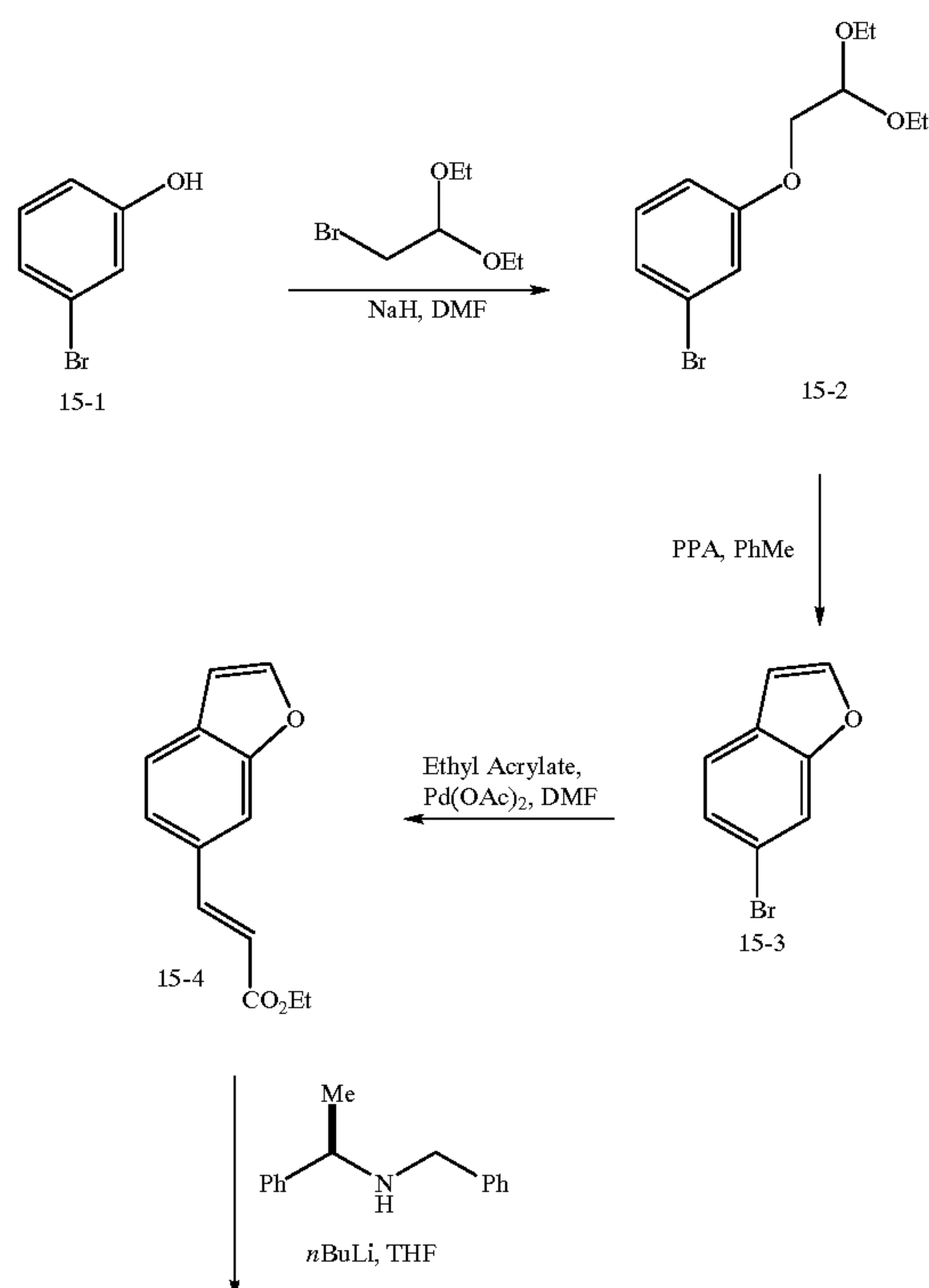
SCHEME 15
