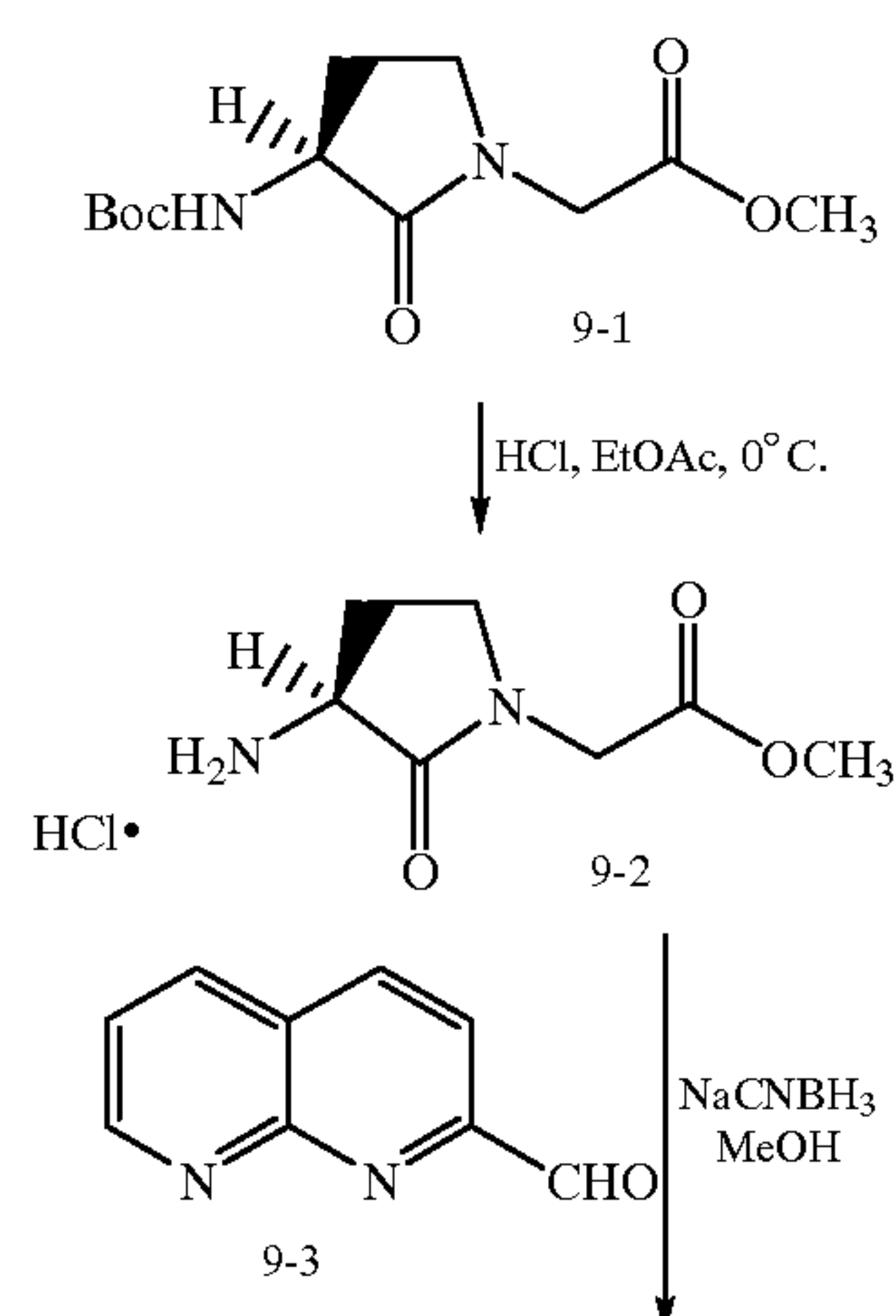
Scheme 9
