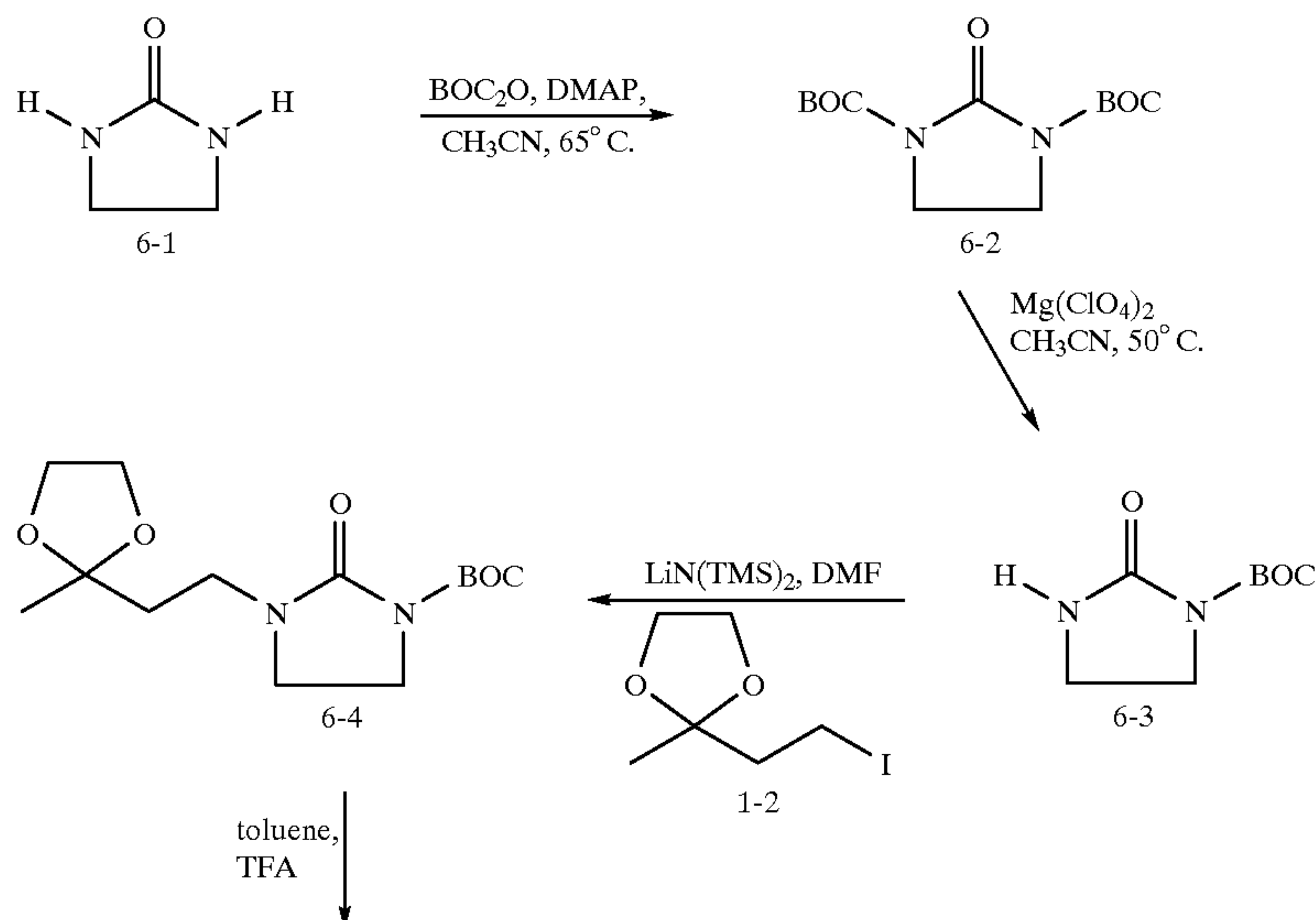
SCHEME 6
