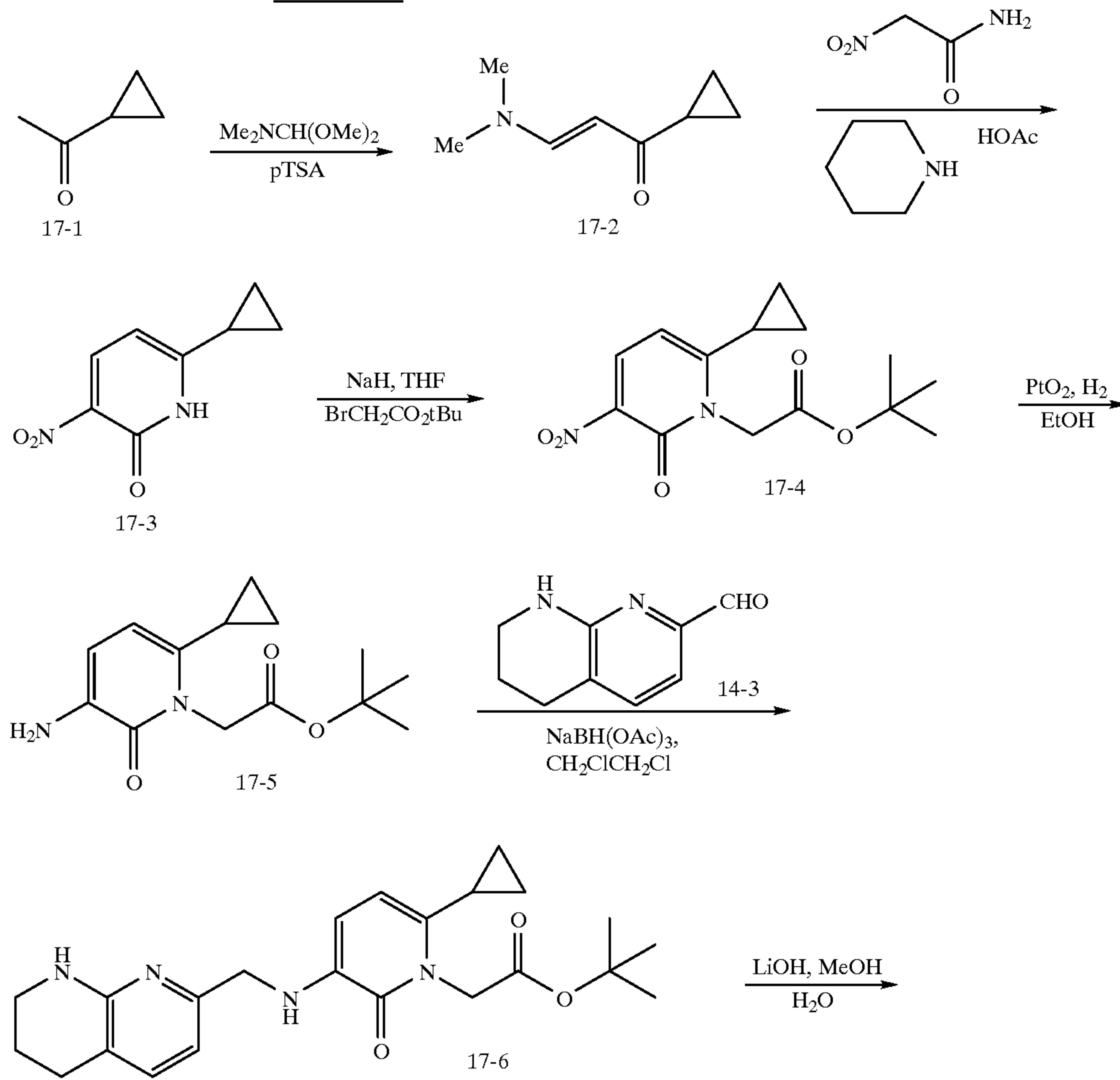
SCHEME 17
