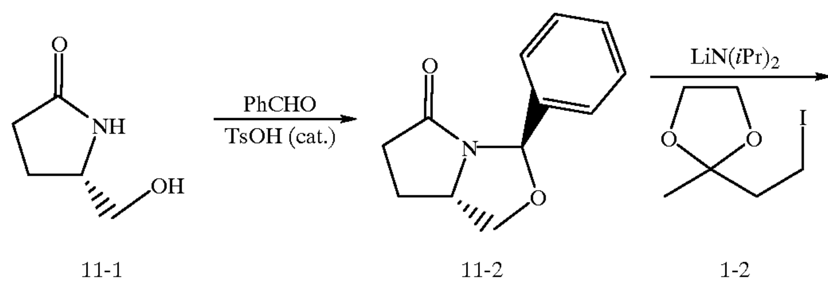
Scheme 11
