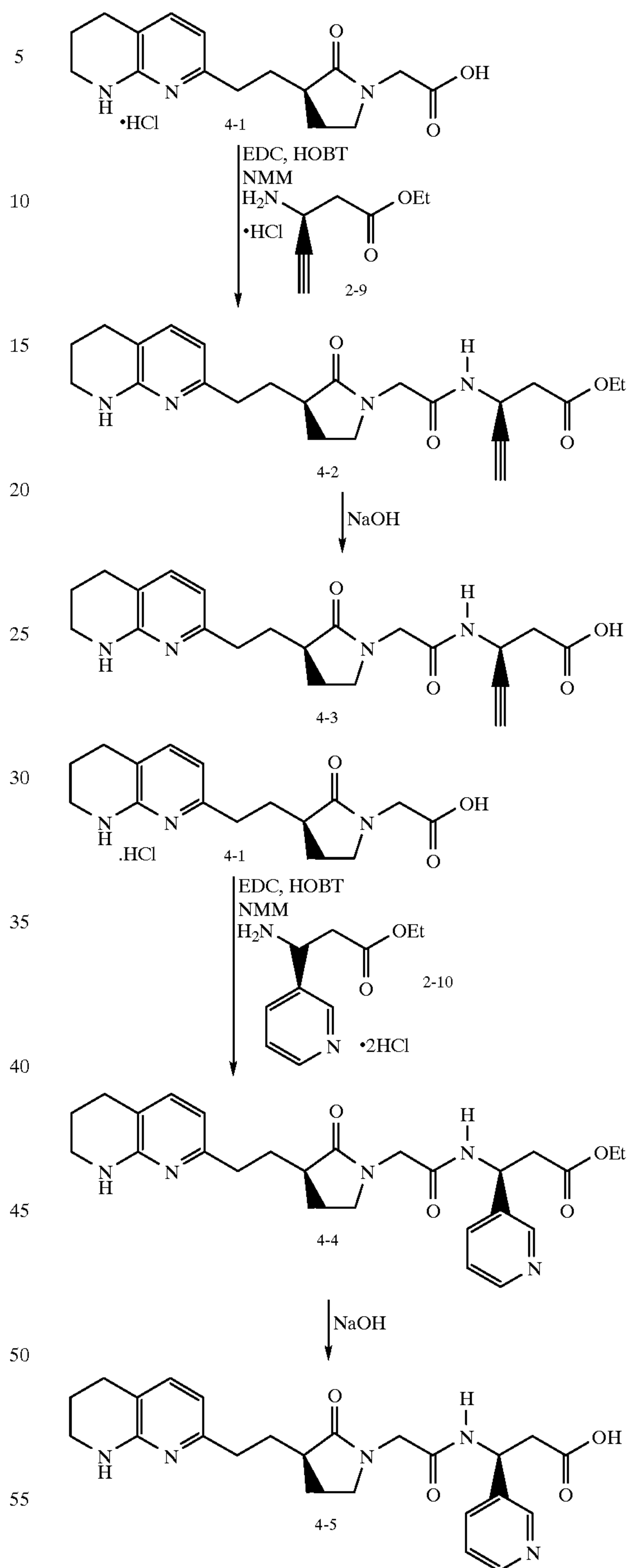
Scheme 4
