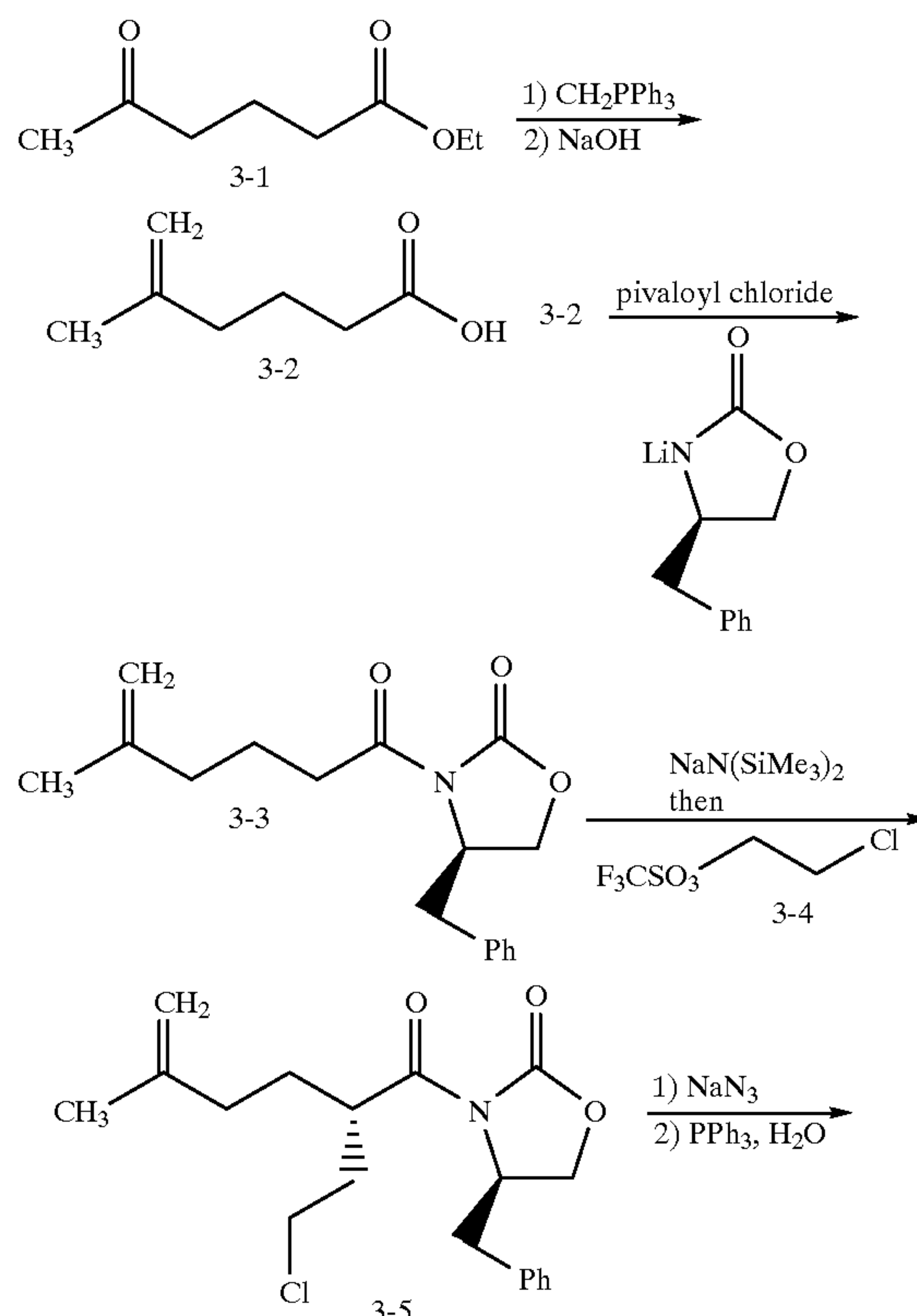
SCHEME 3
