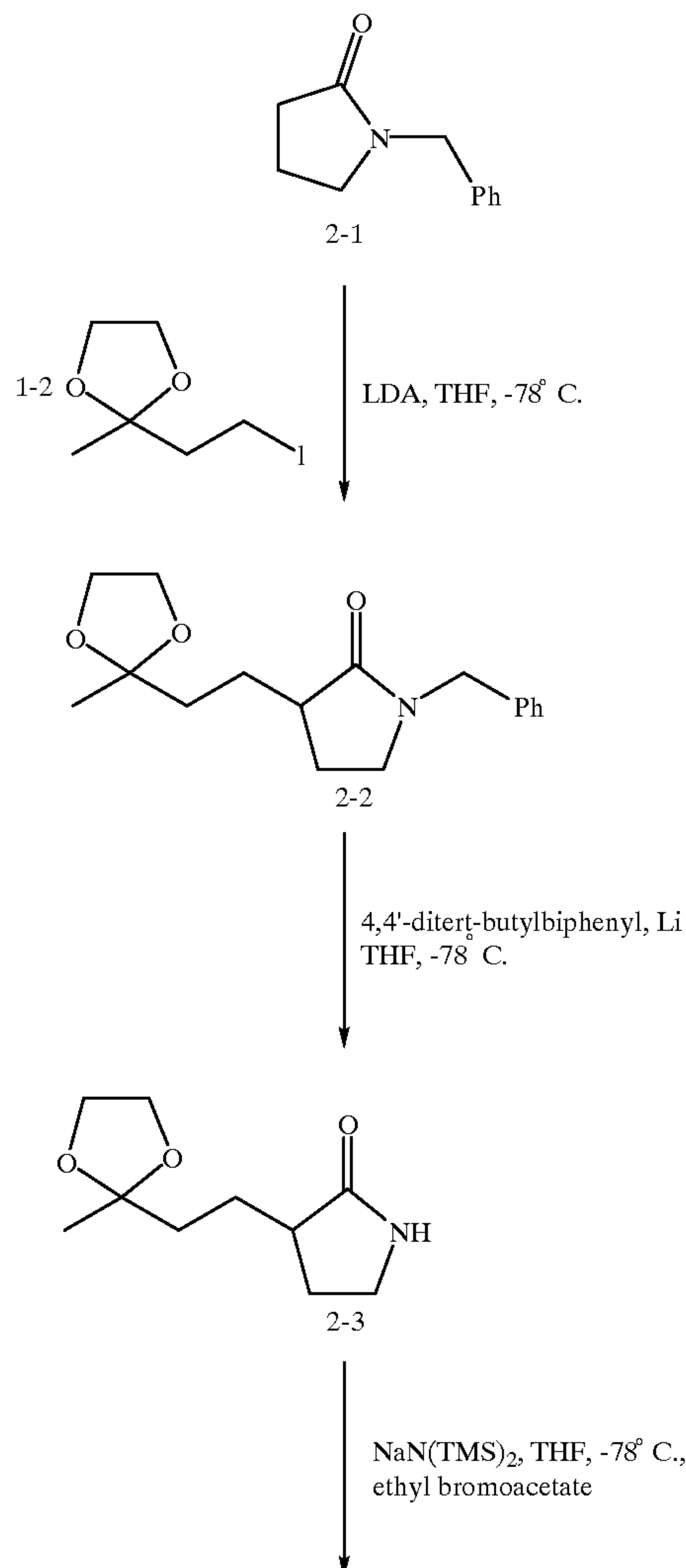
SCHEME 2
