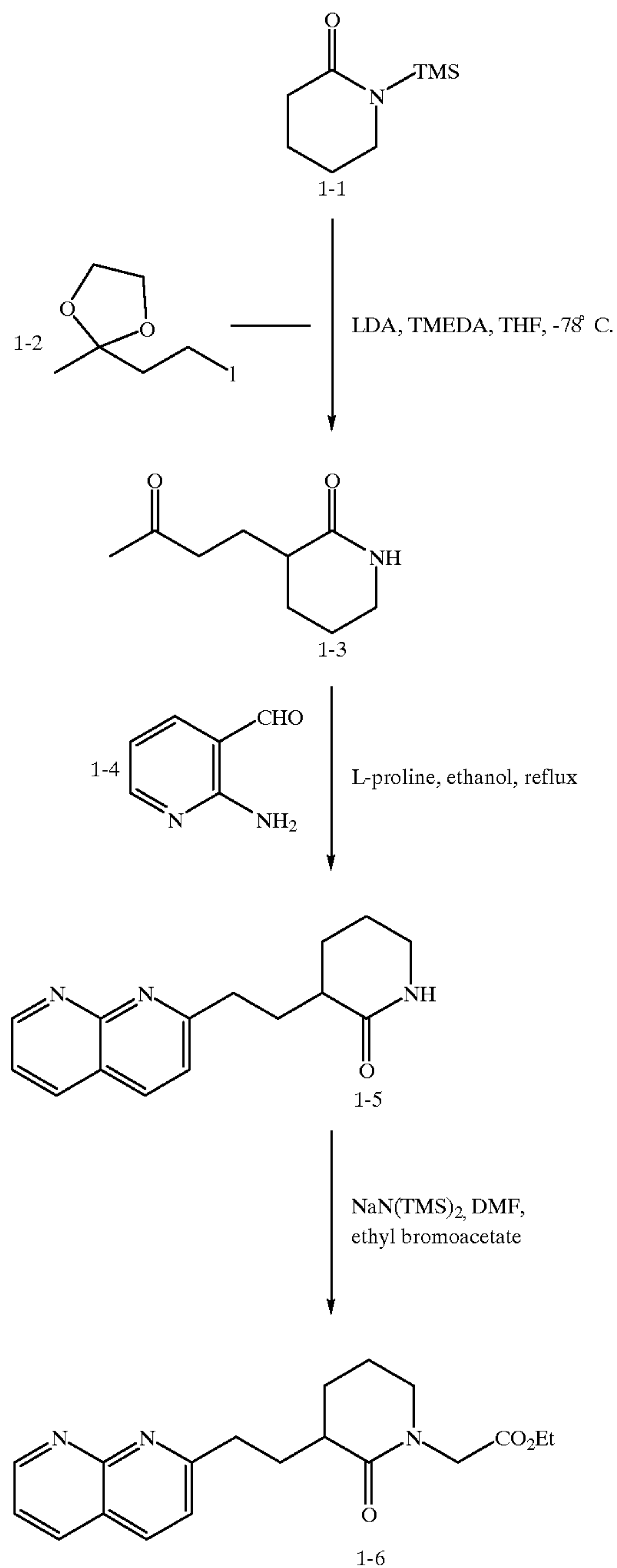
SCHEME 1
