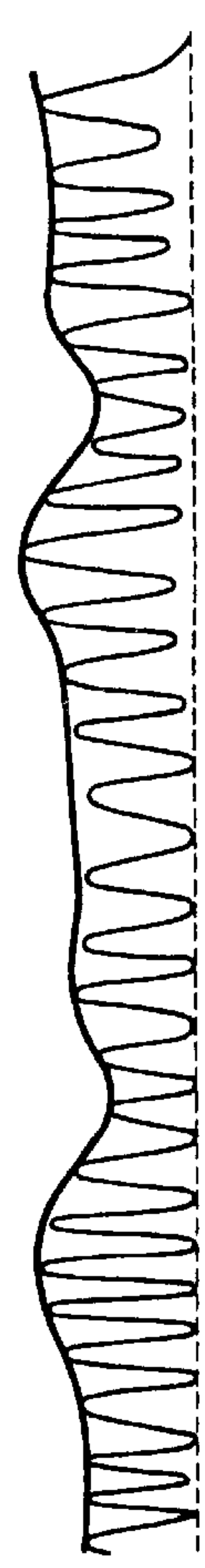
OUTPUT OF GAIN CONTROL CIRCUIT 81
