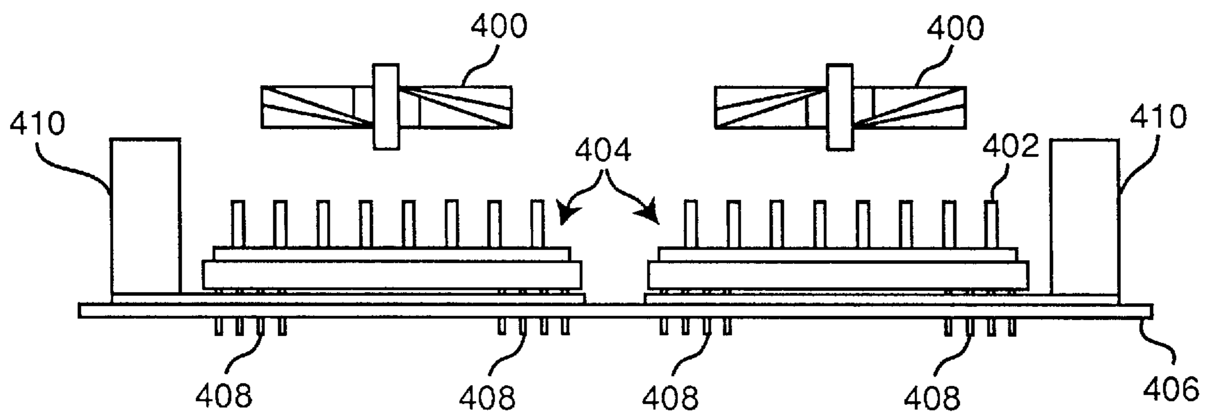
Figure 4 Prior Art
