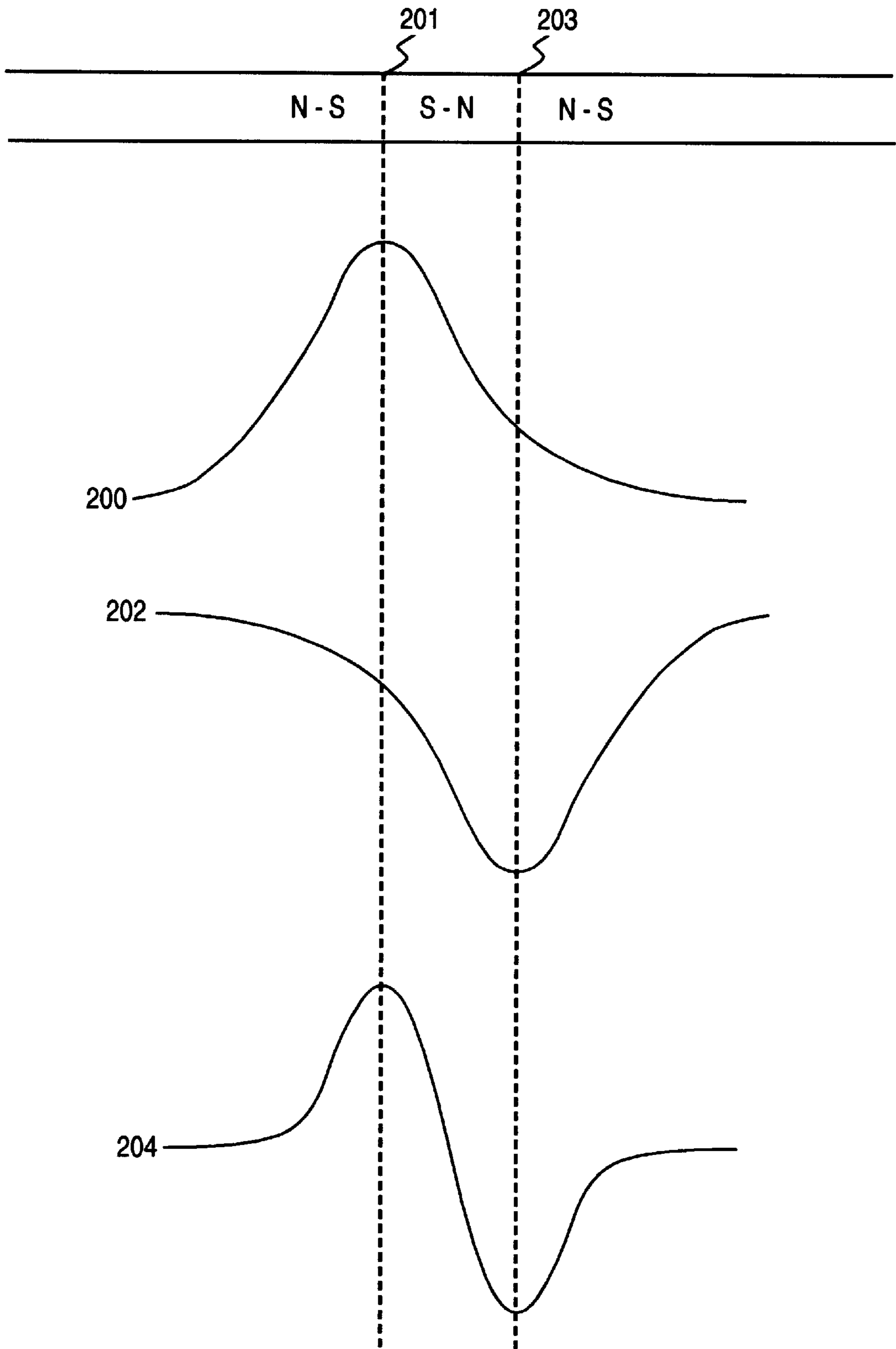
FIG. 2 (Prior Art)
