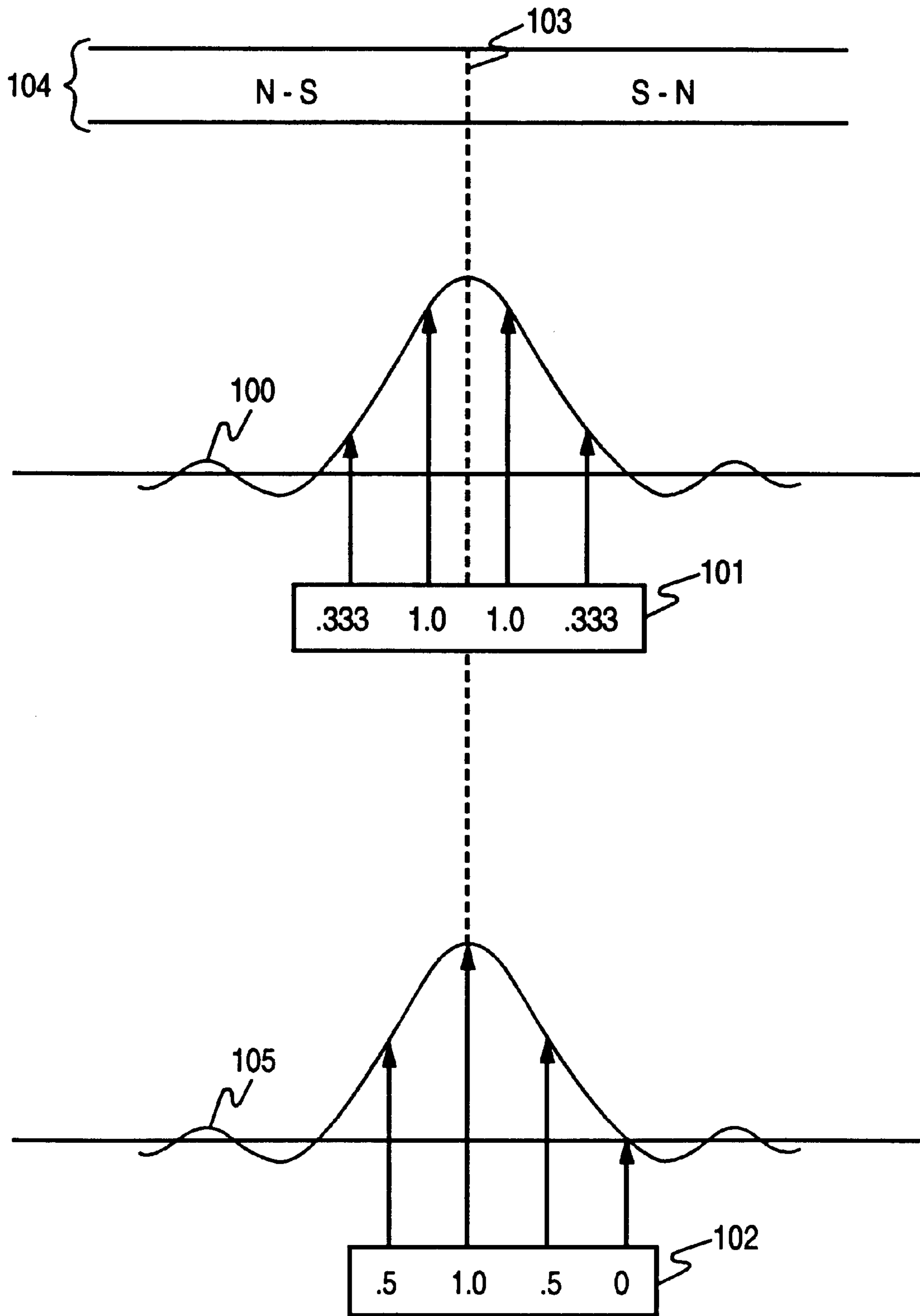
FIG. 1 (PRIOR ART)
