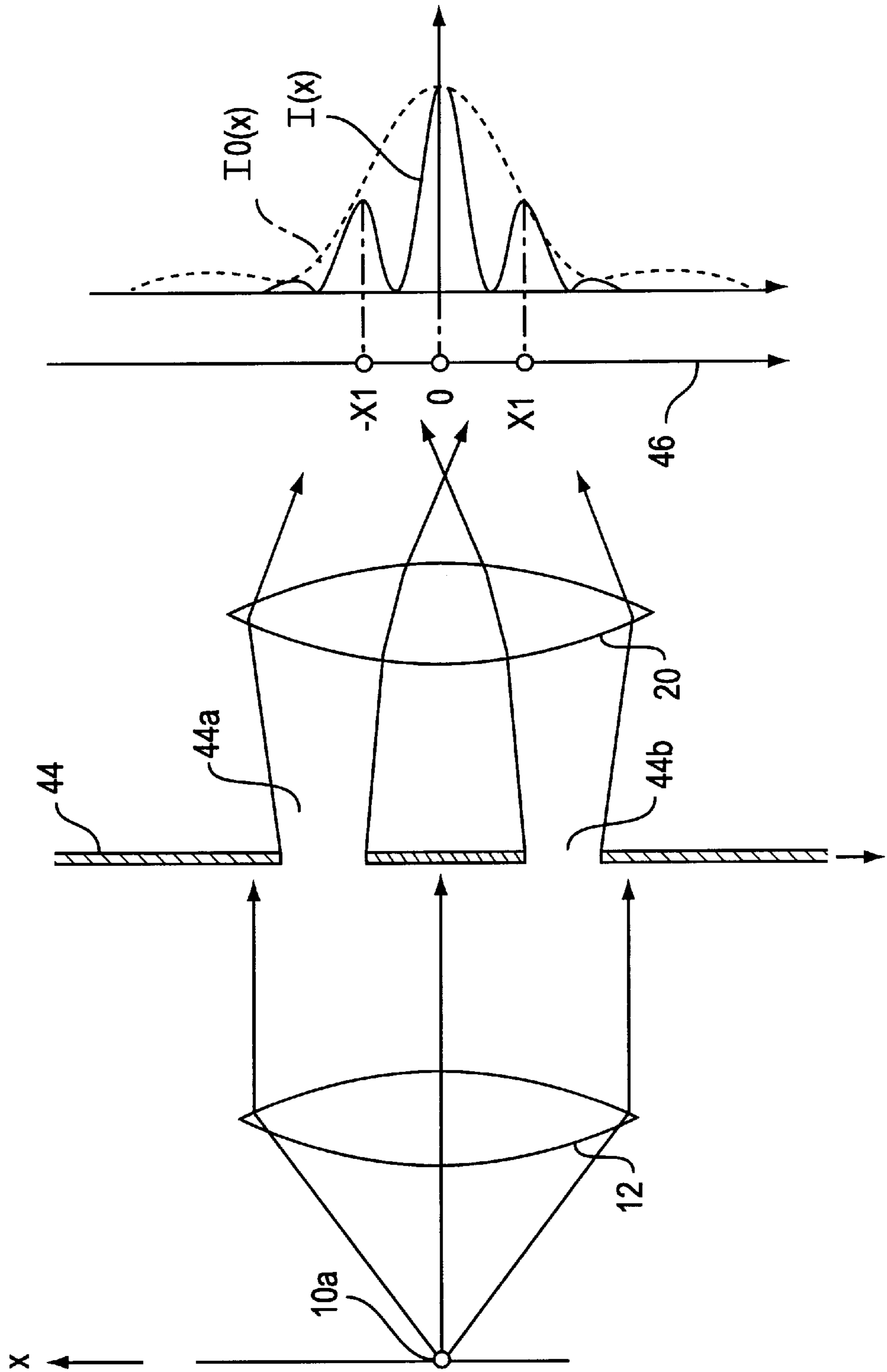
FIG. 20 PRIOR ART
