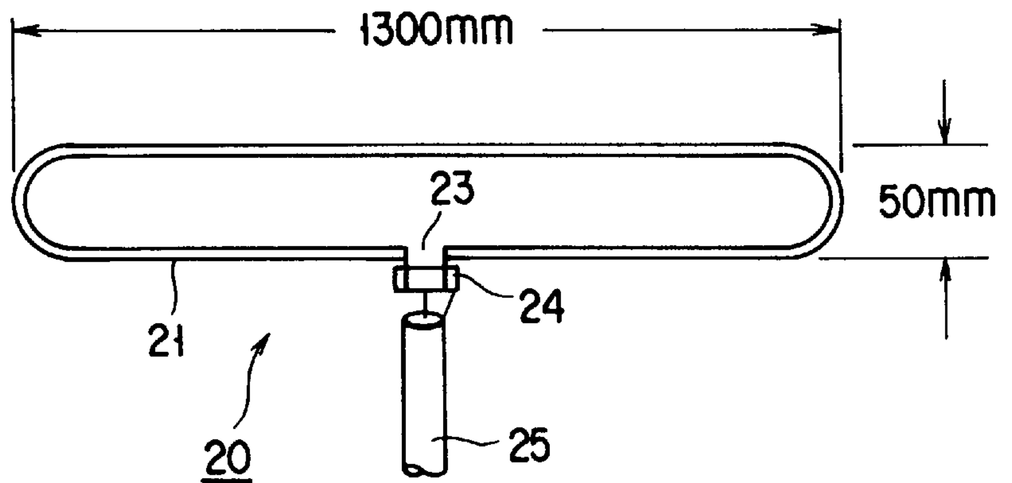
FIG. 21 (PRIOR ART)
