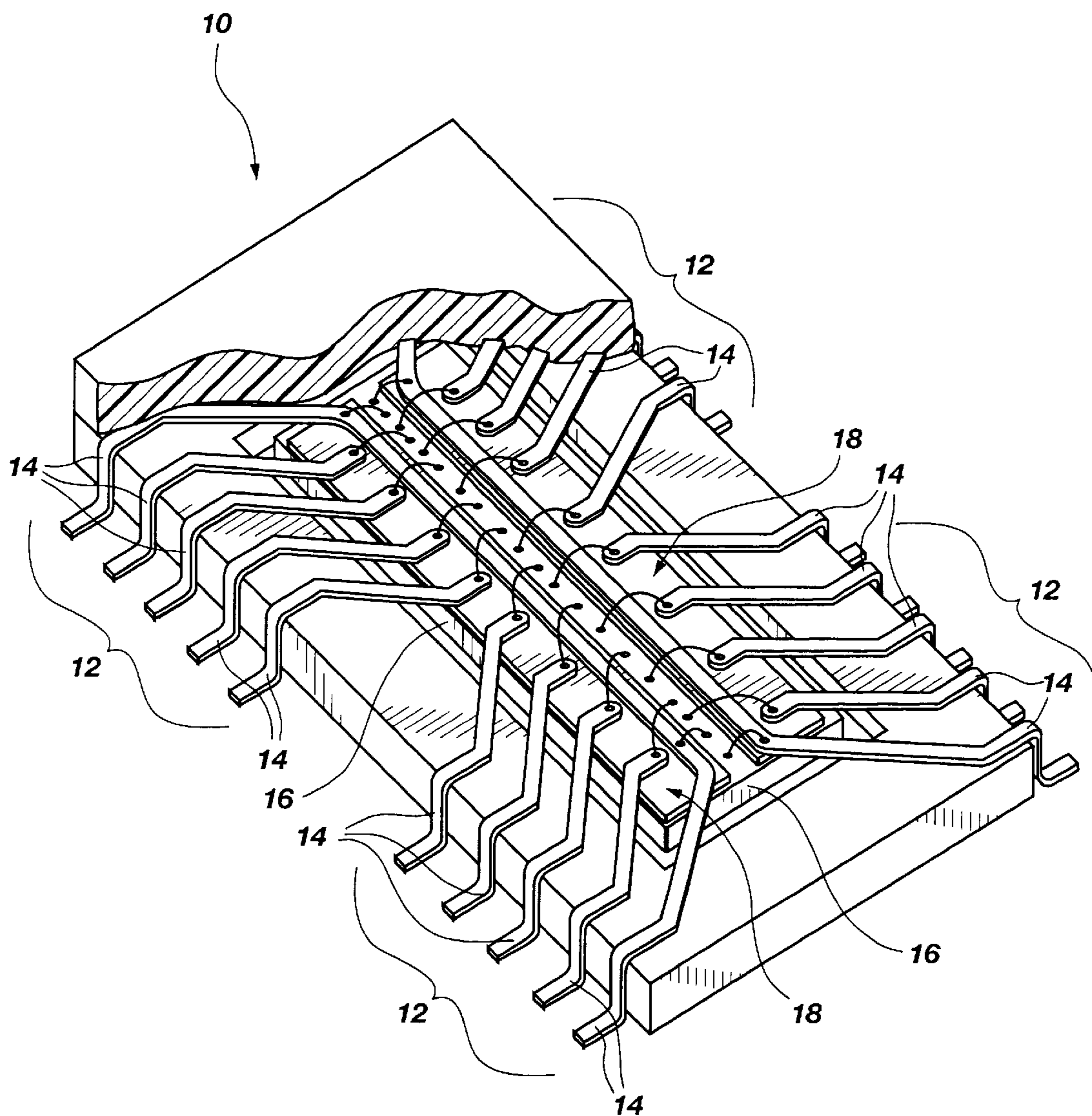
Fig. 1 (PRIOR ART)
