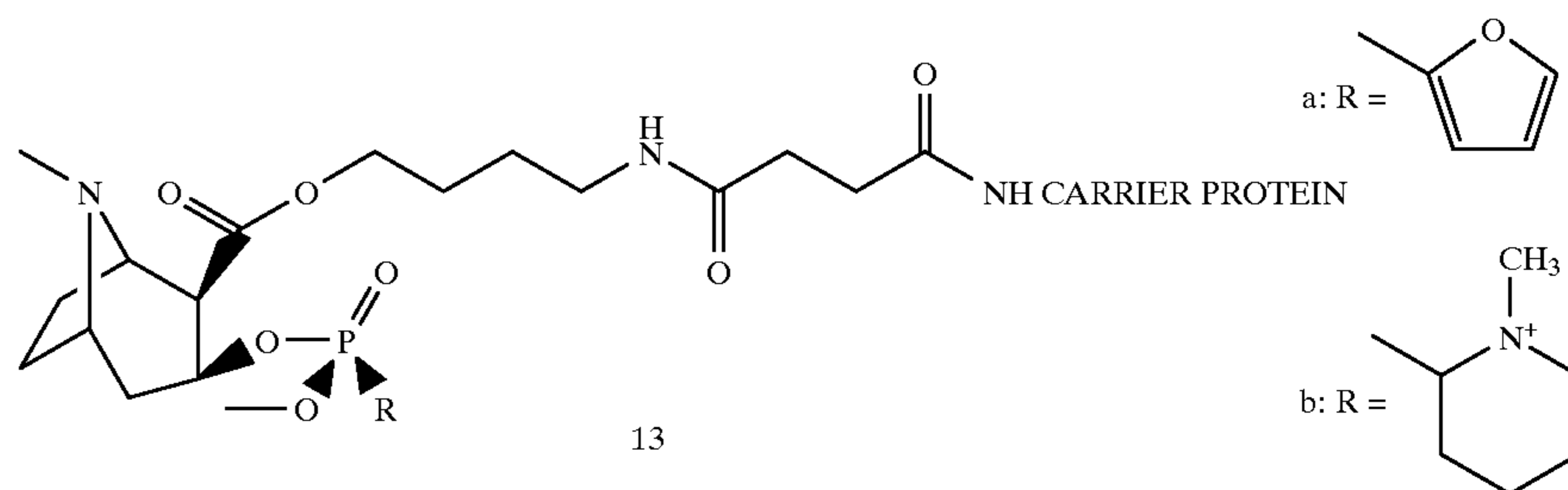
SCHEME IX
