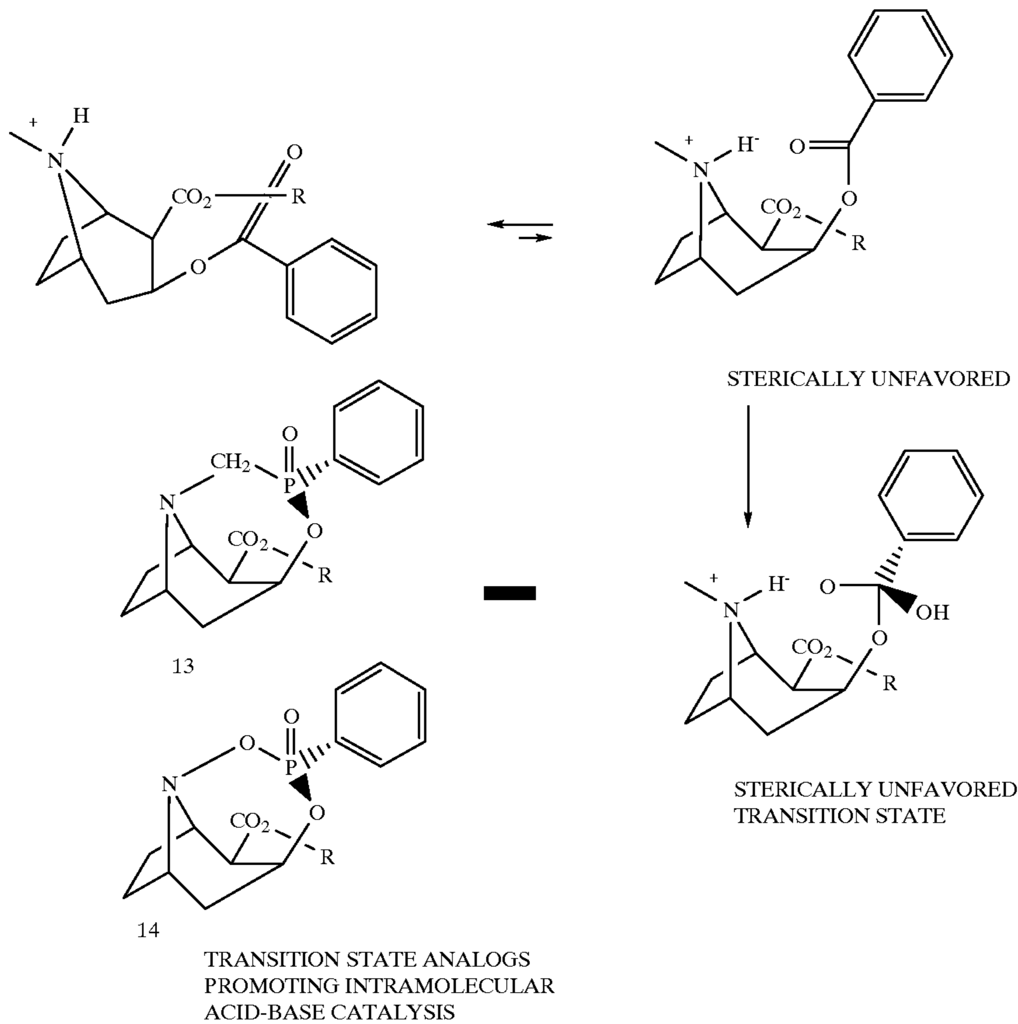
SCHEME X
