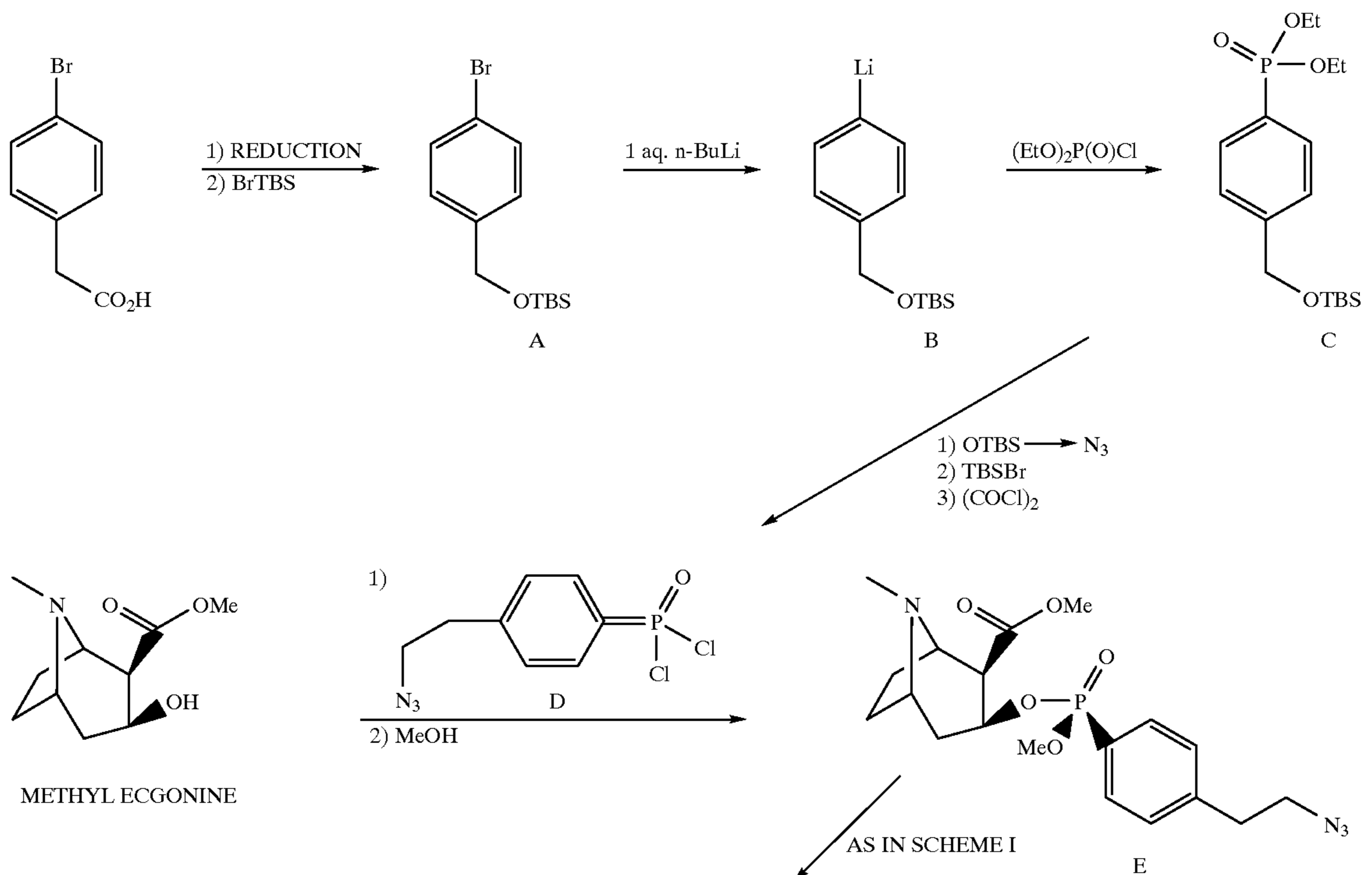
SCHEME VIII
