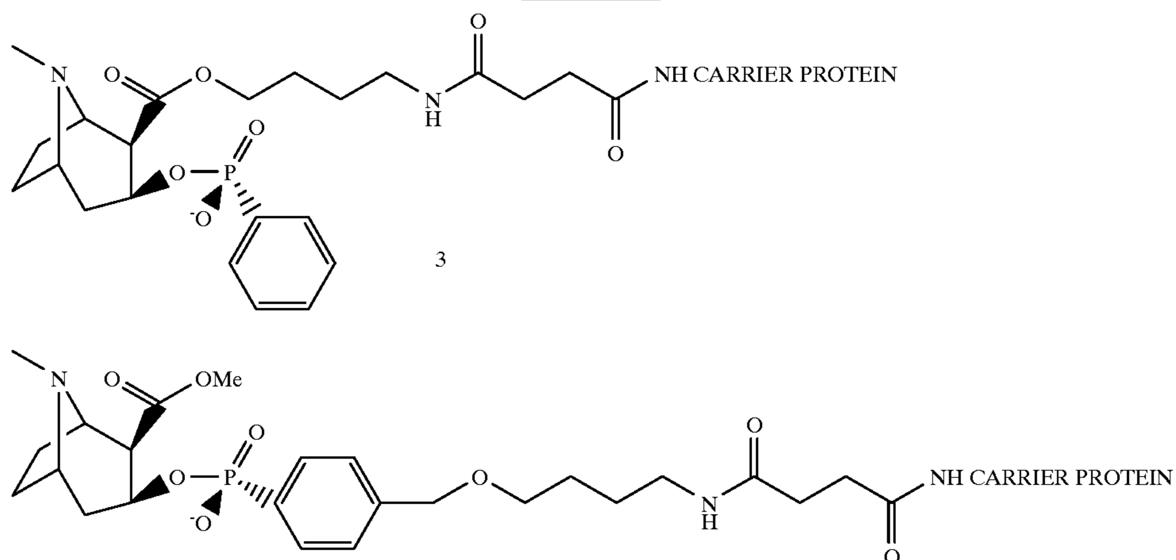
SCHEME VII
