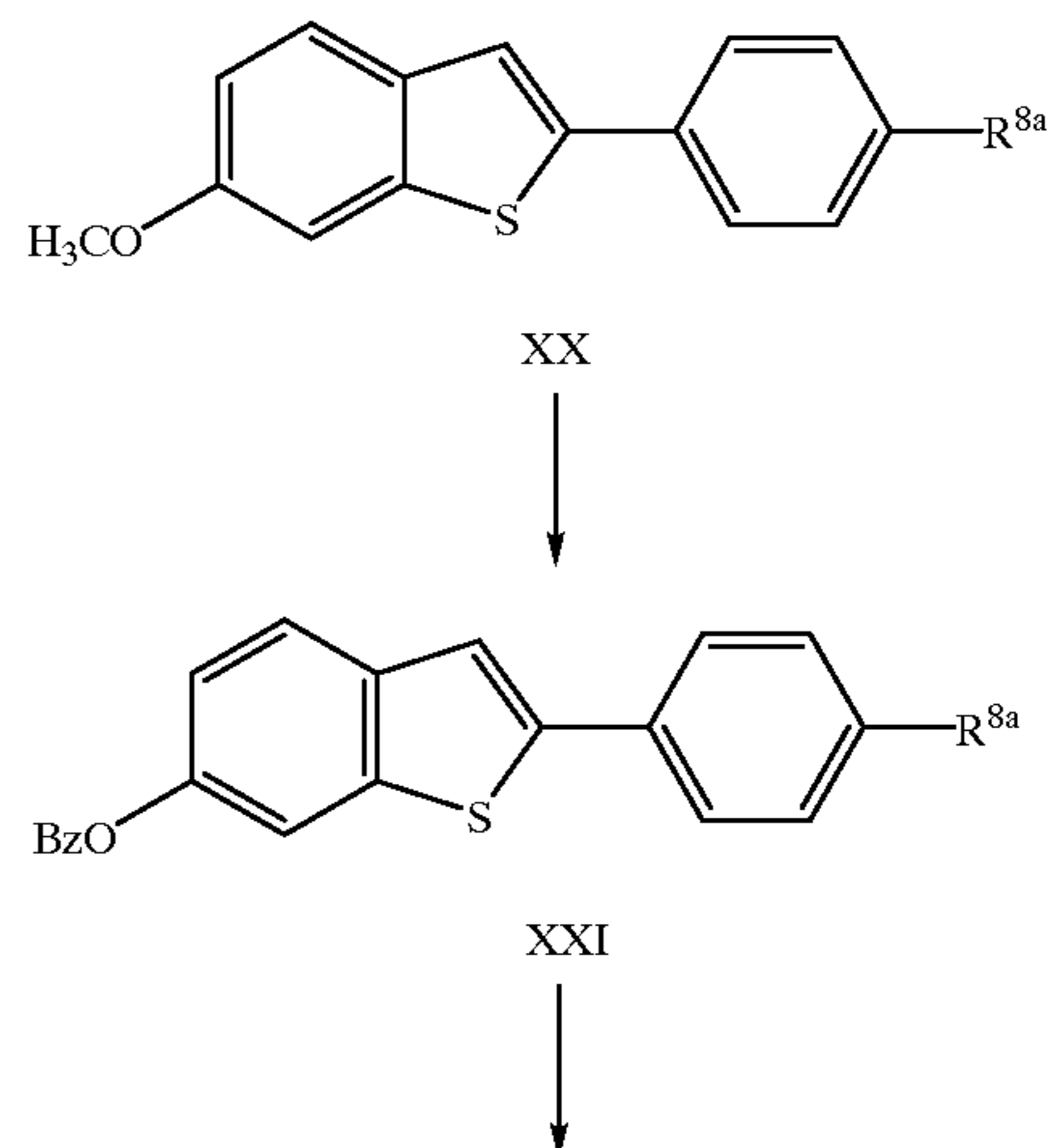
Scheme VII
