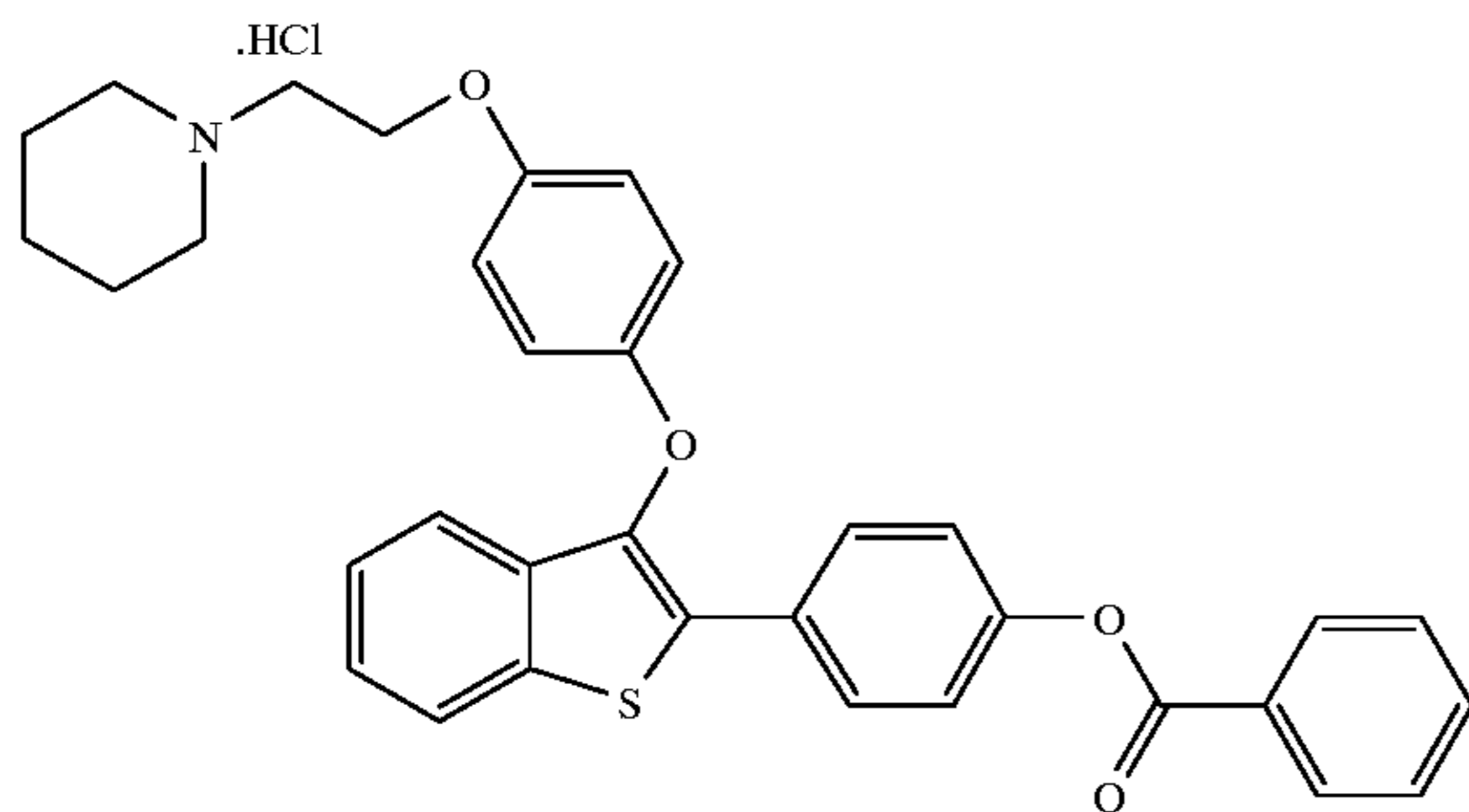
3-[4-[2-(1-piperidinyl)ethoxy]phenoxy]-2-(4-benzoyloxyphenyl)benzo[b]thiophene hydrochloride
