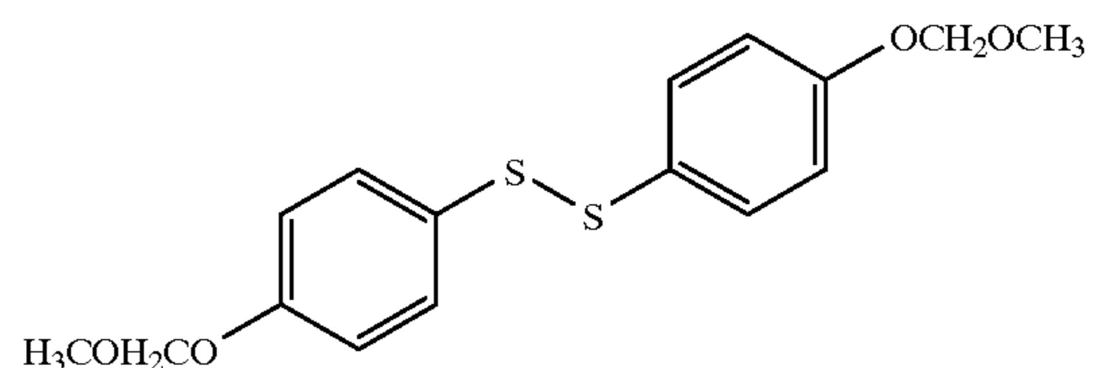
[6-Hydroxy-3-[4-[2-(1-piperidinyl)ethoxy]thiophenoxy]-2-(4-hydroxyphenyl)]benzo[b]thiophene
