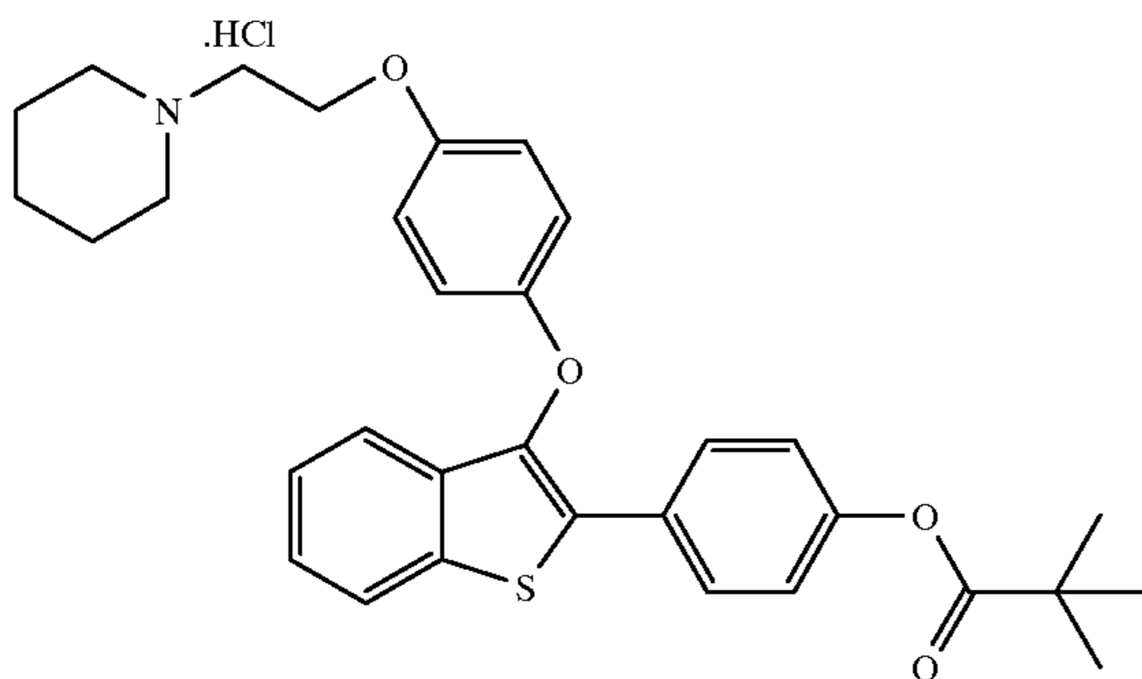
3-[4-[2-(1-piperidinyl)ethoxy]phenoxy]-2-(4-pivaloyloxyphenyl)benzo[b]thiophene hydrochloride
