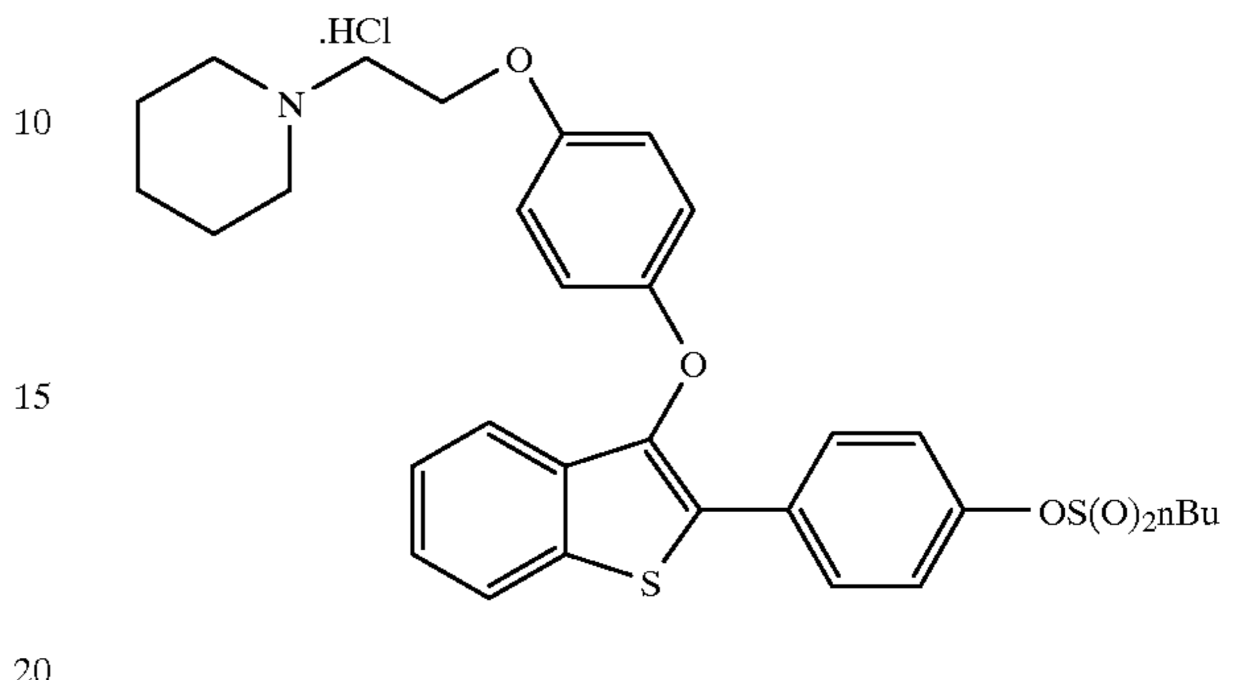
3-[4-[2-(1-piperidinyl)ethoxy]phenoxy]-2-(4-butylsulfonyloxyphenyl)benzo[b]thiophene hydrochloride
