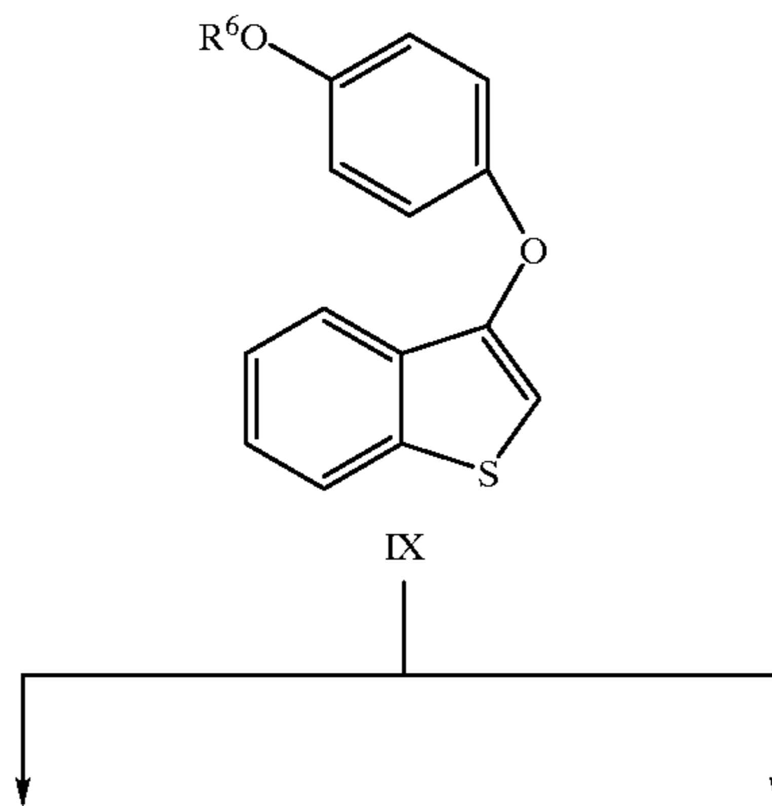
Scheme IV
