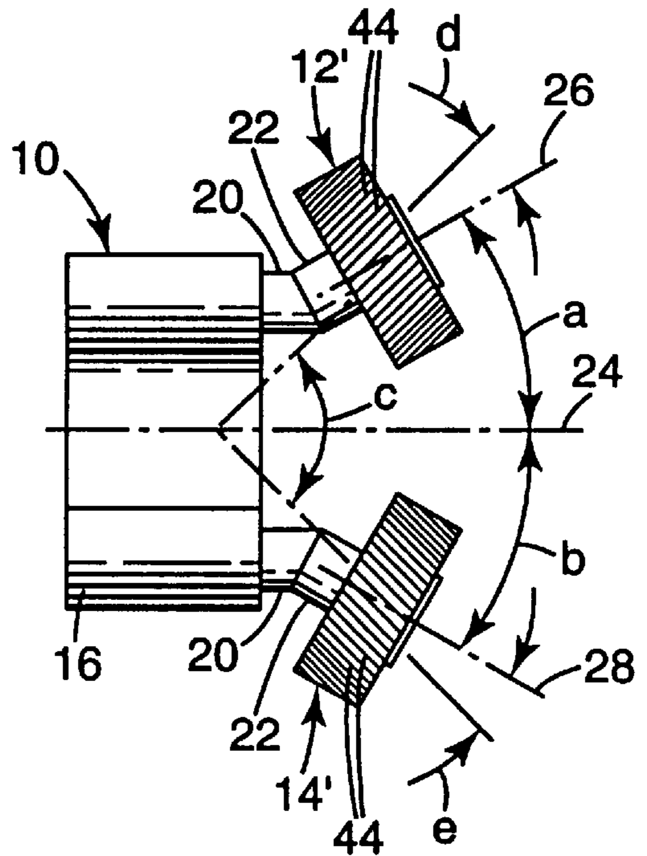
Fig. 4 PRIOR ART
