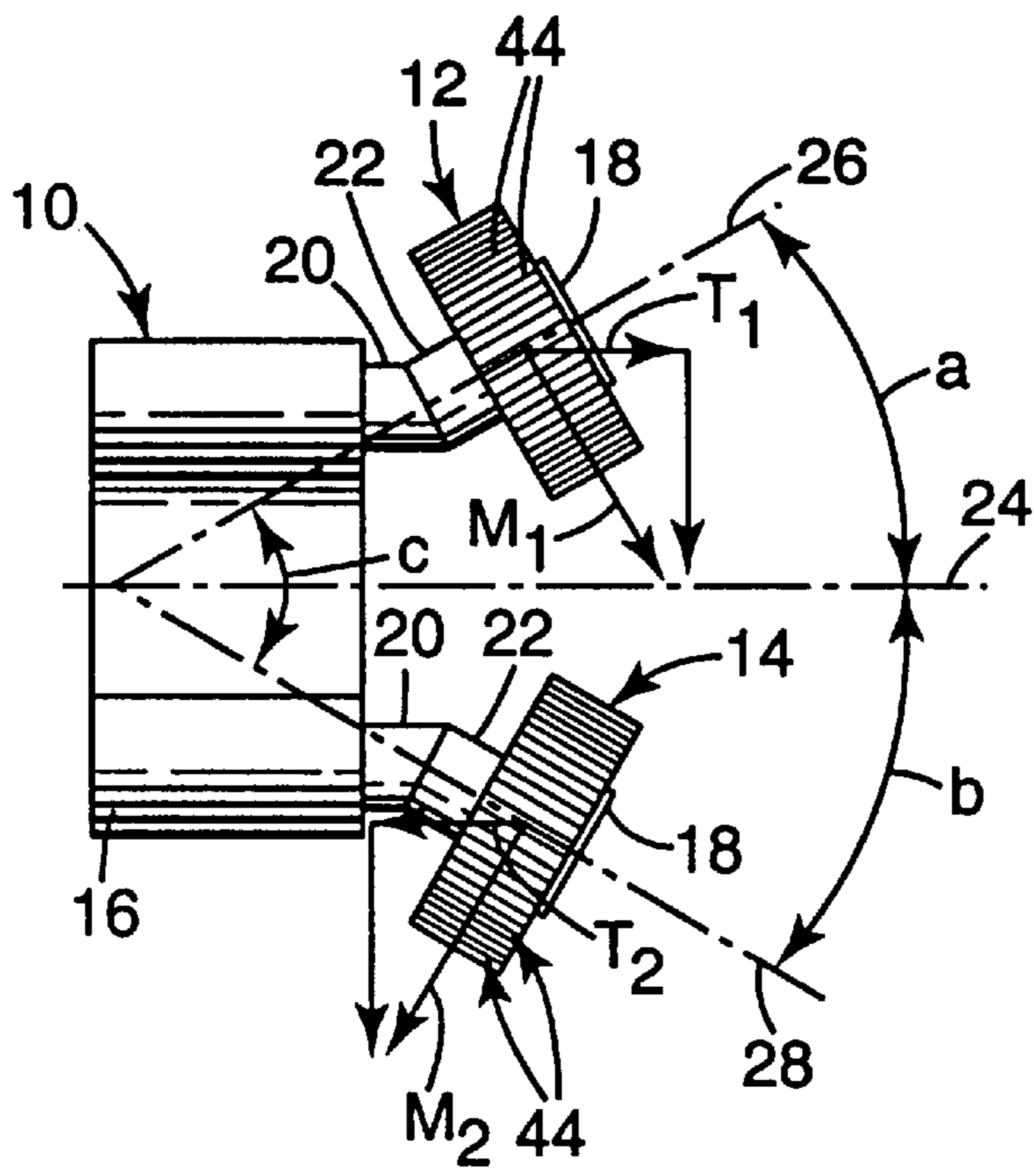
Fig. 3 PRIOR ART
