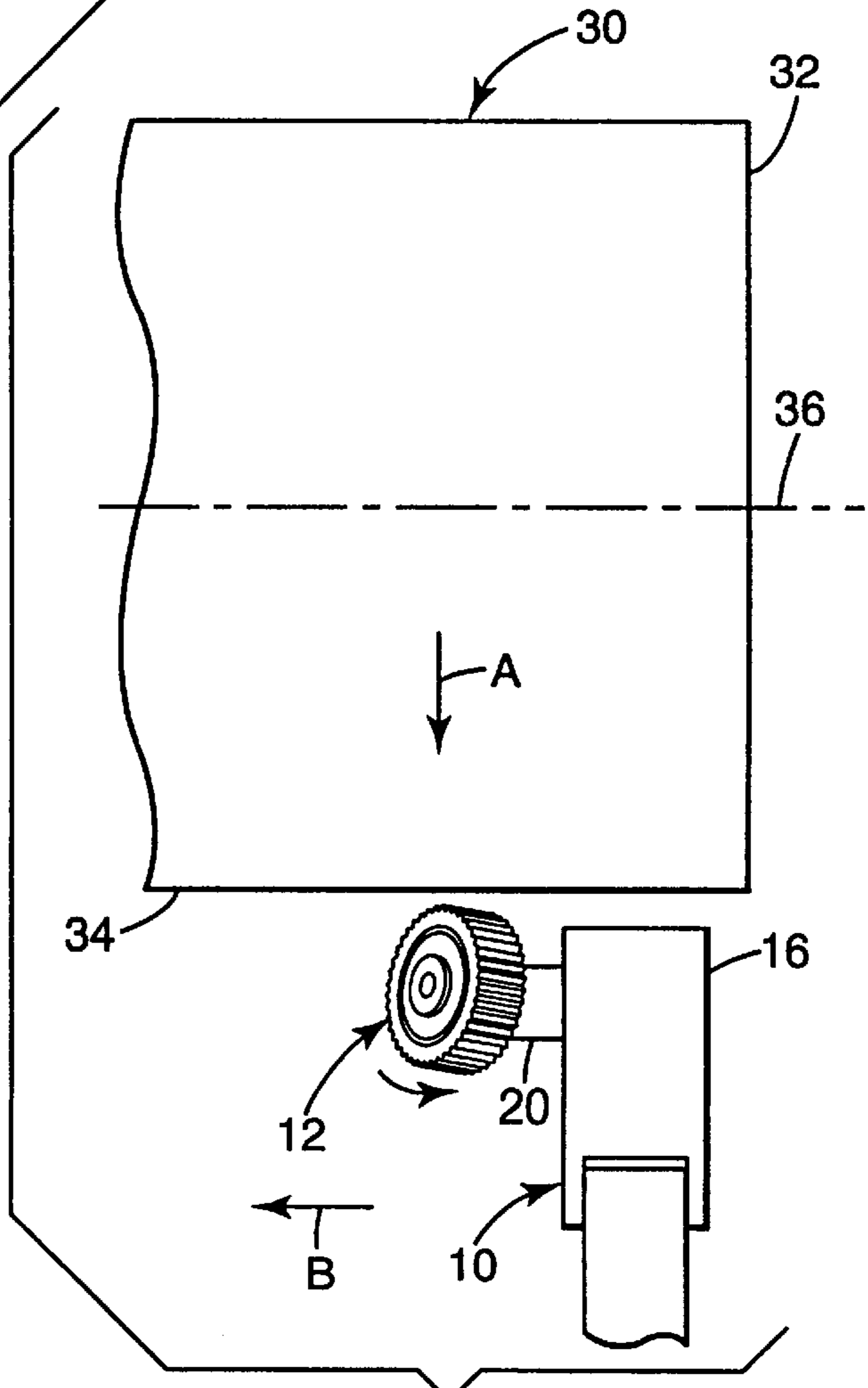
Fig. 2 PRIOR ART
