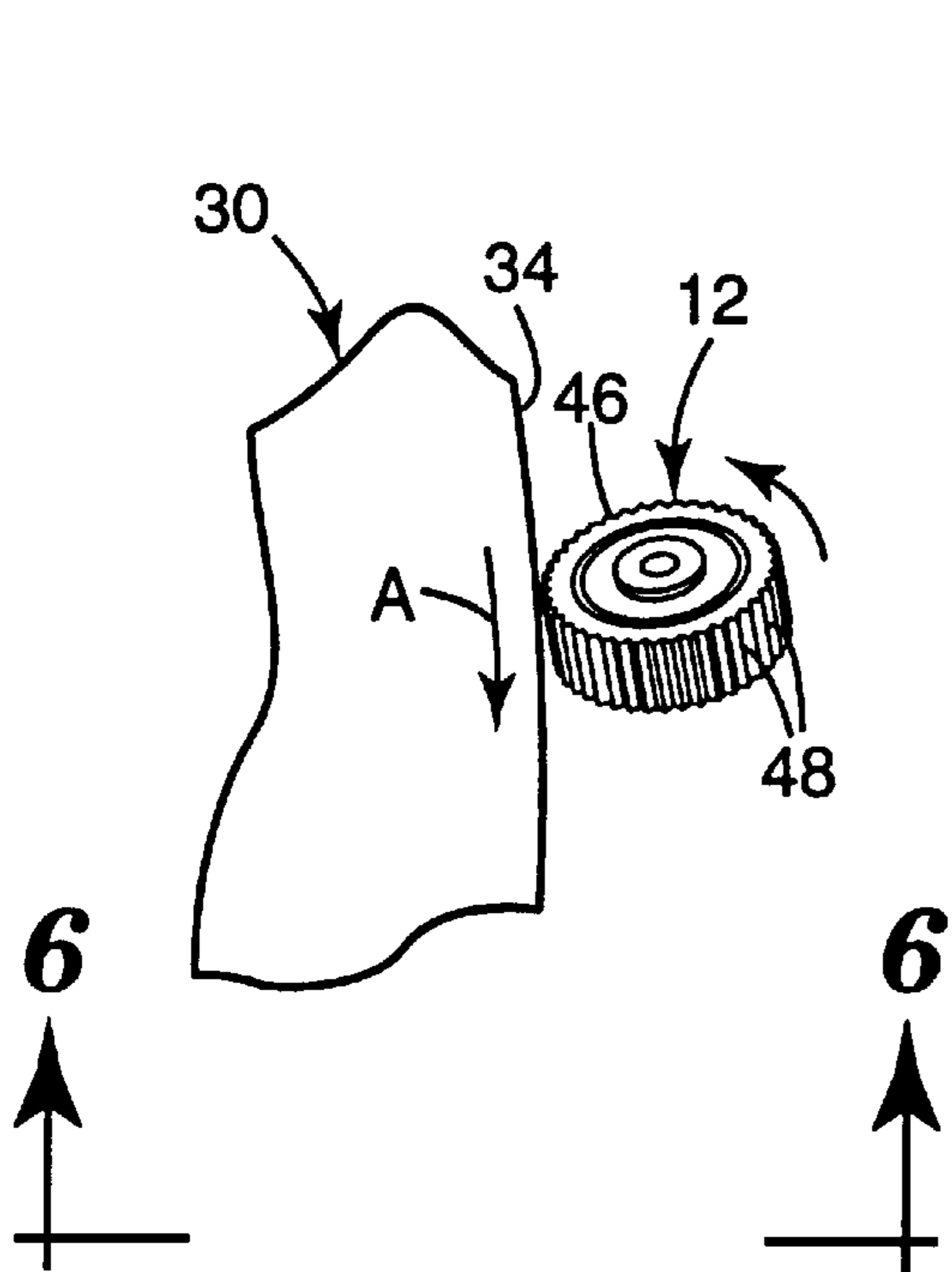
Fig. 5 PRIOR ART
