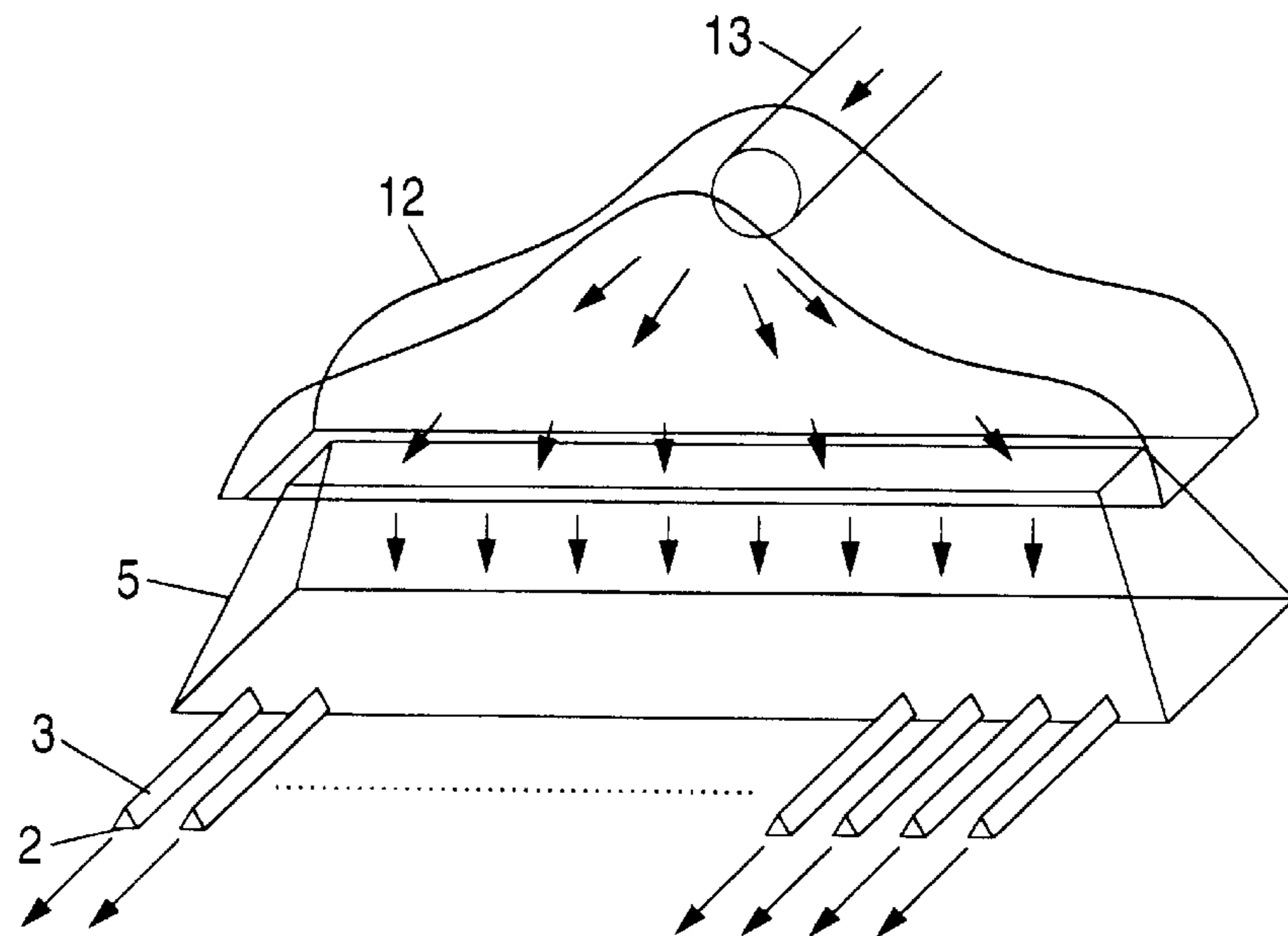
FIG. 19 PRIOR ART
