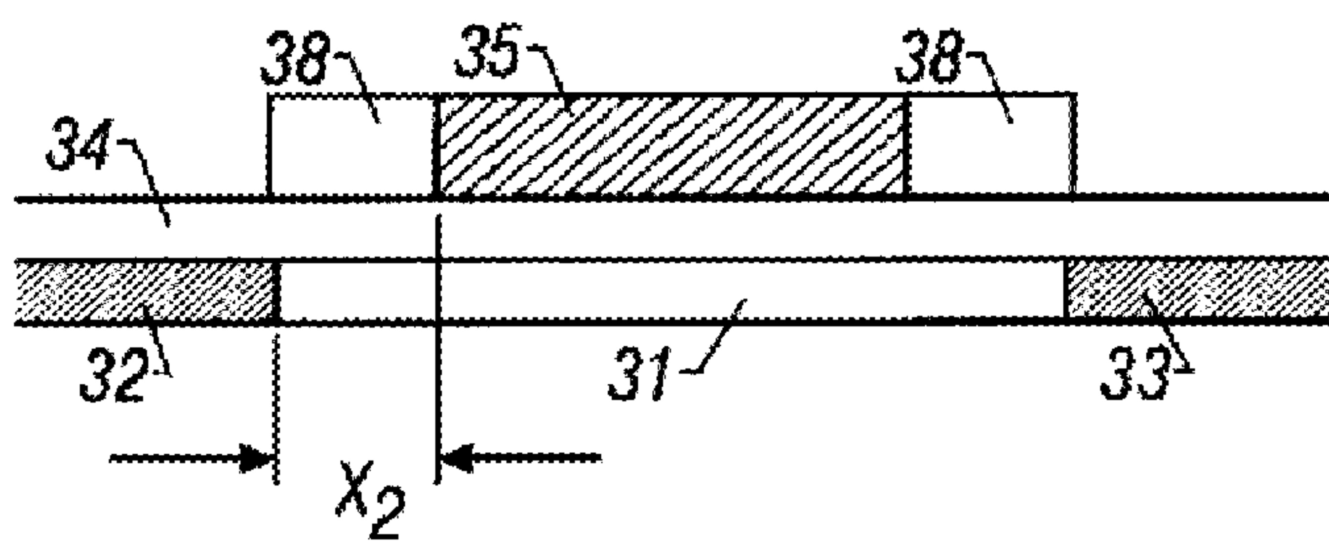
FIG. 3C (Prior Art)
