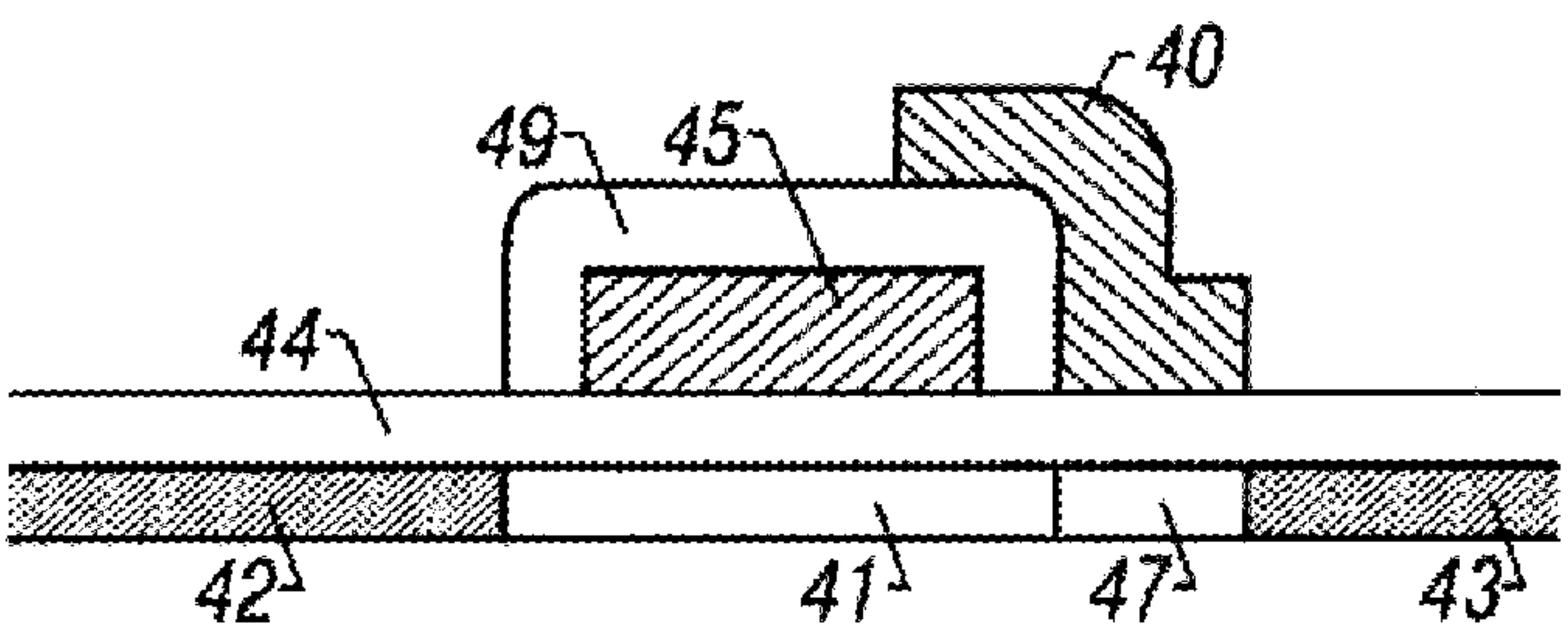
FIG. 4 (Prior Art)
