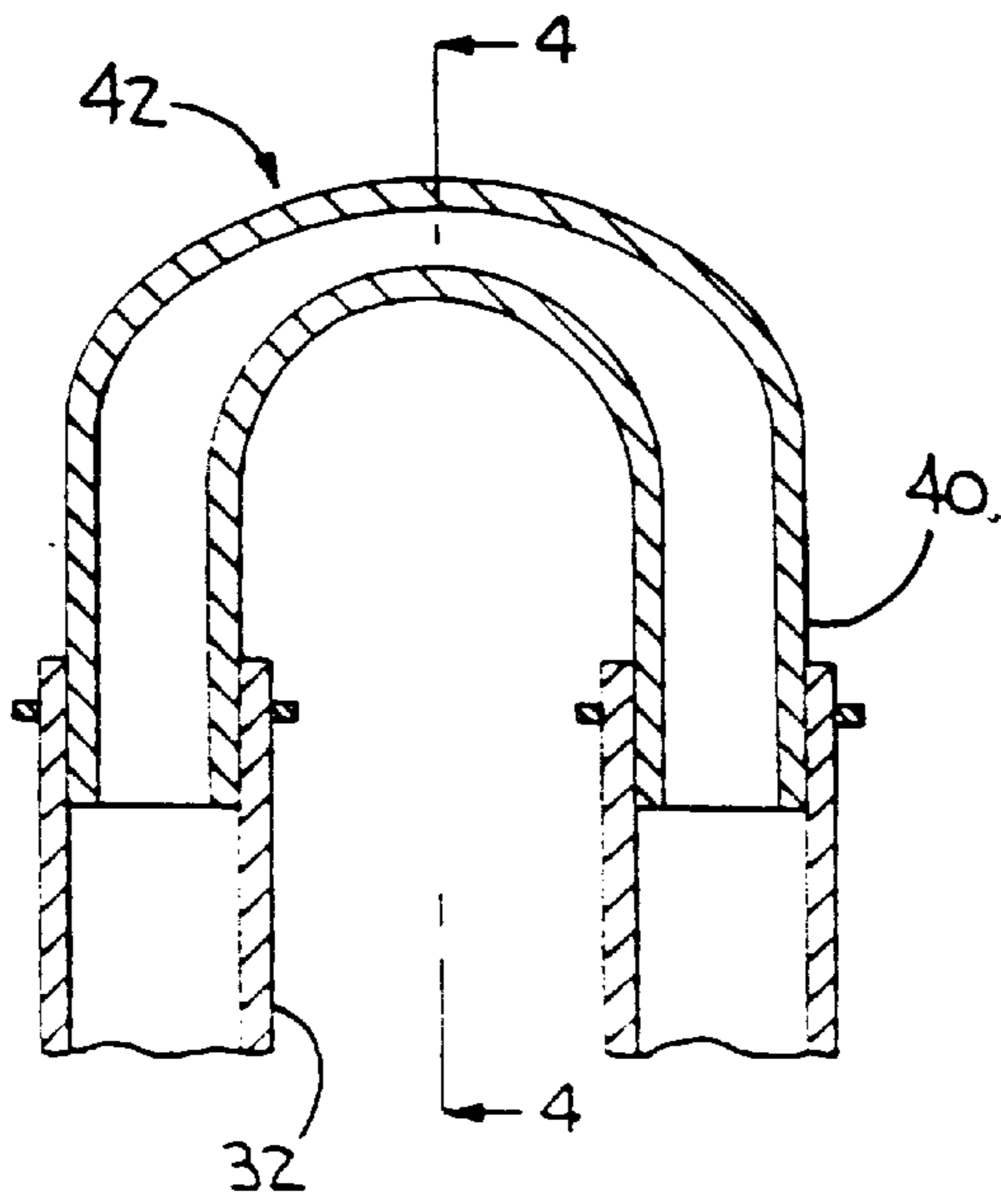
FIG. 3 (PRIOR ART)
