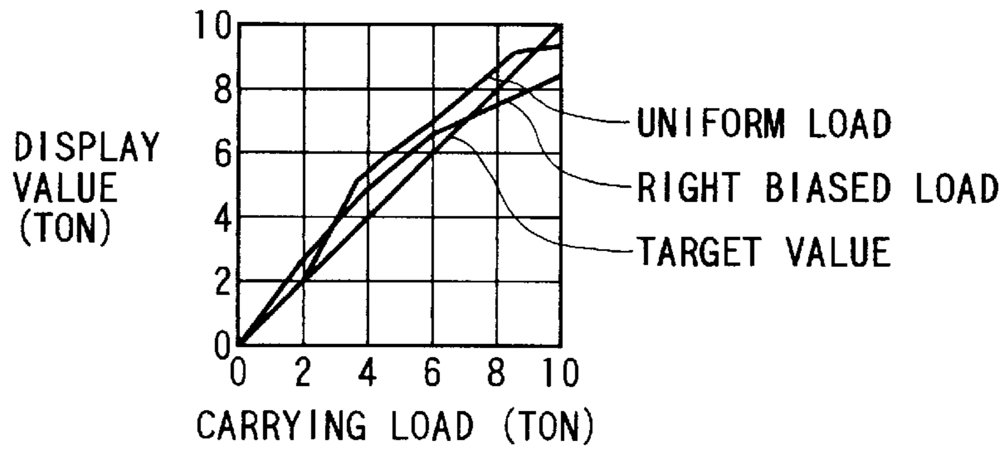
RELATION BETWEEN CARRYING LOAD AND DISPLAY VALUE
