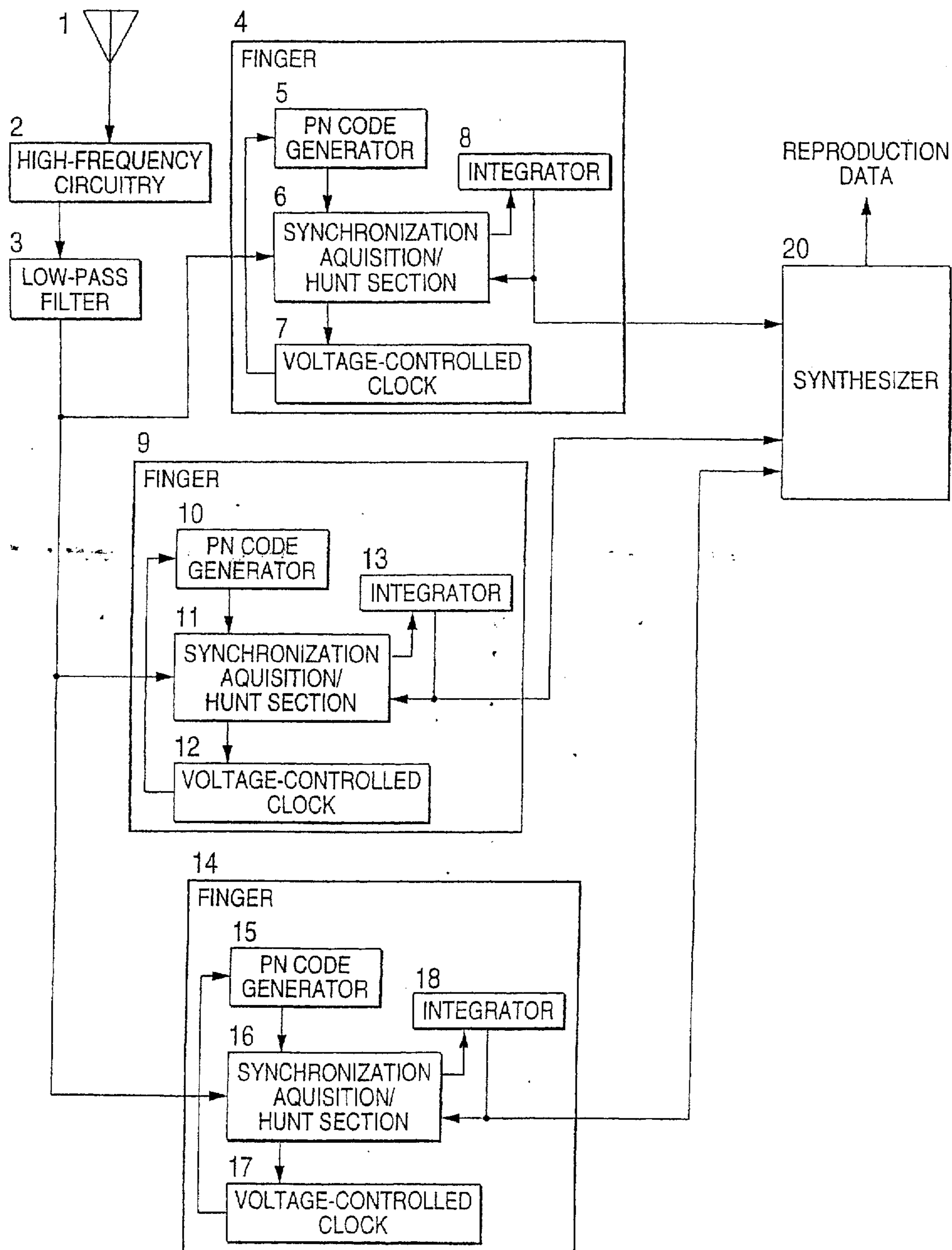
FIG. 6 PRIOR ART
