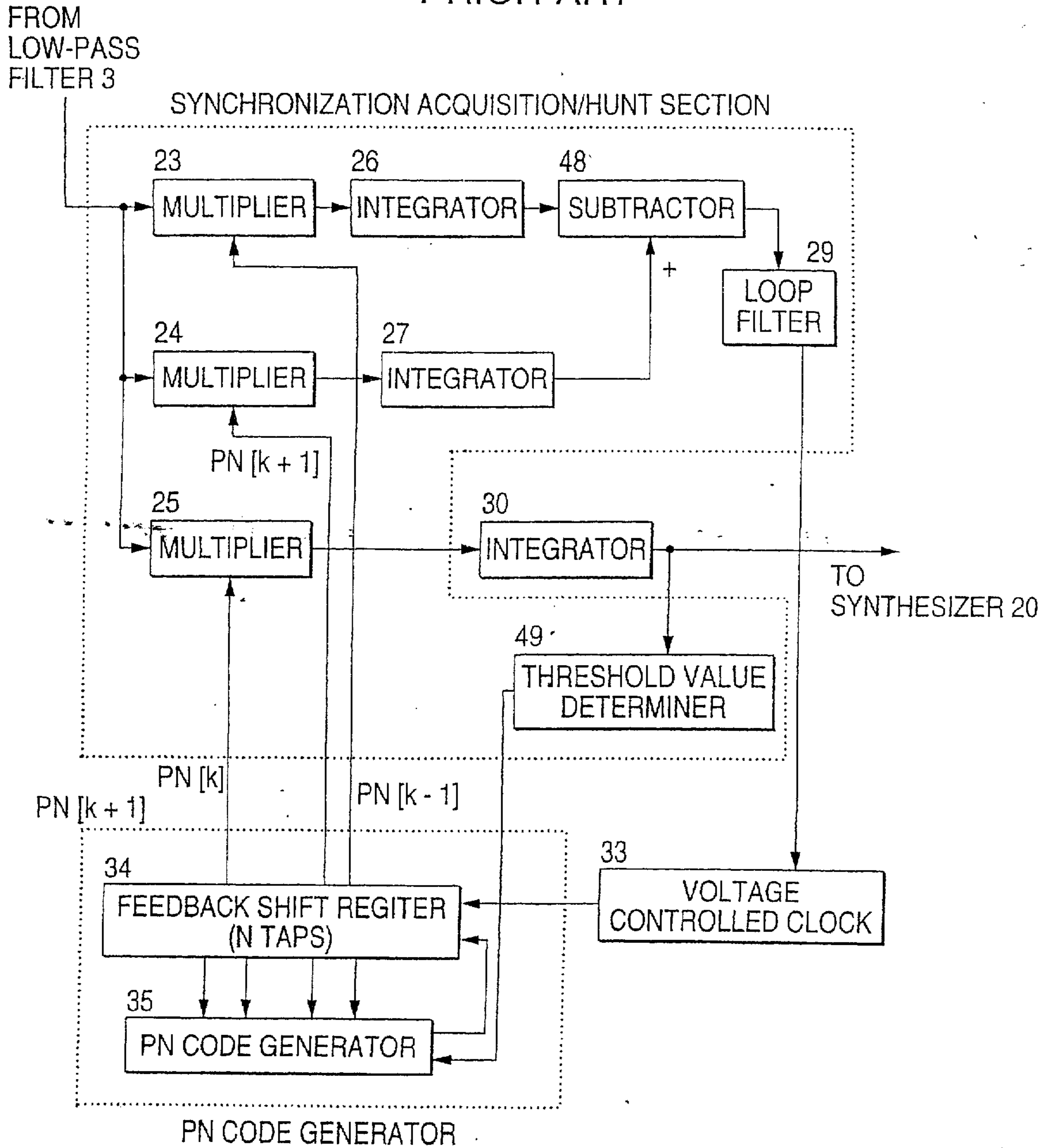
FIG. 7 PRIOR ART
