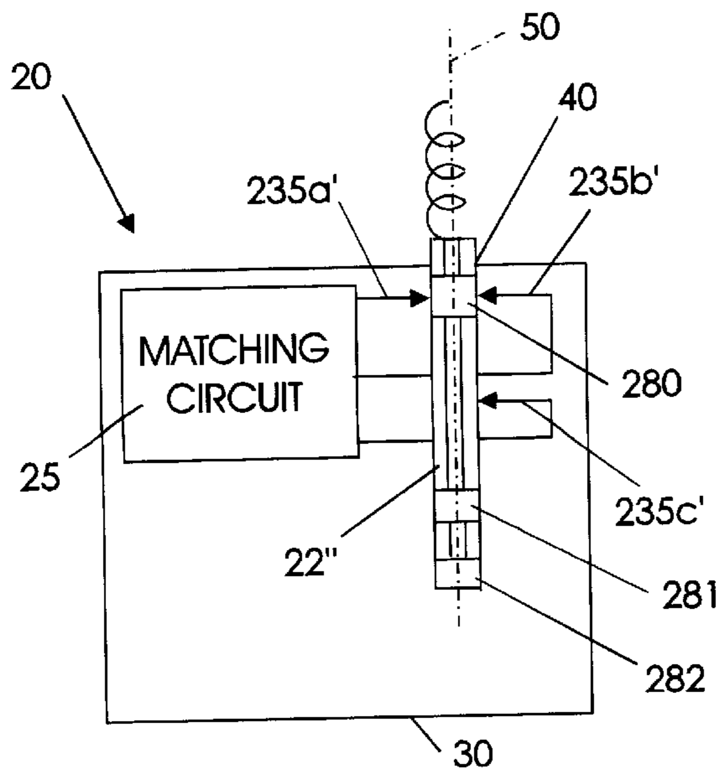
FIG. 11C RETRACTED
