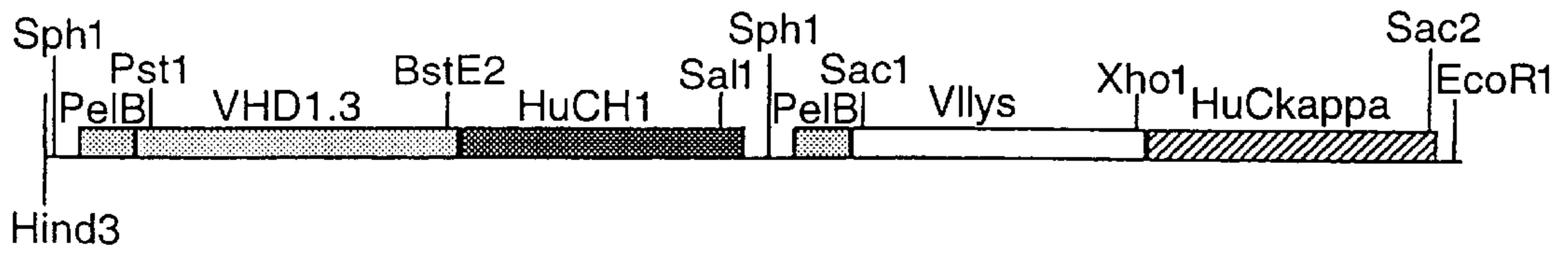
FabD1.3 in pUC19
