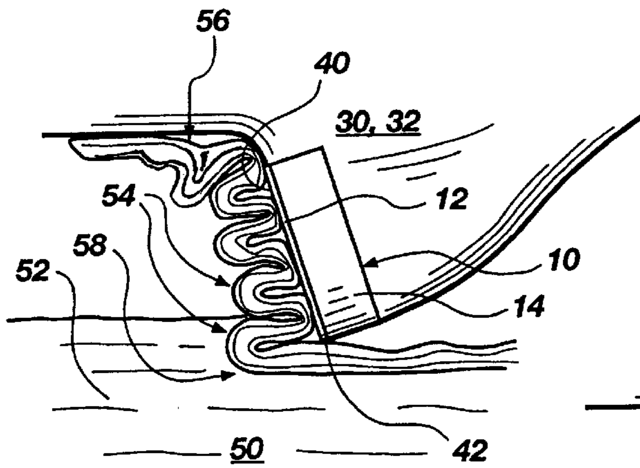
Fig. 3 (PRIOR ART)
