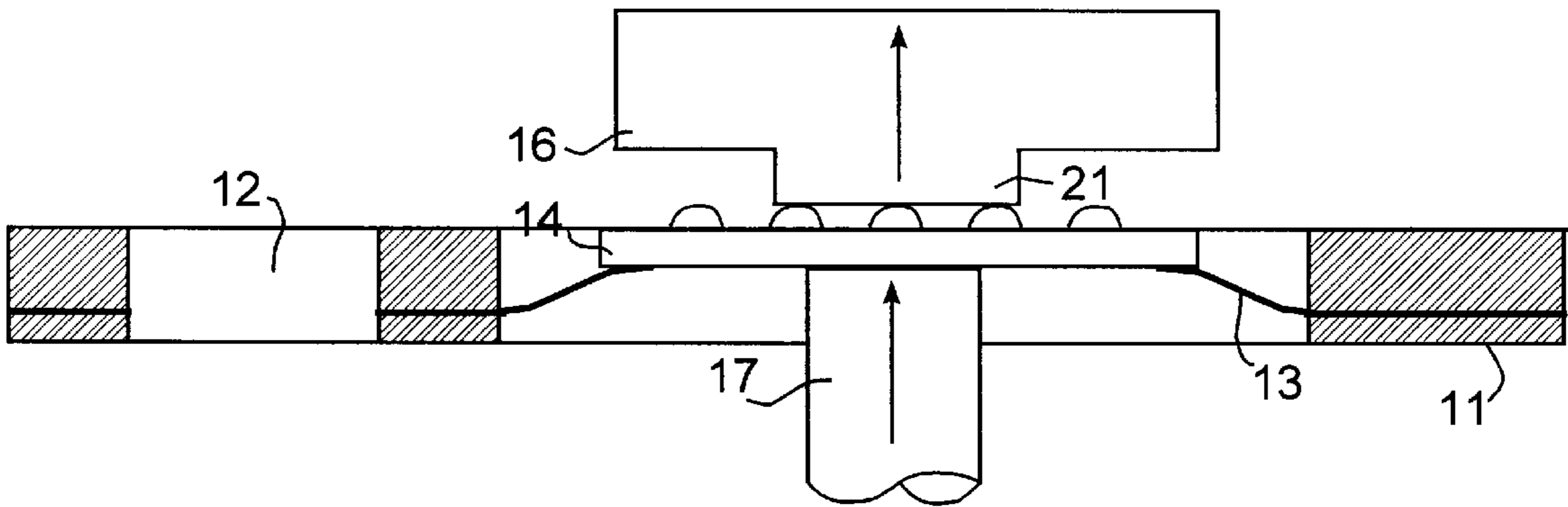
FIG. 3 (prior art)
