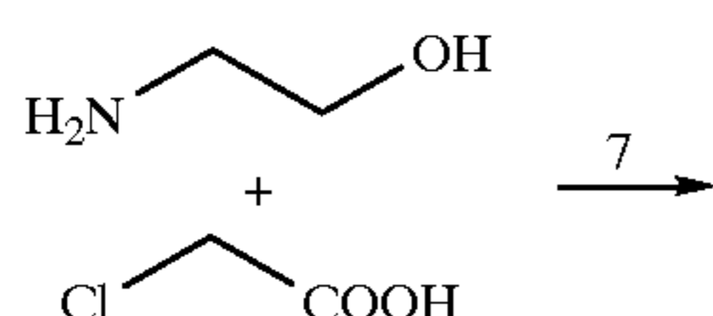
Example 4 Reaction Scheme
