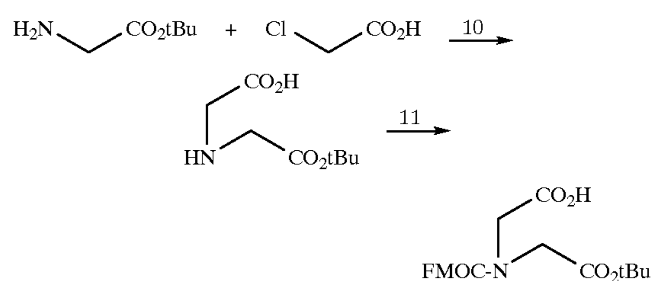
Example 5 Reaction Scheme
