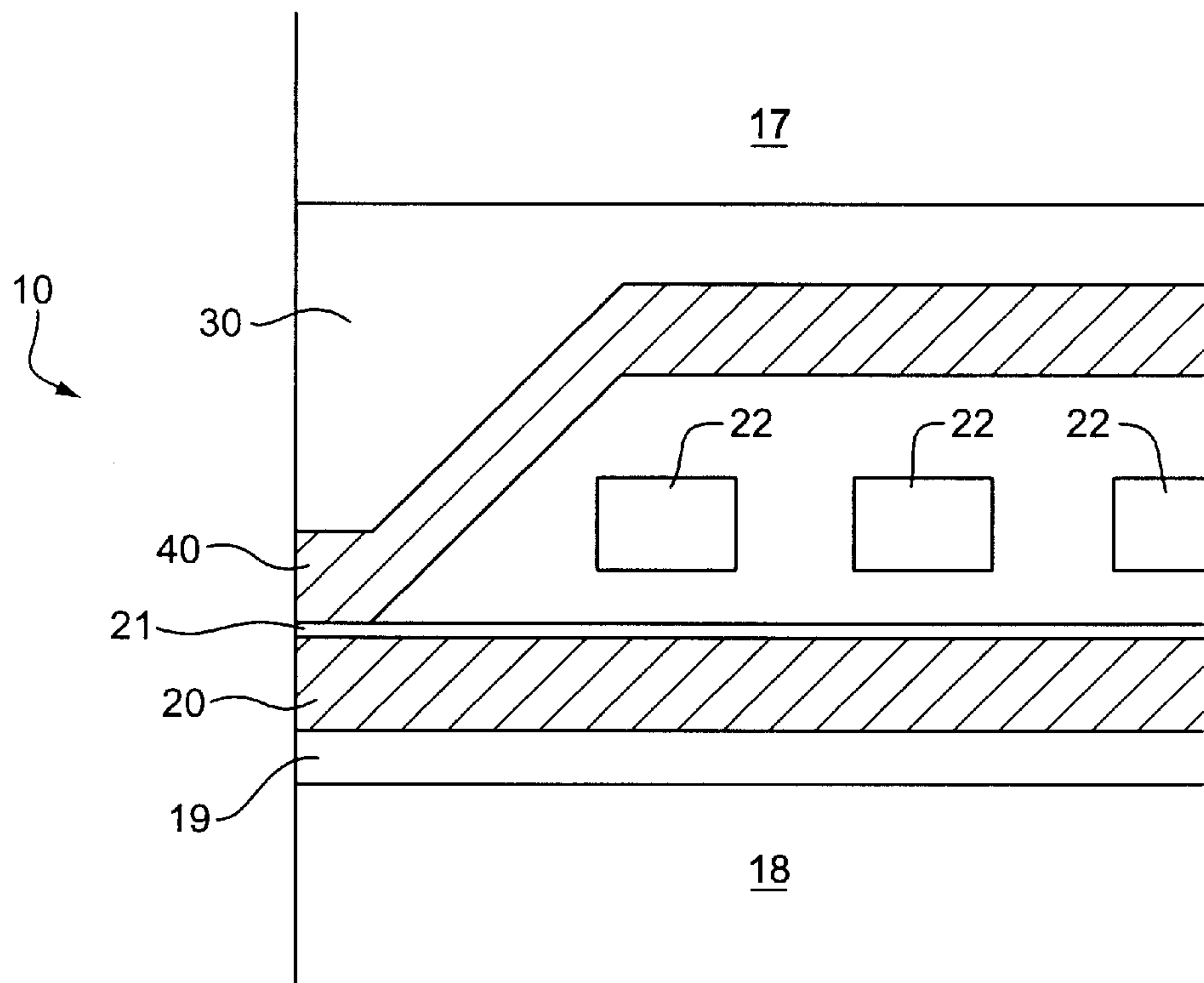
FIG. 3 PRIOR ART
