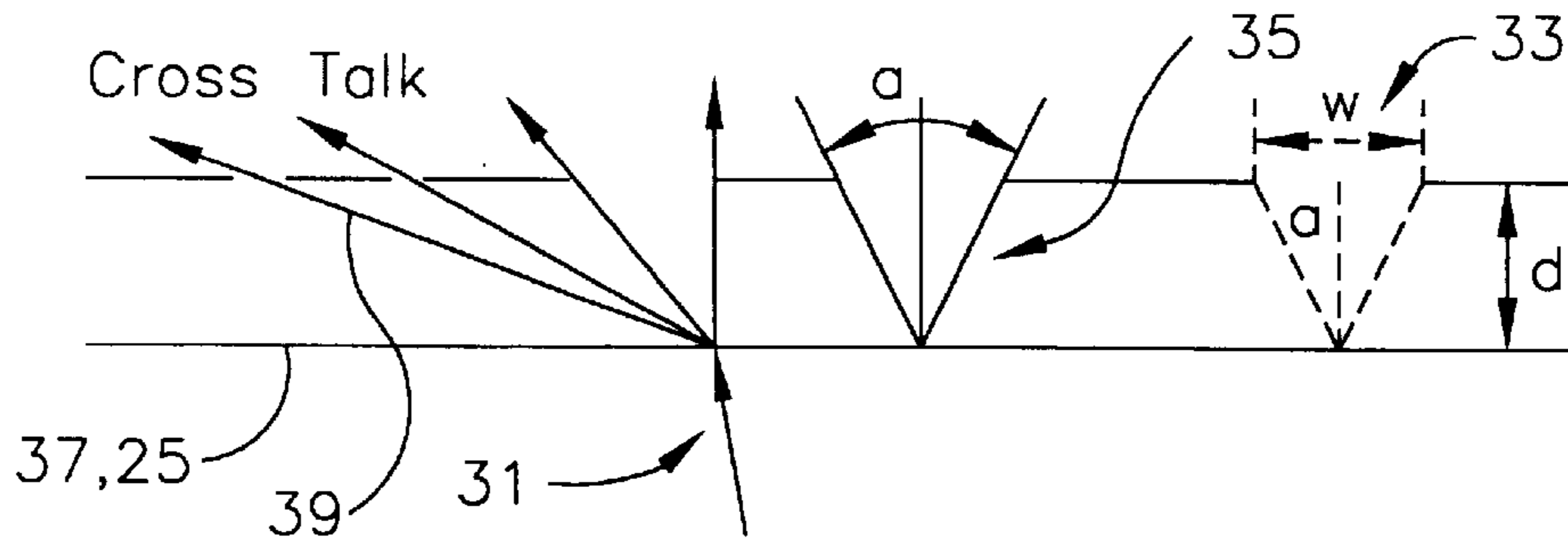
FIG. 2 (Prior Art)
