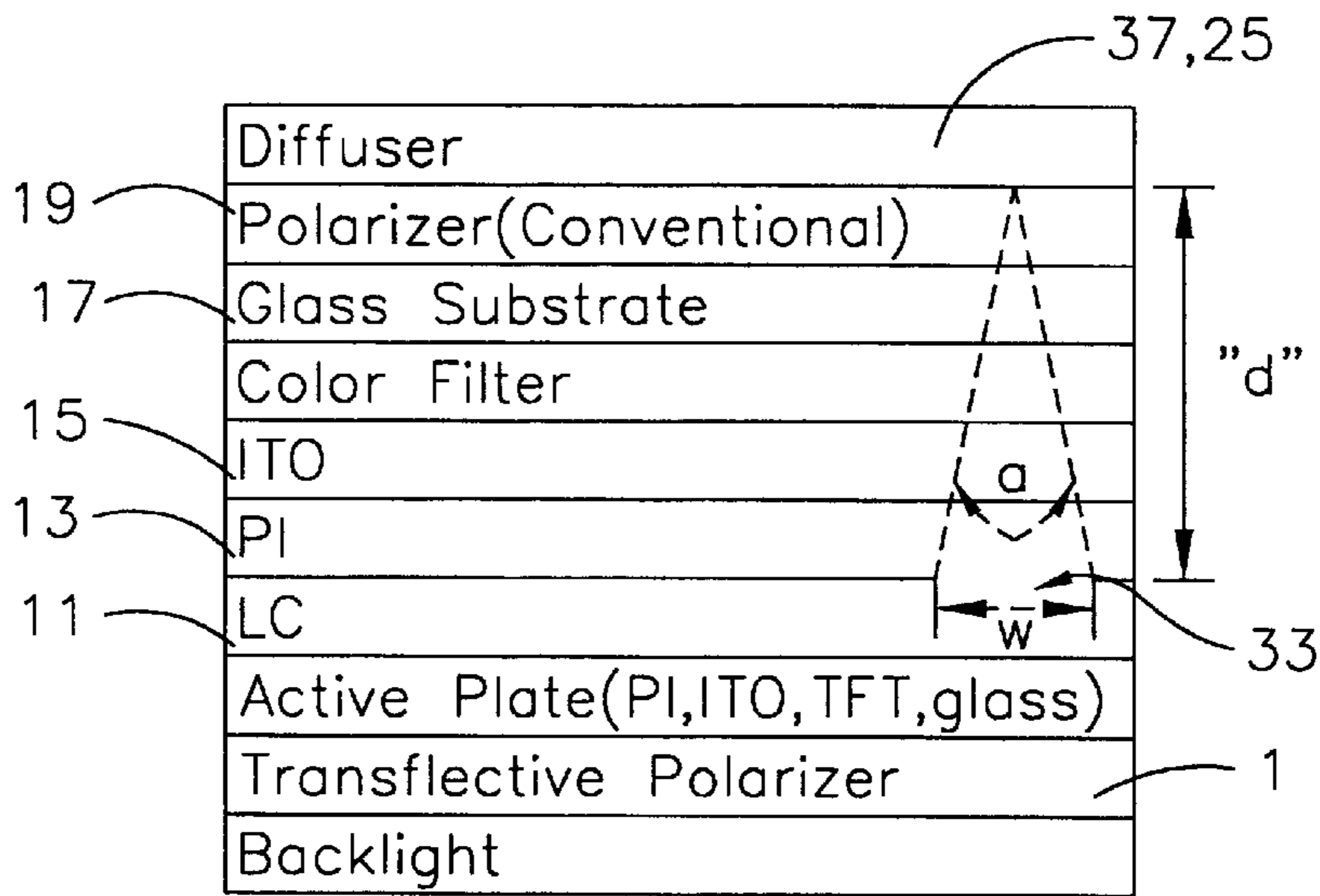
FIG. 3 (Prior Art)
