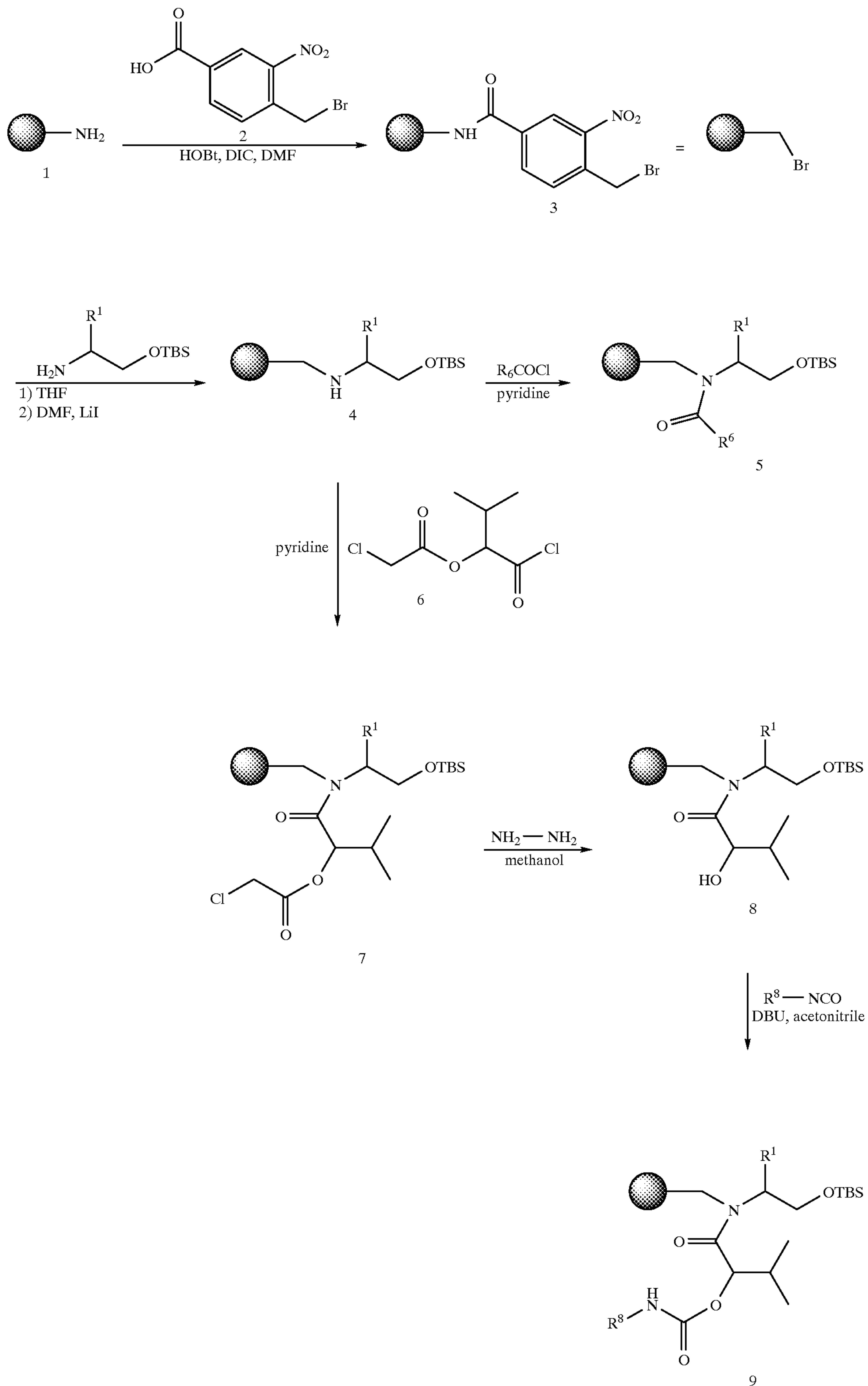
Scheme 1. Hydroxyphosphonate Synthesis
