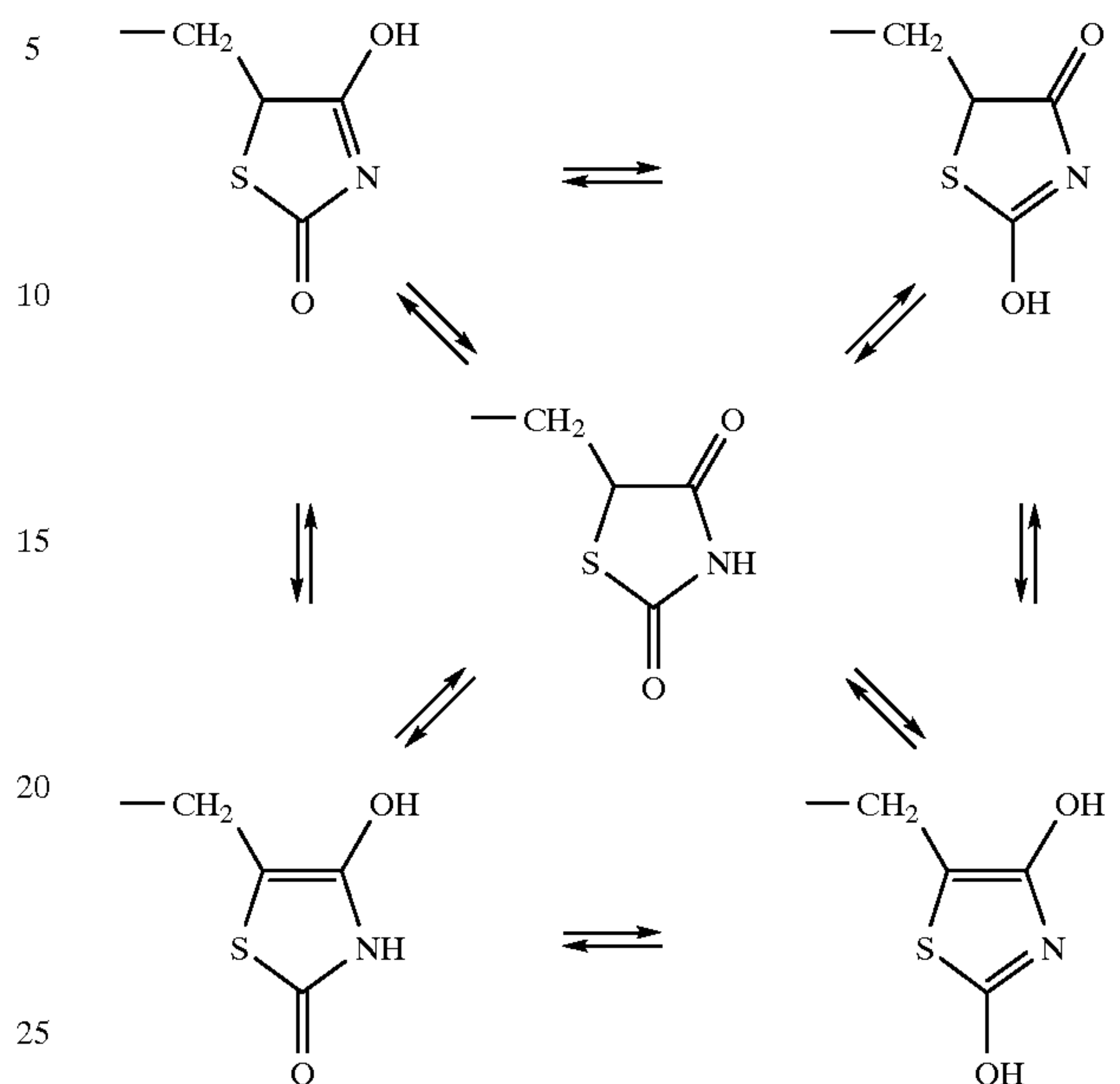
Scheme \alpha
