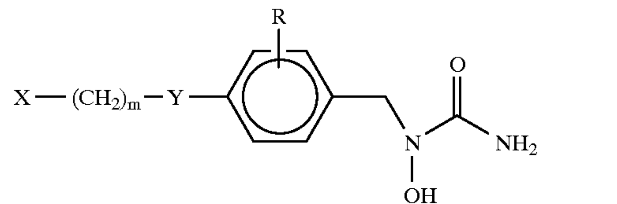
(I-5)
