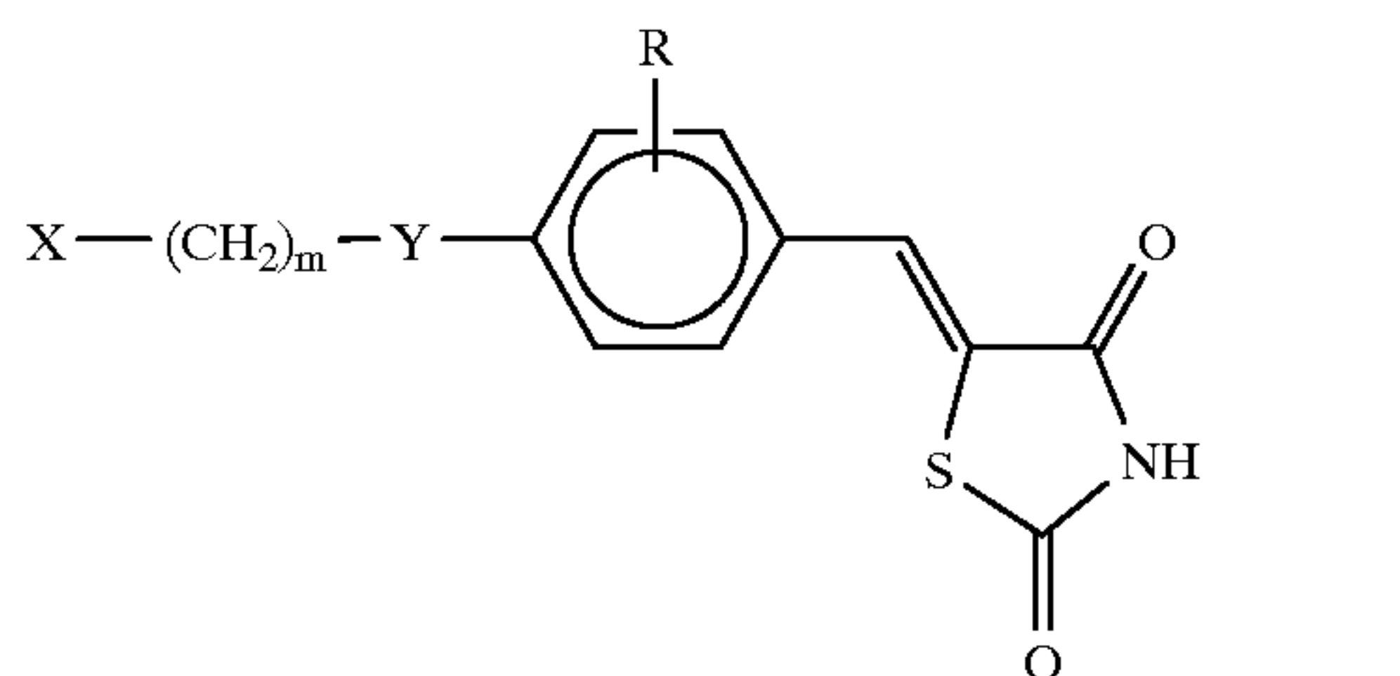
(I-2)
