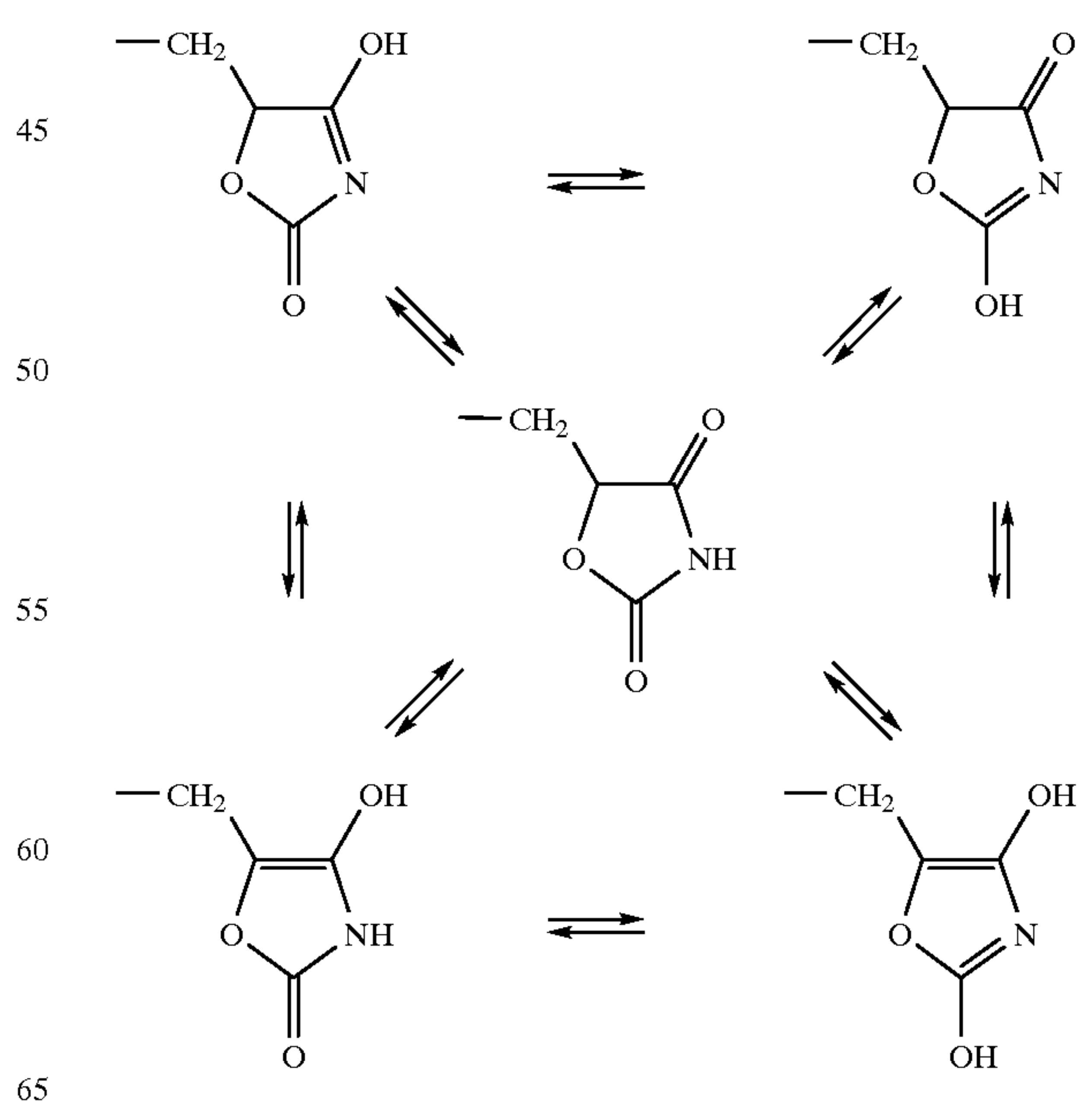
Scheme \gamma
