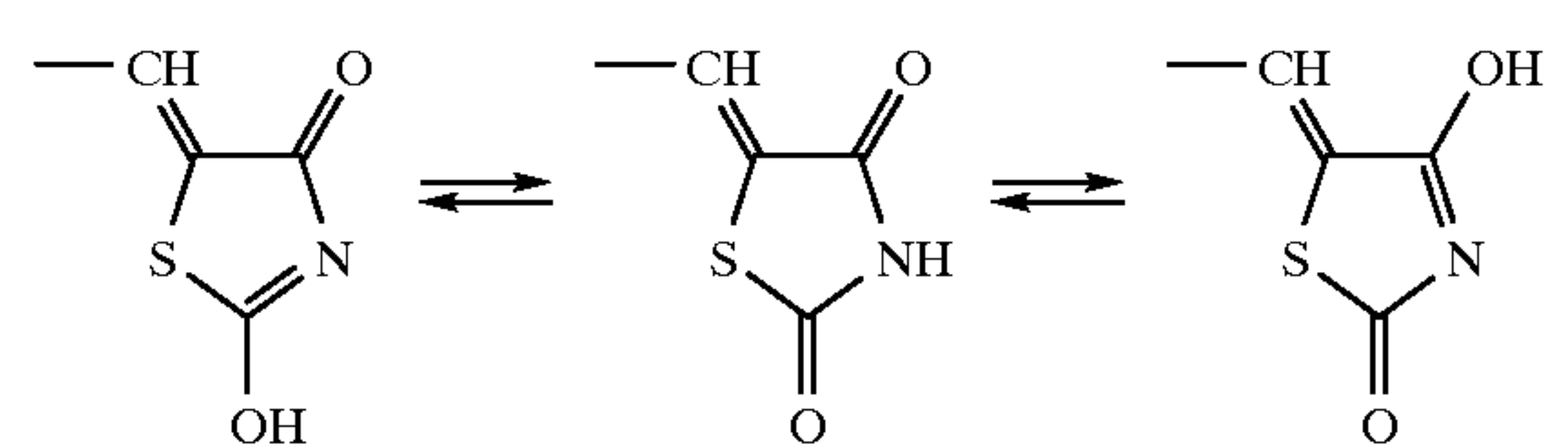
Scheme \beta
