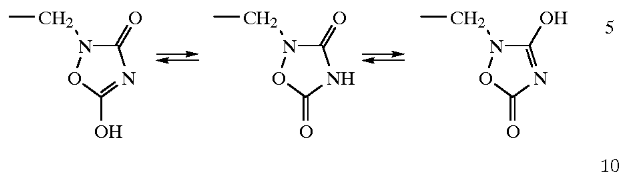
Scheme \delta
