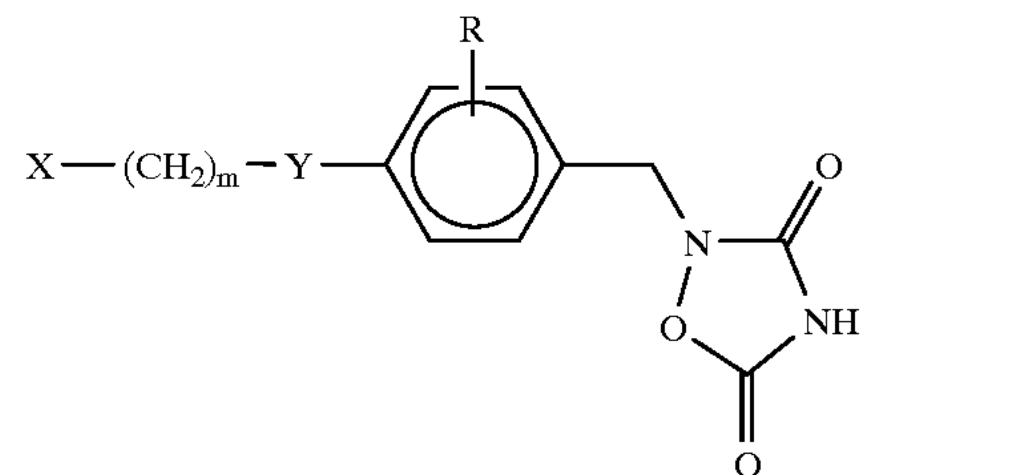
(I-5)
