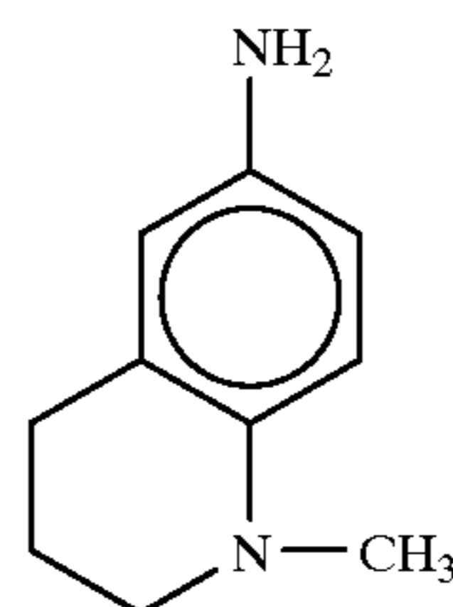
Compound (US-3) described in U.S. Pat. No. 2,196,739
