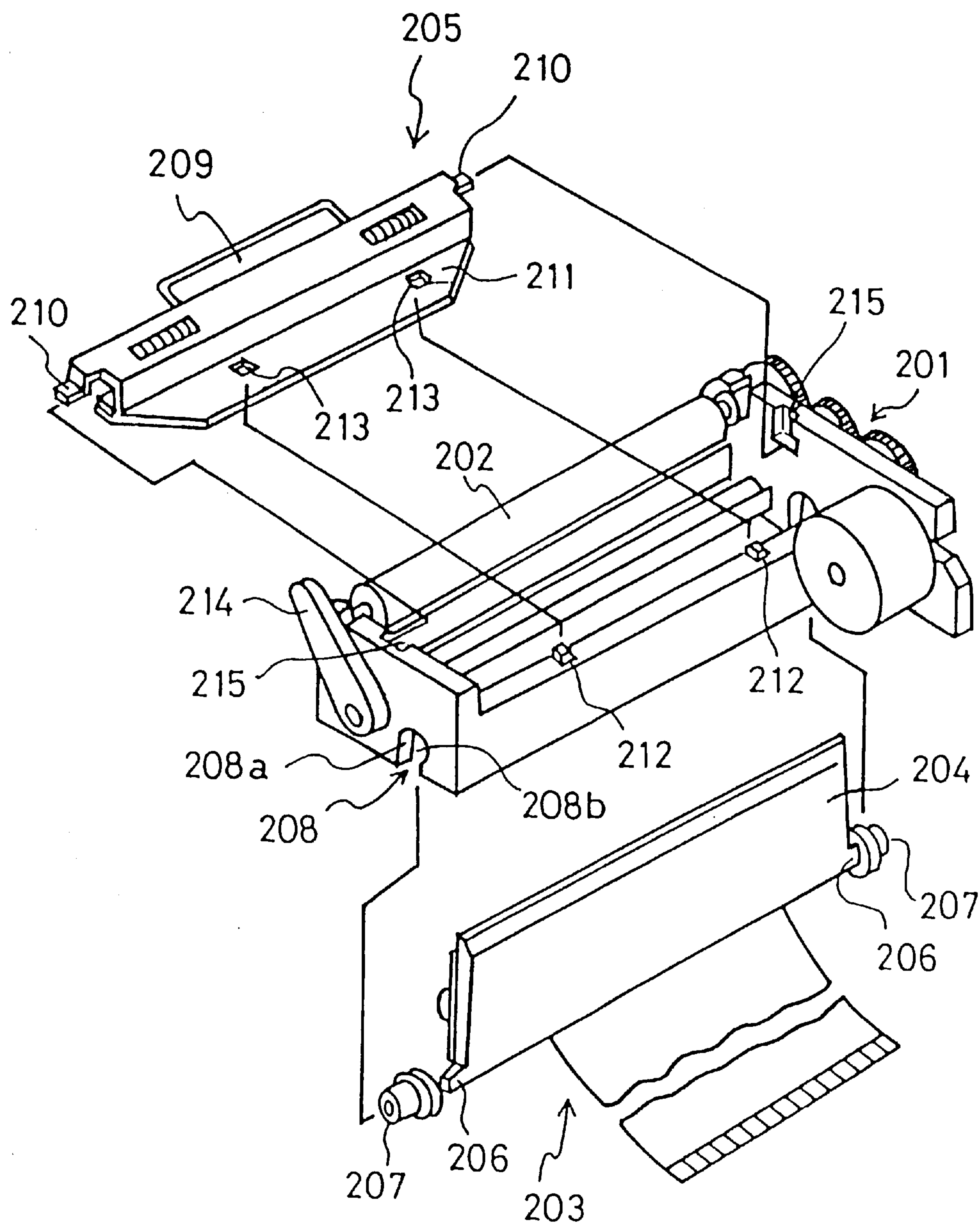
FIG. 4 PRIOR ART
