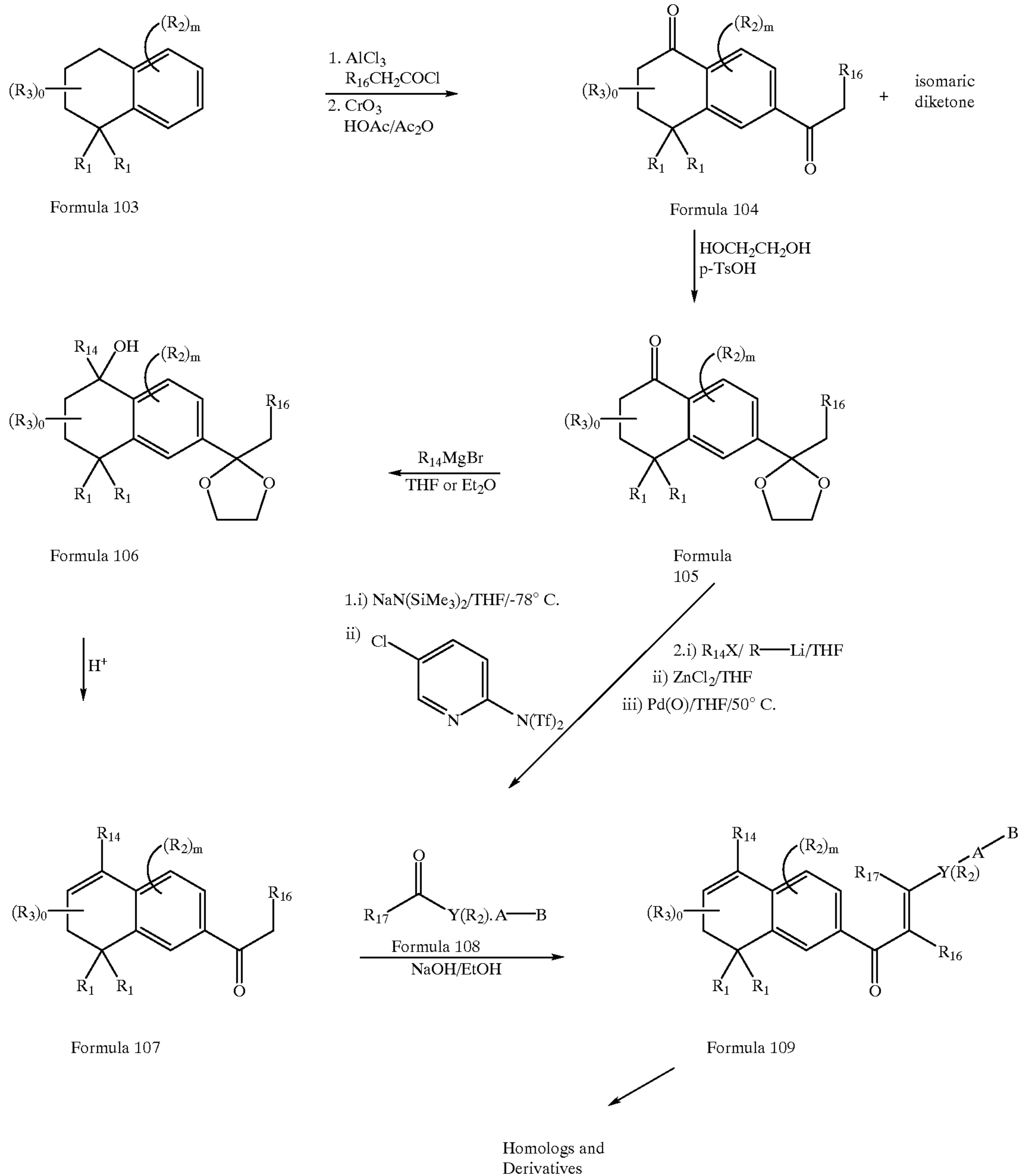
Reaction Scheme 101
