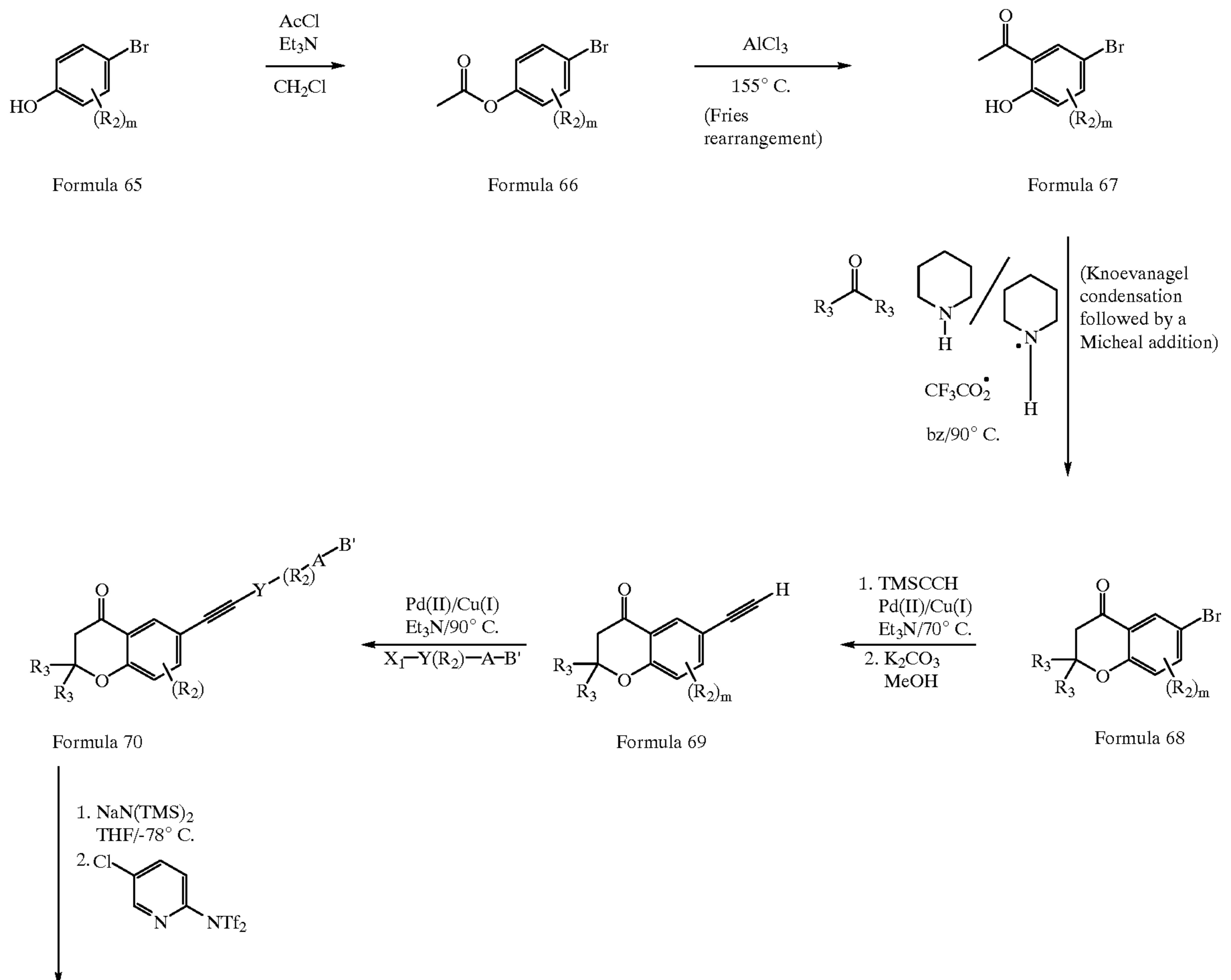
Reaction Scheme 10
