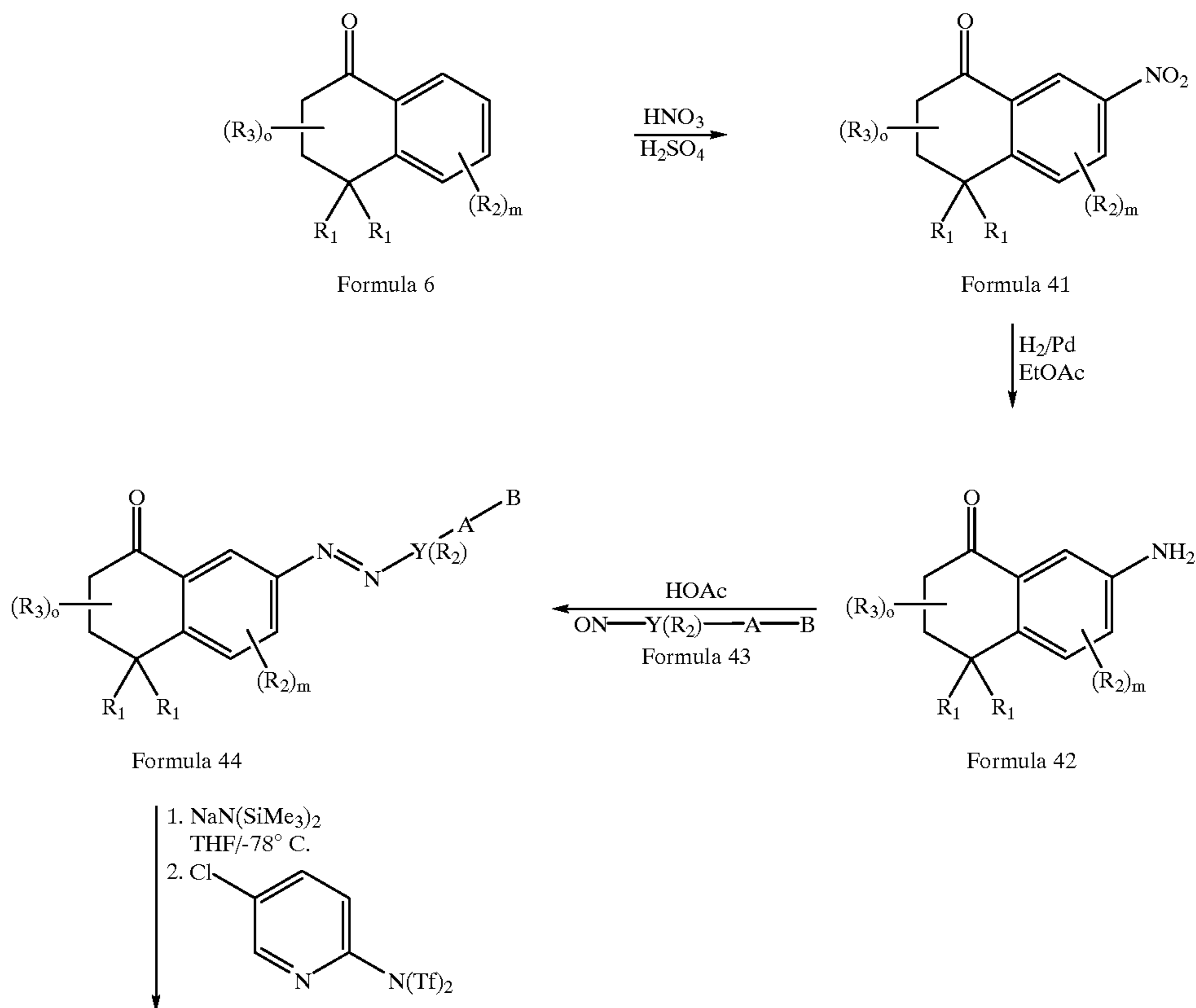
Reaction Scheme 5
