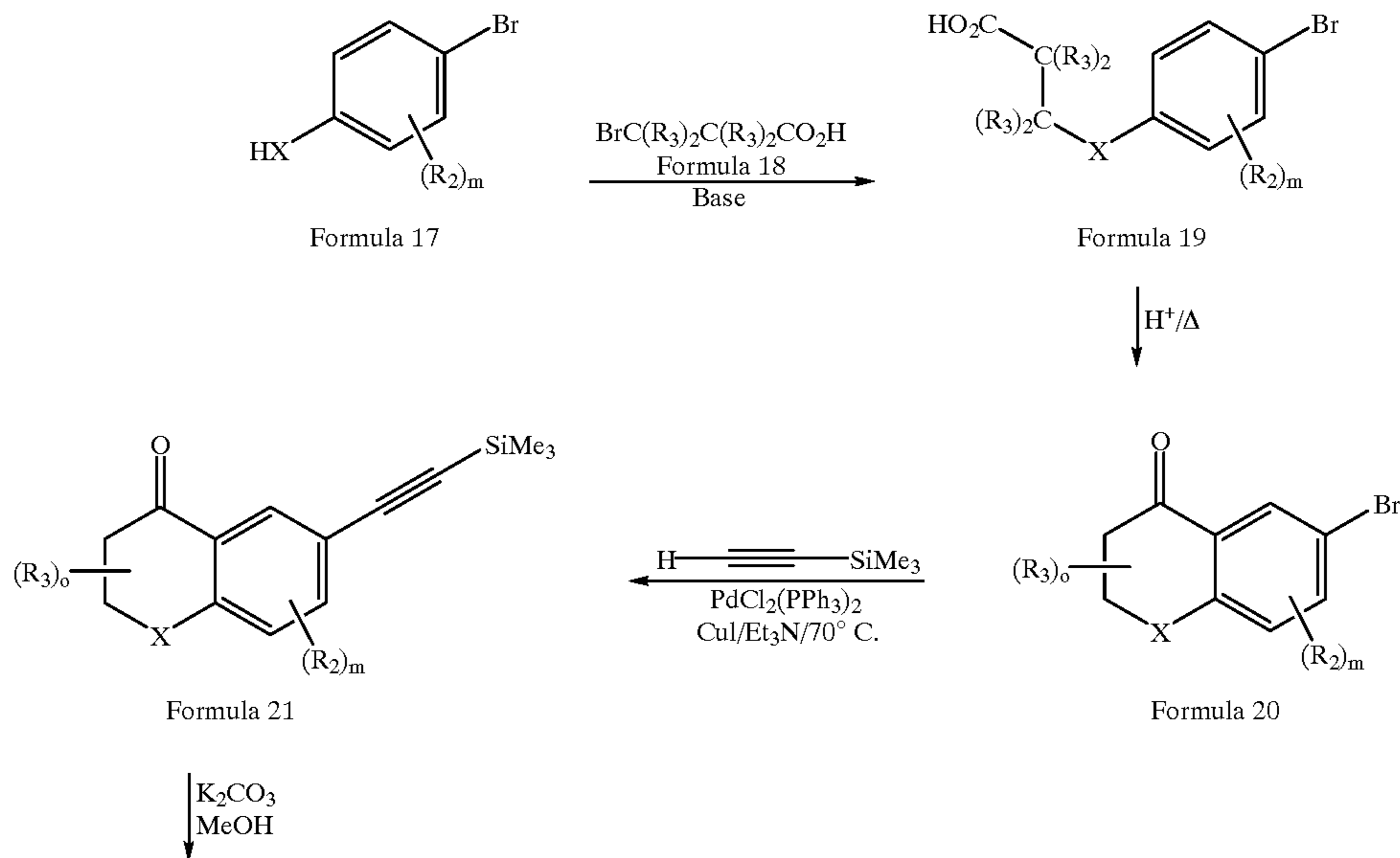
Reaction Scheme 2
