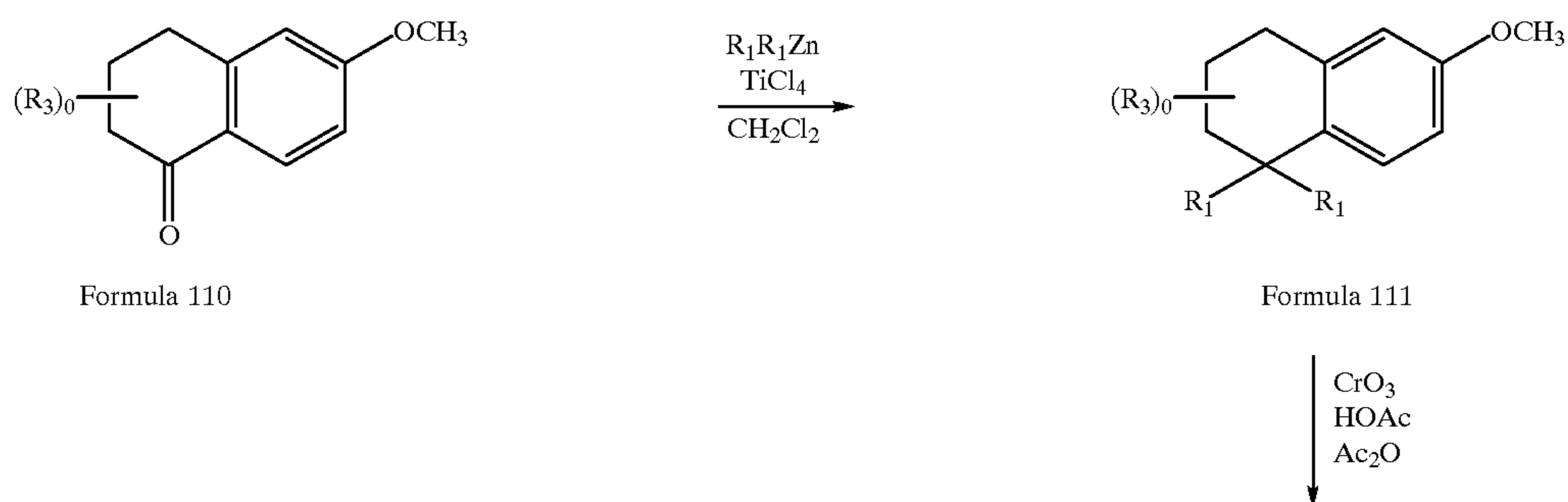
Reaction Scheme 102
