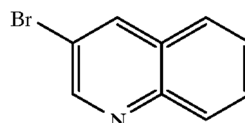
3-Bromoquinoline
