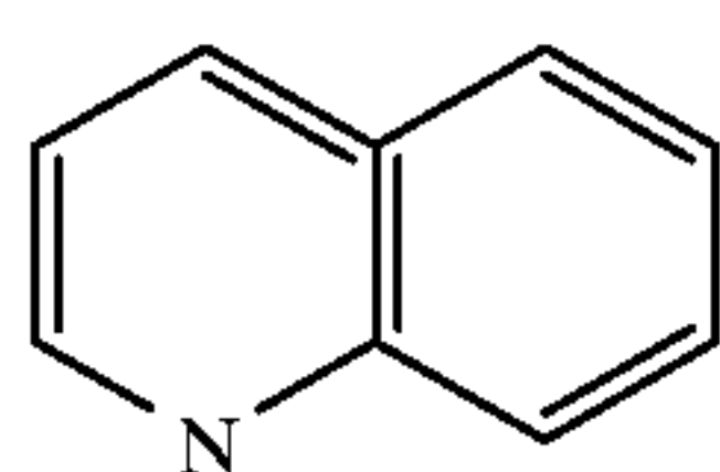
quinoline
