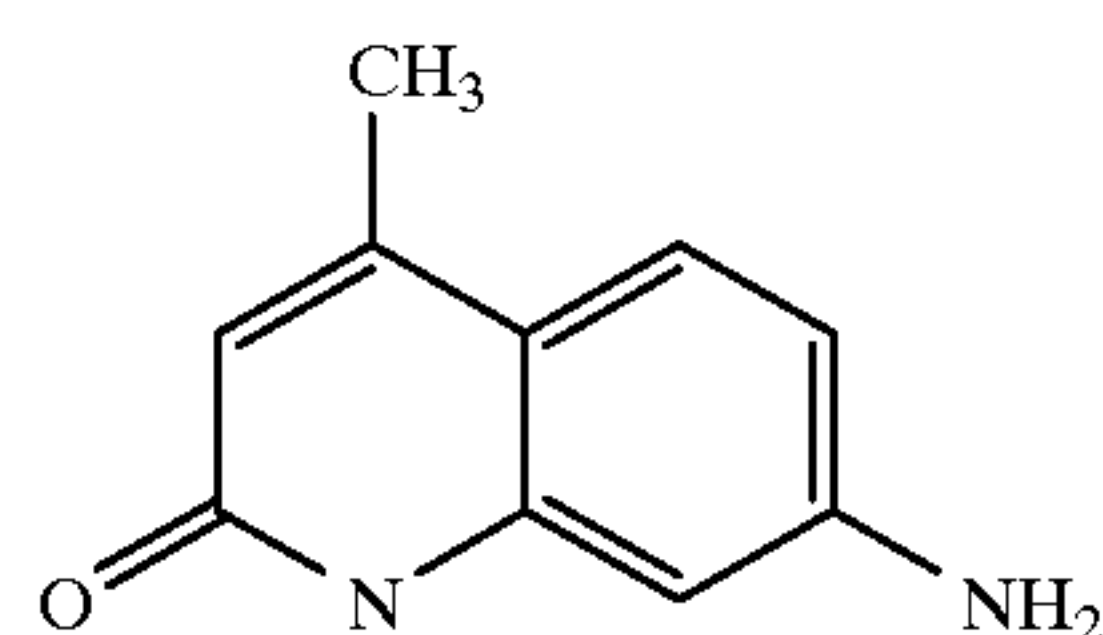
CARBOSTYRIL 124 (7-amino-4-methyl-2(1H)-quinolinone)
