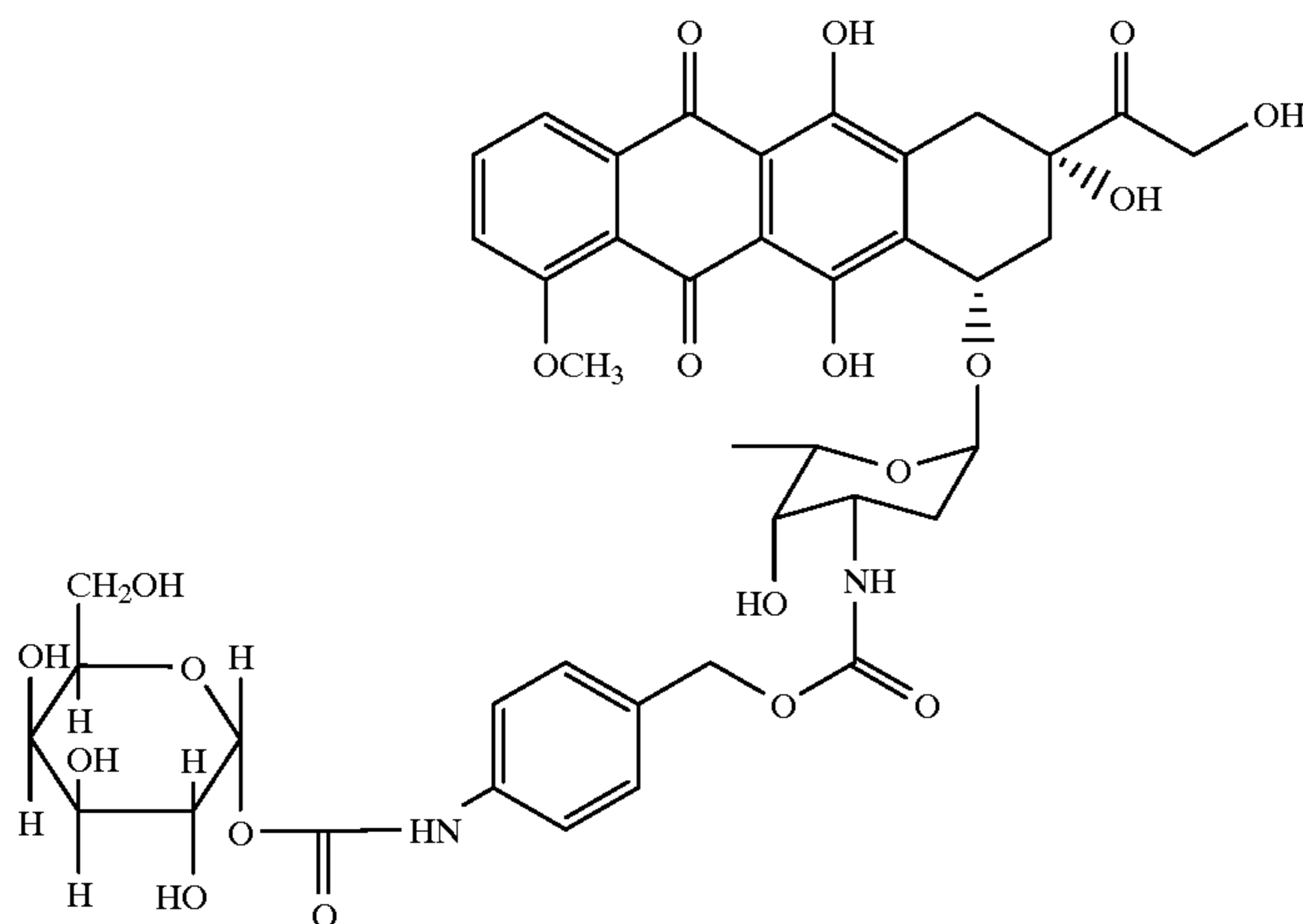
N-[4-(Alpha-D-galactopyranosyloxycarbonylamino)benzyloxycarbonyl]doxorubicin (compound 23)
